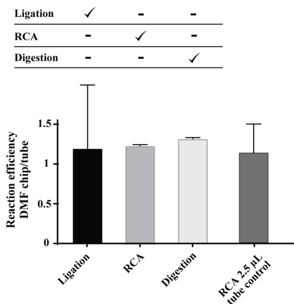
Figure 4: Enzymatic reaction efficiencies on the DMF chip. The C2CA enzymatic reaction steps were individually tested on-chip (The respective step that was performed on the DMF chip is indicated with “✓” in the table above the graph). Prior and subsequent steps were performed off-chip in reaction tubes (as indicated with “-” in the table above the graph). A RCA control with 2.5 \mu L reaction volume was performed in tubes testing for the effect of reaction volume reduction. After remaining steps were performed in tubes the C2CA products were counted. The reaction efficiencies are plotted as the ratio to the counted C2CA product number of a 20 \mu L tube control experiment. Error bars represent 1 stdev. from the mean (n=3 for ligation and RCA 2.5 \mu L, n=2 for RCA and Digestion; experiment repeated twice).
