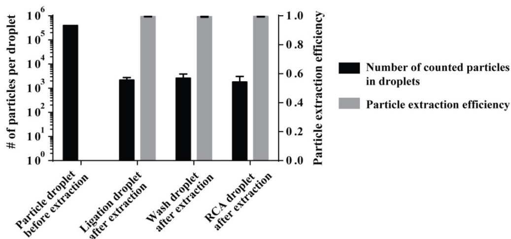
Figure 3: Magnetic particle extraction efficiency. Black bars indicate the average number of particles counted after extraction from the ligation, washing and RCA droplets and the number of particles per droplet before extraction (black bar on the left). Grey bars show the particle extraction efficiencies calculated as 1 - \text{number of particles in droplets after extraction} / \text{number of particles in droplets before extraction} ( n=4 each, error bars represent 1 stdev. from the mean).
