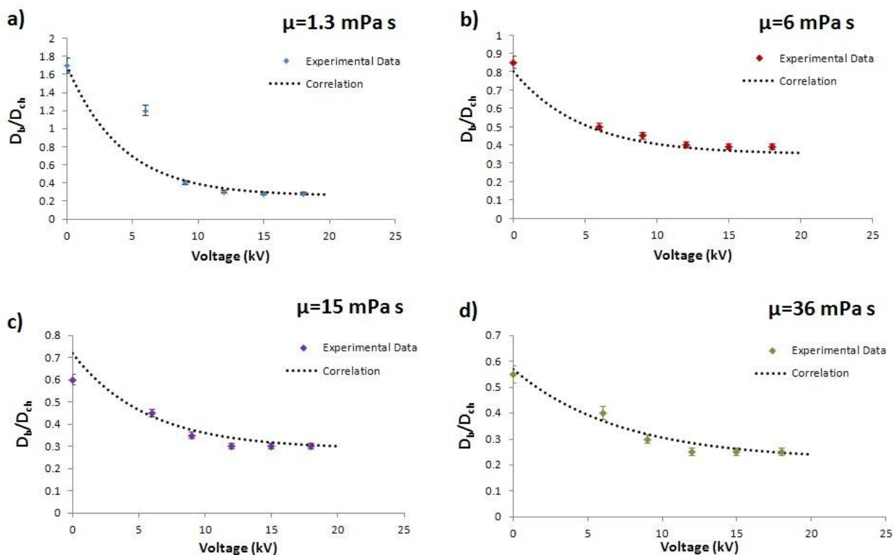
Fig. 7: Variation in bubble dimensionless diameter for solution with viscosity of a) 1.3, b) 6, c) 15 and d) 36 mPa s. (PDI < 1%).
