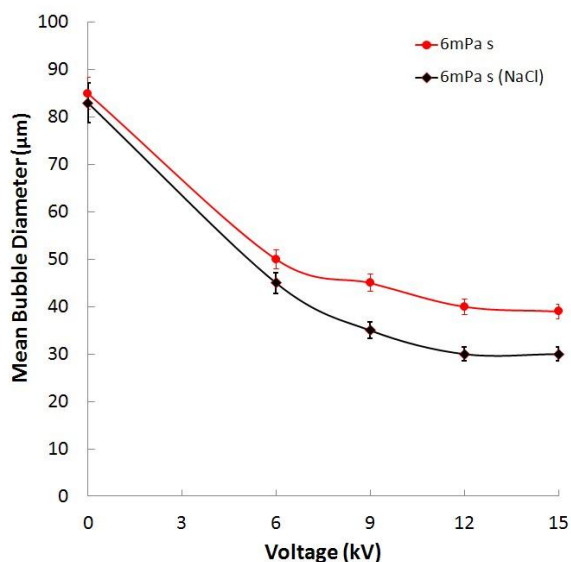
Fig. 6: Graph showing variation of mean bubble diameter with applied voltage for solution with constant viscosity of 6 mPa s with and without the addition of 1 wt.% NaCl solution (PDI < 1%).
