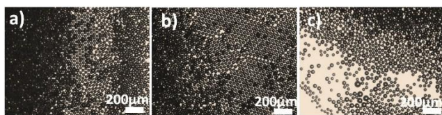
Fig. 4: Optical micrographs of microbubbles from a solution with 75% glycerol concentration at constant liquid flow rate of 0.01 ml/min at applied voltages of a) 12, b) 15 and c) 21 kV.
