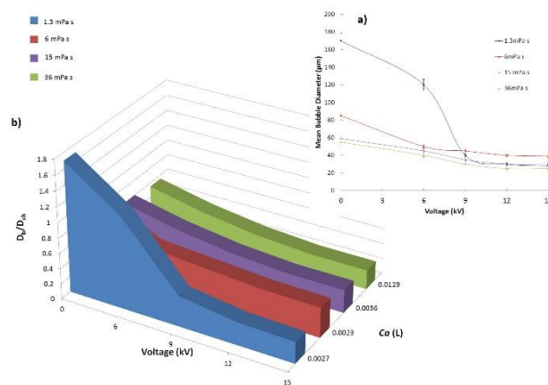
Fig. 5: a) Graph showing variation of bubble diameter with applied voltage for solution viscosities of 1.3, 6, 15 and 36 mPa s, and b) 3D plot of dimensionless bubble diameter with respect to voltage and capillary number increment.
