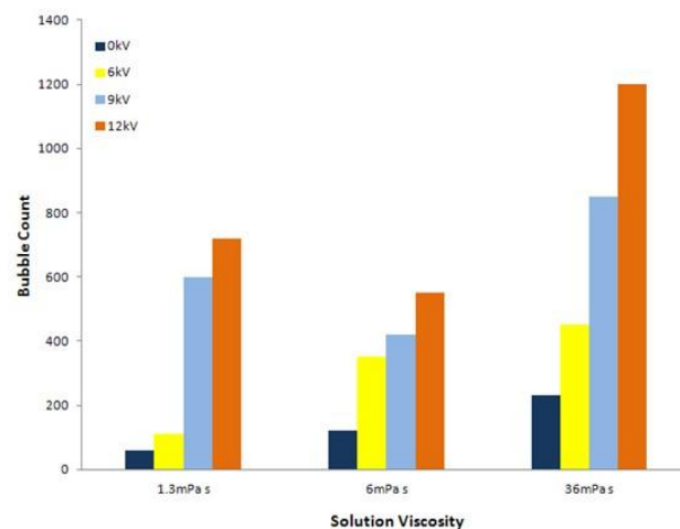
Fig. 9: Graph showing variation in the number of bubbles generated with applied voltage for three different solution viscosities of 1.3, 6 and 36 mPa s over a fixed time period of 5 seconds and collection area of 1.5 mm 2 .
