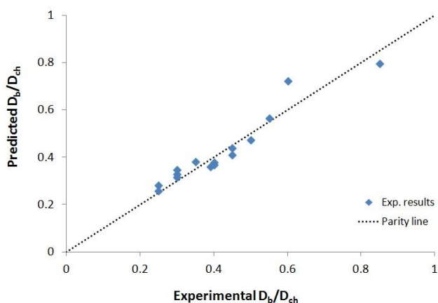
Fig. 8: Graph representing experimental data for dimensionless bubble diameter against predicted values.
