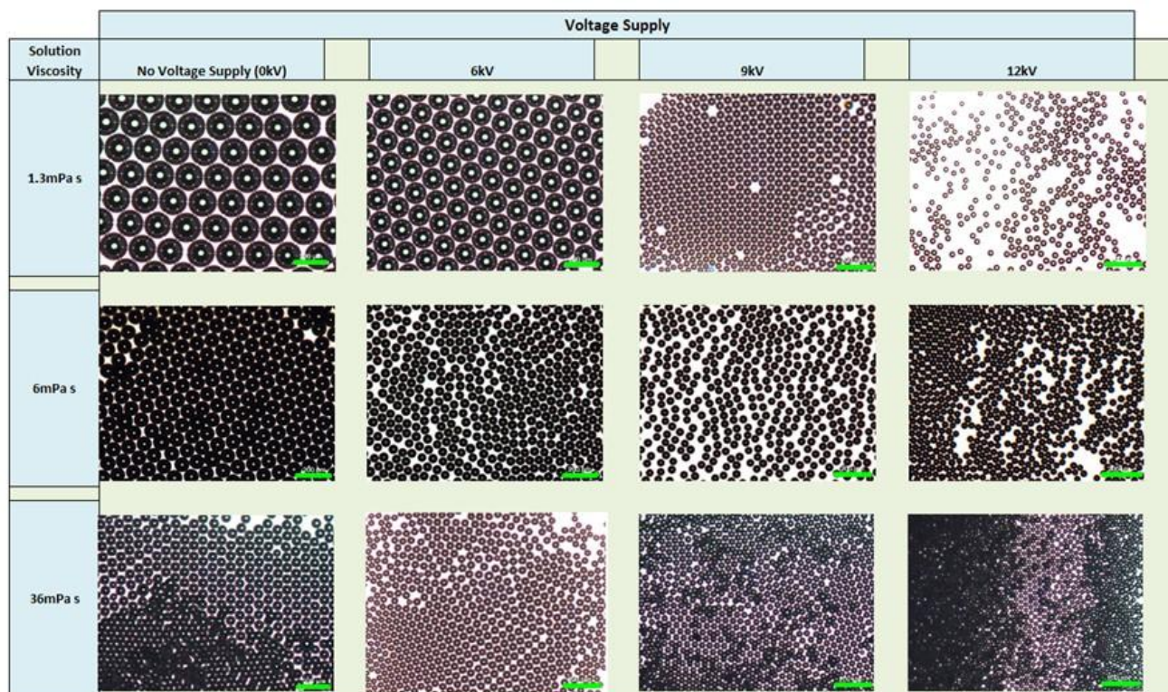
Fig. 3: Optical micrographs of bubbles formed in aqueous glycerol with 5, 50 and 75 % concentration at applied voltages of 0, 6,9 to 12 kV and a constant liquid flow rate of 0.01ml/min. Scale bar is 200 \mu\text{m} .
