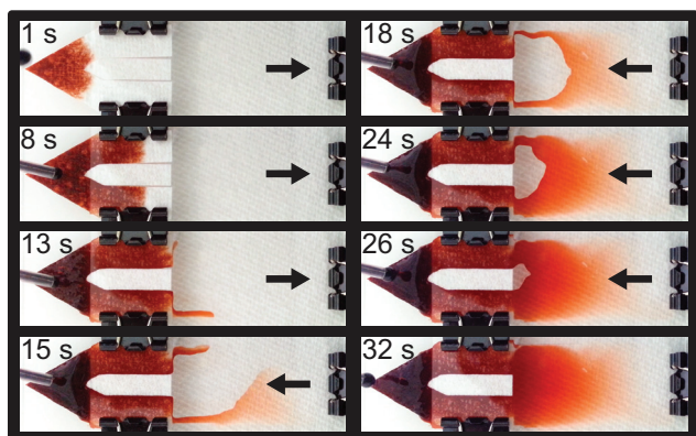
Figure 2 – Time series showing filling of an automated blood staining cartridge, demonstrating use of a snorkel to remove a trapped air bubble from the device. The hydrophilic paper is not dyed in this image sequence to enable easier visualization. Liquid fills the side walls of the cartridge first, then travels back towards the paper wick until an air bubble is encased. Normally, this air bubble would be trapped, but a snorkel allows its escape and replacement with additional liquid. Also evident in this image sequence is the slanted nature of the microscopy chamber, which generates both thick and thin regions. An example of a manually prepared thick and thin smear, prepared by an expert microscopist is shown in Figure S1.
