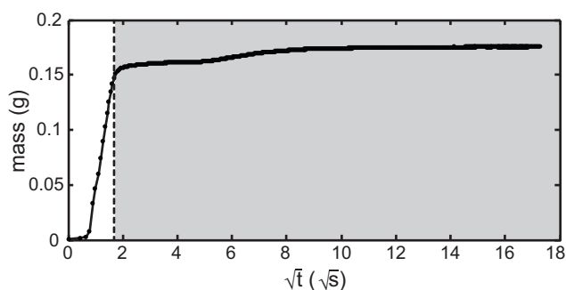
Figure 5 – Mass as a function of time during the filling of a cartridge with DI water, which was measured to determine blood volume in the transparent region and to compare that with the volume of blood used in traditional smear preparation techniques. The area to the right of the dotted line indicates the volume outside the paper (the transparent region). Though pore size in the paper was not determined, the fluid behavior inside the paper shows general agreement with the Washburn equation, which is sufficient for differentiating between the paper and non-paper transparent regions. The mass at the far right data point is 0.1755 g, and the mass at the dotted line is 0.1534 g, indicating a transparent region volume of 22.1 microliters. This experiment was repeated 10 times, with a mean volume of 21.3 +/- 2.1 \mu\text{L} .
