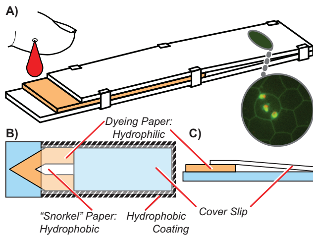
Figure 1 – A) A 3D view of cartridge showing blood being dispensed from the left, acridine orange dye filled paper where staining occurs, and the unobstructed, transparent coverslip region where imaging is conducted via microscopy. B) A top-down view of the cartridge showing the dye-filled paper, the snorkel paper, and a hydrophobic ring around the outside of the cartridge. The snorkel allows air bubbles to leave during filling (see Figure 2). As in dead-end filling, 9 the hydrophobic ring prevents blood from leaving the cartridge during and after filling, without requiring a bonding step. C) A cross-section of the cartridge, emphasizing the slanted nature of the coverslip during use, which permits imaging in both thick (many cells) and thin (single cell) regions.
