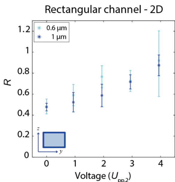
Figure 5. Two-dimensional focusing in the rectangular channel. The relative focusability R plotted against the voltage U_{pp,2} on the second (5-MHz) piezo transducer focusing the particles vertically in the rectangular channel. The voltage U_{pp} on the first (2-MHz) transducer and the flow rate were kept constant at the same value as used to focus the particles giving the data points surrounded by the dashed red rings in figure 4 for the 1- \mu\text{m} ( 10 \mu\text{L min}^{-1} ) and 0.6- \mu\text{m} -particles ( 3 \mu\text{L min}^{-1} ), respectively.
