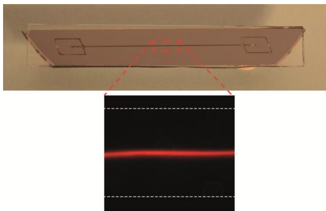
Figure 6. Fluorescent image of 0.5- \mu\text{m} particles (red) focusing in the square-cross-section channel at a flow rate of 2 \mu\text{L min}^{-1} and at the same voltage as used for the 0.6- \mu\text{m} particles in the square-cross-section channel focusing experiments. The broken gray lines show the edges of the channel.
