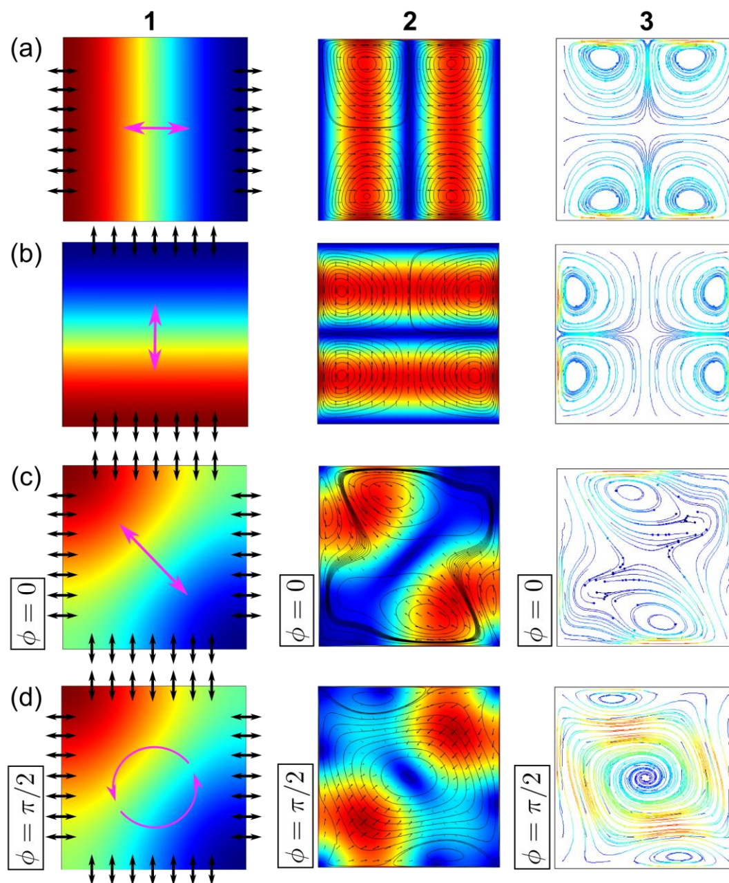
Figure 2. Acoustophoretic motion of 0.5- \mu\text{m} -diameter particles in the nearly-square microchannel cross section. The rows (a-d) corresponds to the four cases shown in Figure 1. The actuation frequency was f_1 in (a), f_2 in (b), and f_m in (c-d). For each case, column 1 is a snapshot in time of the amplitude of the oscillating first-order acoustic pressure (color plot where red is positive, green is zero, and blue is negative). Column 2 is the acoustic radiation force (color plot and arrows where red is positive and blue is zero) together with streamlines (black contour lines) of the steady streaming velocity field. Column 3 is the acoustophoretic trajectories (colors indicate the speed where red is positive and blue is zero) of 0.5- \mu\text{m} -diameter particles released from a regular grid in the channel cross section. To best illustrate the qualitative results, the color scale is set by the maximum value in each plot individually. For the color plots 1(a-c) the magenta arrow indicates that the pressure has an almost static nodal line (green) while the amplitude oscillates. For the color plot 1(d) the magenta arrows indicate that the nodal line (green) of the pressure field rotates in time.
