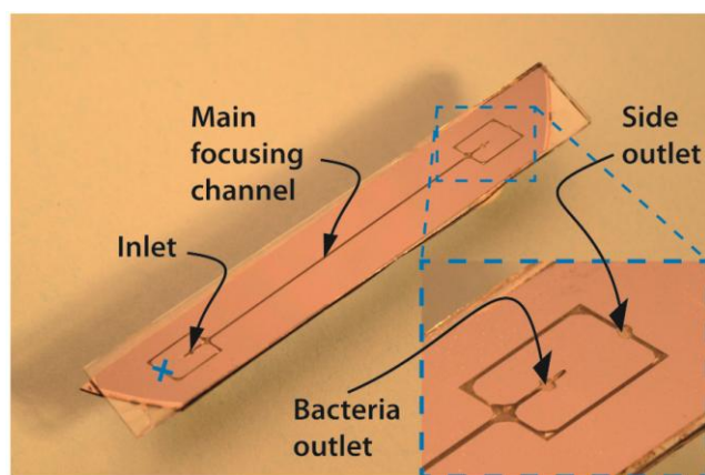
Figure 3. Photograph of the chip design. The main focusing channel is 35 mm long and 230 \mu\text{m} wide, while its height is either 230 \mu\text{m} (square channel) or 150 \mu\text{m} (flat rectangular channel). After the trifurcation, the side channels are connected to one outlet. The inlet marked with a blue cross is not used.
