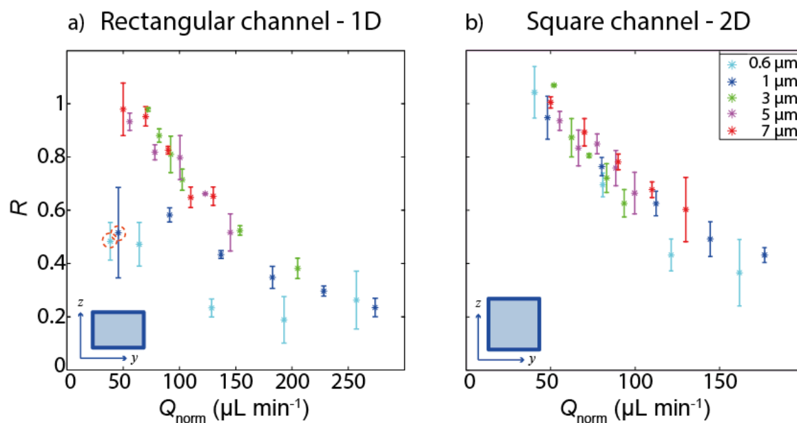
Figure 4. (a) One-dimensional focusing in the rectangular channel. The relative focusability R plotted against the normalized flow rate Q_{\text{norm}} . (b) Two-dimensional focusing in the square channel. The relative focusability R plotted against Q_{\text{norm}} . All error bars are standard deviations from three repeated measurements. The nominal flow rates for each data point are collected in table 1.
