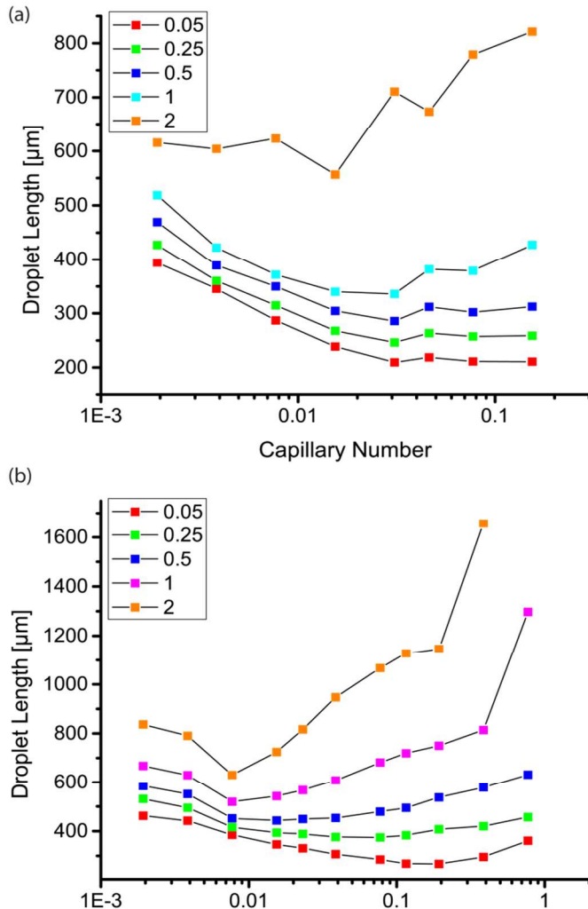
Fig. 3 Plot of droplet length as a function of capillary number for different flow rate ratios as indicated in the legends in channels with inlet and main channel widths of (a) 50 and 200 μm and (b) 100 and 400 μm.
