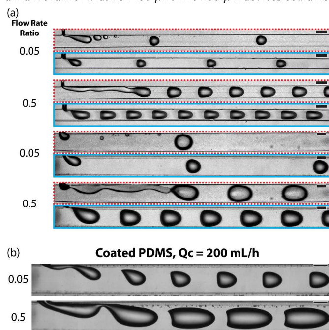
Fig. 2 (a) Micrographs contrast the droplet formation process in uncoated (red/dashed outline) and fluoropolymer coated (cyan/solid outline) channels. The continuous phase flow rate was 10 mL/h and the channel widths were 200 or 400 μm. (b) Droplet formation was imaged at a continuous phase flow rate ( Q_c ) of 200 mL/h in coated channels with a width of 400 μm. Scale bars indicate 200 μm.
