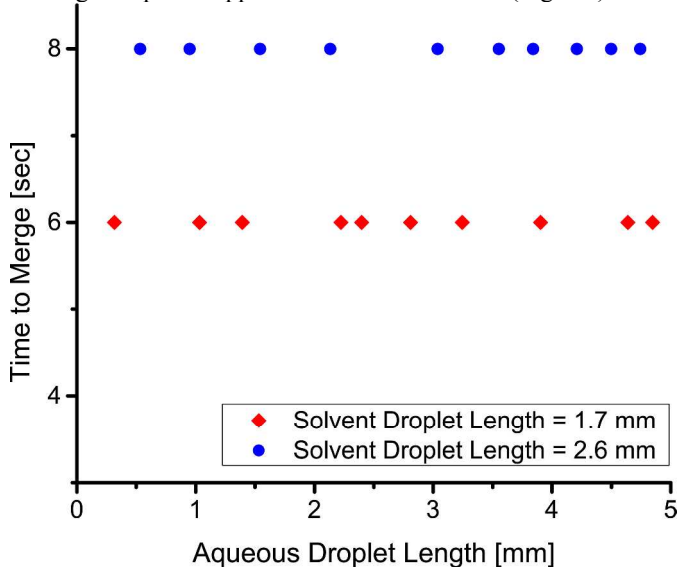
Fig. 7 The relation between the time to merge two aqueous droplets and the length of one of the aqueous droplets for a droplet velocity of 2.0 mm/s.
