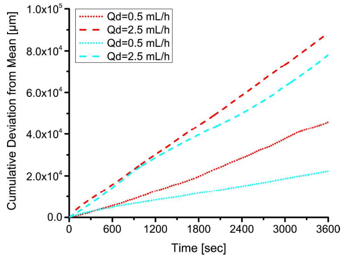
Fig. 4 The deviation in the size of droplets in coated (cyan) and uncoated (red) channels during an hour of operation at two different flow rate ratios and a continuous flow rate of 10 mL/h and various dispersed phase flow rates (Qd) as indicated in the legend. The deviations are calculated based on a constant, total mean.
