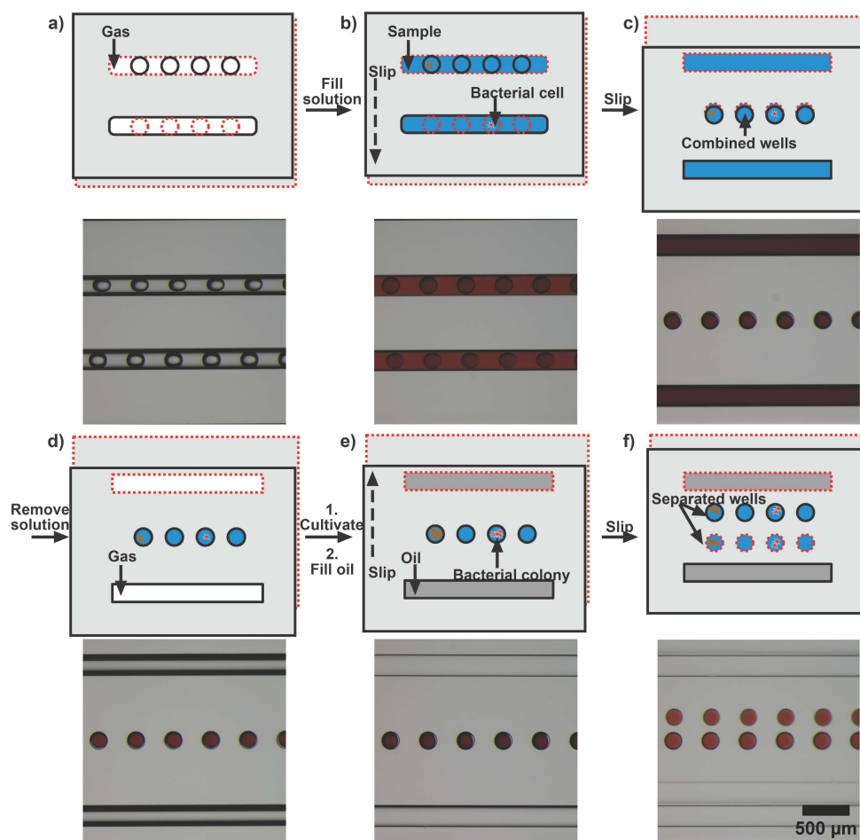
Fig. 2 Schematic drawings (top rows) and photographs (bottom rows) of a replica-SlipChip, illustrating device design for microbial culture and its operation visualized with red dye experiments. Top rows show illustrations of device operation with a sample containing a suspension of cells; bottom rows show representative photographs of the chip loaded with a red dye solution. (a) An empty chip was aligned so that wells and channels overlapped. The oil in the channel was removed by applying a vacuum to the inlets. (b) Sample was loaded. (c) The chip was slipped to overlap the wells in the two plates. (d) Channels were purged with a vacuum so that air was introduced through the inlets. The device was then incubated to promote microbial growth. (e) Channels were flushed with oil. (f) The chip was slipped to separate the overlapping wells and prepare their contents for splitting.
