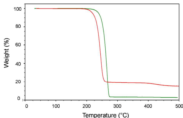
Figure 8. Comparison of TGA profiles for pure and impure P(3HB) obtained with SAS: i) P(3HB) recovered with 200 wt% \text{NH}_4 -laurate (— green line) and ii) P(3HB) recovered with 100 wt% \text{NH}_4 -laurate (— red line).
