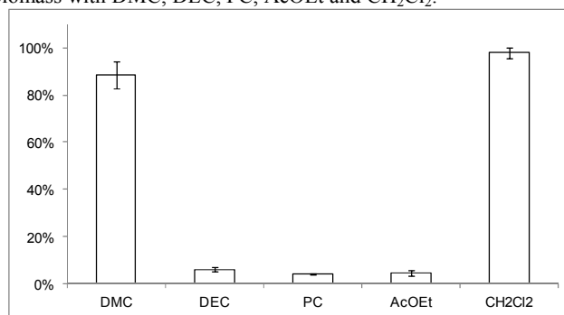
Figure 1. P(3HB) recovery (expressed as percentage of the polymer content in the cells) obtained after 4 h-extraction of freeze-dried biomass with DMC, DEC, PC, AcOEt and CH 2 Cl 2 .
