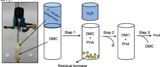
Figure 3. DMC-based protocol for the extraction of C. necator slurry.
