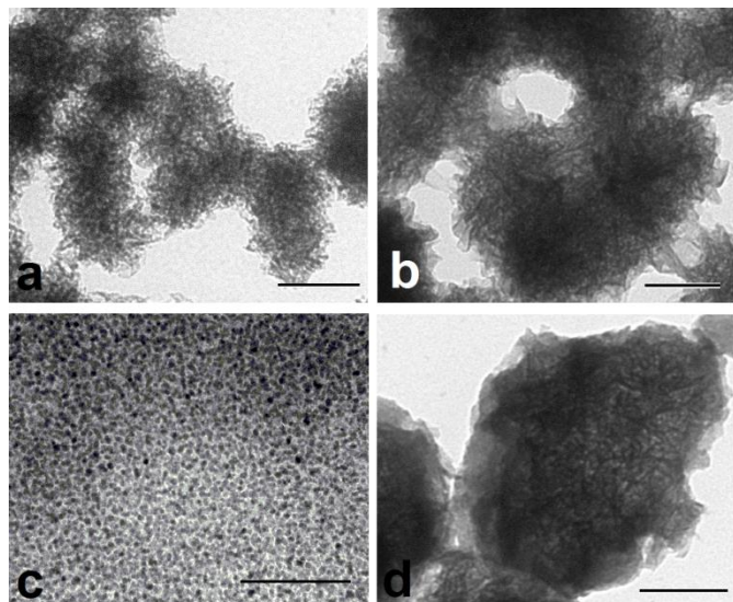
Fig. 2. TEM images showing (a) \text{Mn}_3\text{O}_4 -lactate; (b) \text{CaMn}_3\text{Ox} -lactate; (c) Co-lactate 1:1 (average size 4.5nm); (d) \text{CaMn}_3\text{Ox} -lactate recovered from photocatalytic reaction after 200 min with cobalt oxide coating formed in-situ. (Scale bars = 100nm)
