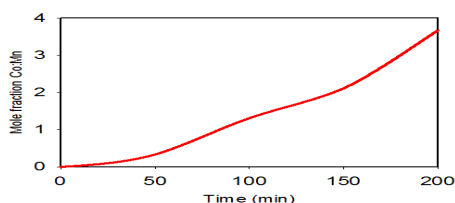
Fig. 8. Graph of increase in Co:Mn mole fraction for \text{CaMn}_3\text{Ox} -lactate samples recovered at intervals from photocatalytic reaction as measured by quantitative EDX analysis.
