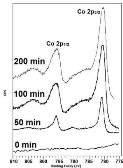
Figure 9. High resolution XPS analysis of \text{CaMn}_3\text{Ox} -lactate catalysed photocatalytic reaction with washed samples recovered at intervals showing accumulation of Co from decomposed electron acceptor. The Co2p region has band position and shape consistent with cobalt oxide as \text{Co}_3\text{O}_4 together with broader bands of increasing intensity indicating increasing hydroxide presence.
