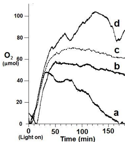
Fig. 6. Graph showing \text{O}_2 generation with \text{CaMn}_3\text{Ox} -lactate catalysts under different reaction protocols. (a) 10mg of \text{CaMn}_3\text{O}_6 stirred in reaction mixture in dark for 45 min prior to light on; (b) 10mg of \text{CaMn}_3\text{O}_6 added by injection to reaction flask at light on; (c) 10mg commercial nanoparticulate \text{Co}_3\text{O}_4 (for comparison); (d) 10 mg of in-situ formed Co-Mn oxide lactate recovered from previous 200min \text{CaMn}_3\text{Ox} -lactate photocatalytic reaction.
