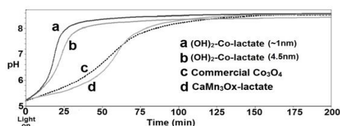
Fig. 5. Change in pH for a photocatalytic water oxidation utilizing [\text{Ru}(\text{bipy})_3\text{Cl}]^{2+} , [\text{Co}(\text{NH}_3)_5\text{Cl}]^{2+} (electron acceptor) and catalyst suspended in \text{N}_2 degassed aqueous acetate buffer solution at pH 5.2. Time course using Co-lactates, \text{CaMn}_3\text{Ox} -lactate, and commercial \text{Co}_3\text{O}_4 (with 10mg metal oxide present in all cases).
