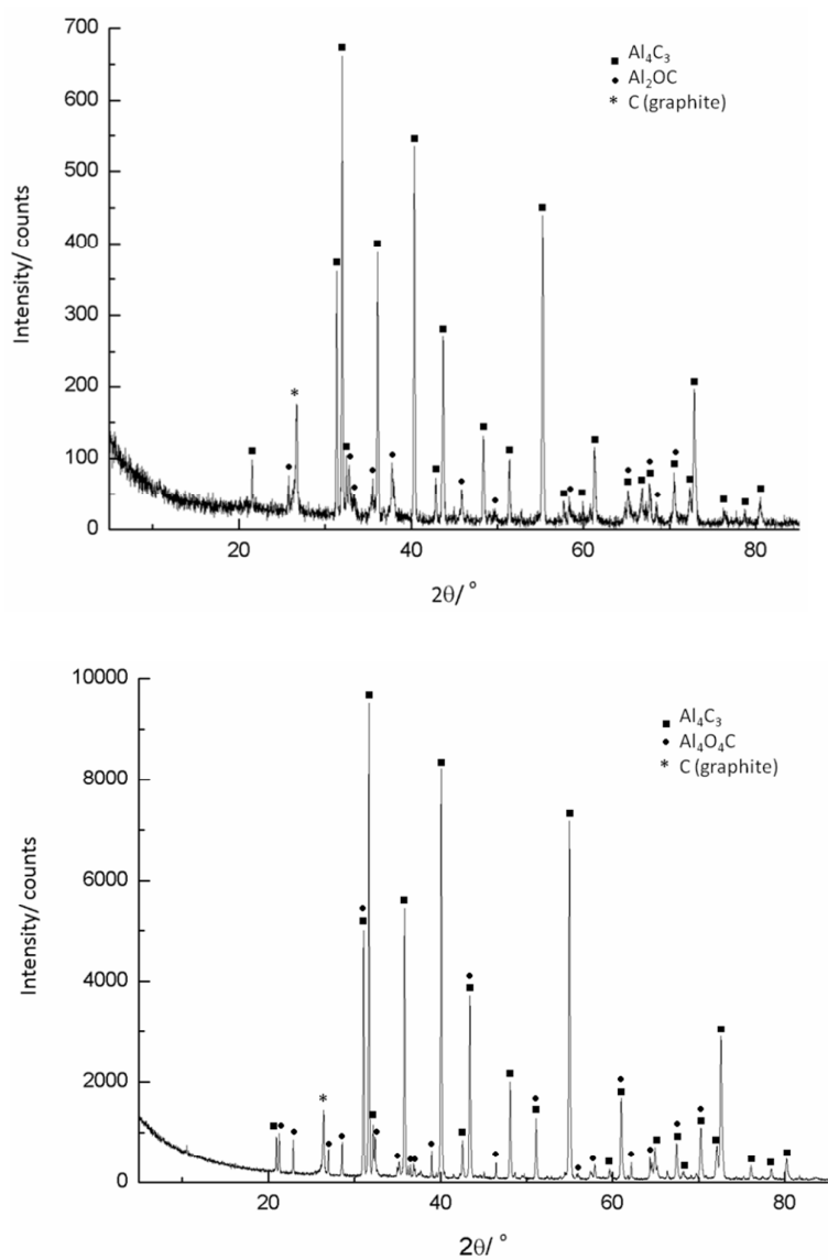
Fig. S3 Ex-situ PXD patterns from typical 4 Al + 3 C reactions performed in air for 30 min using graphite powder as a susceptor in the MMC reactor.
