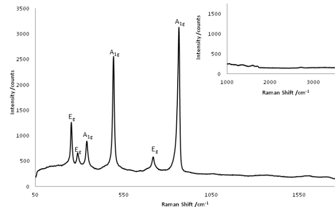
Fig. 6 Raman spectrum of \text{Al}_4\text{C}_3 showing the six characteristic bands of the carbide and the absence of carbon D and G bands (inset).
