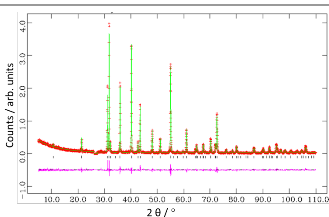
Fig. 4 Observed (pluses), calculated (solid green line), and difference (solid purple line) profile plot for the Rietveld refinement against powder XRD data for aluminium carbide. Tick marks denote \text{Al}_4\text{C}_3 diffraction peaks. The graphite reflection at 2\theta \sim 27^\circ was excluded from the refinement.
