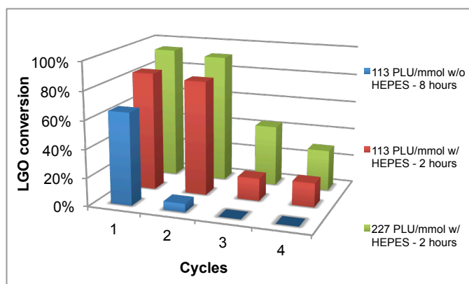
Figure 5. LGO conversion after repeated use of CAL-B with or without HEPES
