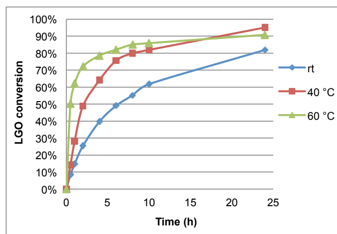
Figure 2. Effect of temperature on LGO oxidation kinetics
