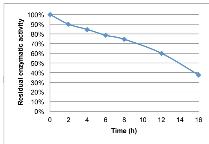
Figure 3. Residual activity of CAL-B during the lipase-mediated oxidation of LGO (Measured using lauric acid method - see experimental section)
