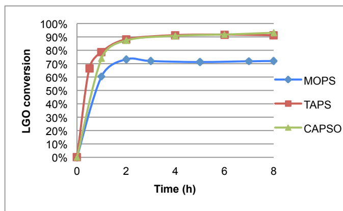
Figure 4. Effect of solid buffer on the lipase-mediated oxidation of LGO
