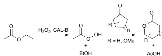
Scheme 2. Lipase-mediated Baeyer-Villiger oxidation of cyclic ketones using AcOEt as acyl donor and H 2 O 2 as oxidant
