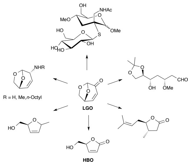
Figure 1. Some chemical intermediates obtainable from LGO
