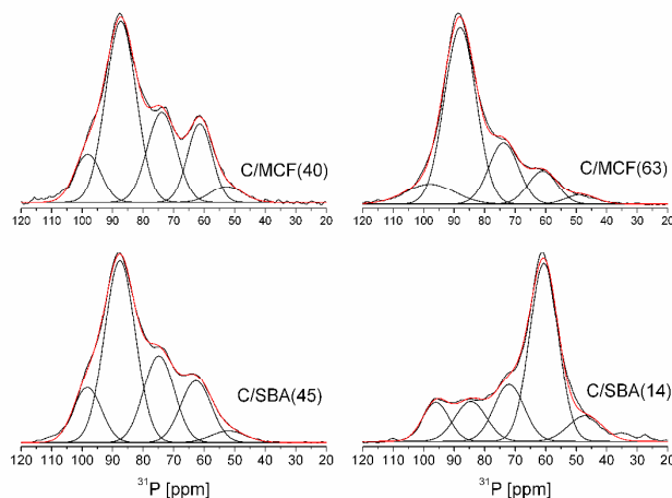
Fig. 5. 1 H-decoupled 31 P MAS NMR of the mesoporous C/S composites.
