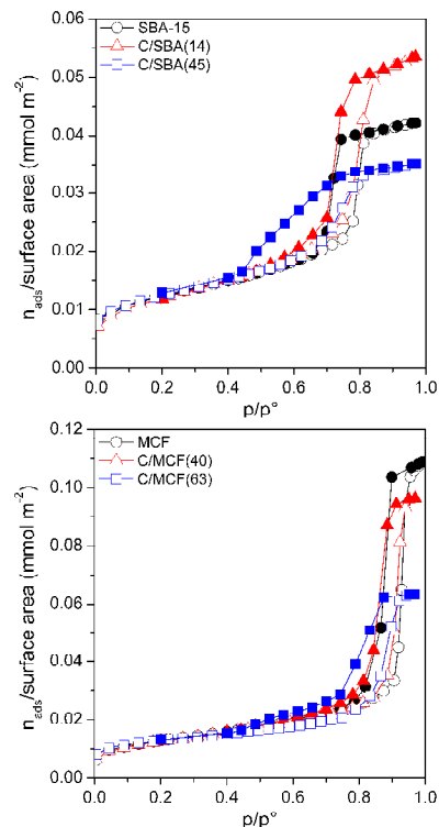
Fig. 2. Nitrogen adsorption-desorption isotherms at -196 °C of the C/S composites and corresponding uncoated silicas, plotted as amount adsorbed per unit of surface area (open symbols-adsorption; closed symbols-desorption).
