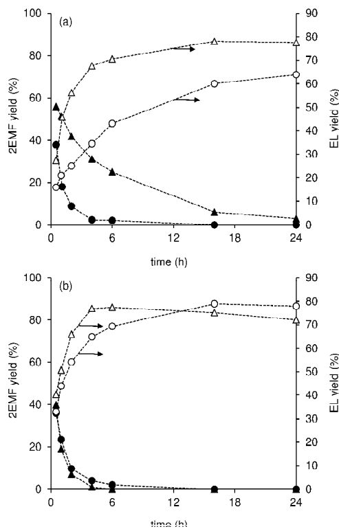
Fig. 9. Dependency of the yields of 2EMF (black symbols) and EL (white symbols) on the time of reaction of FA (until 24 h) in the presence of the composites (a) C/SBA-15 (C/SBA(45) (triangles), C/SBA(14) (circles)) or (b) C/MCF (C/MCF(63) (triangles), C/MCF(40) (circles)); FA conversion was always 100%. Reaction conditions: 0.33 M FA, catalyst loading=10 g cat dm -3 , 110 °C. The dashed lines are visual guides.
