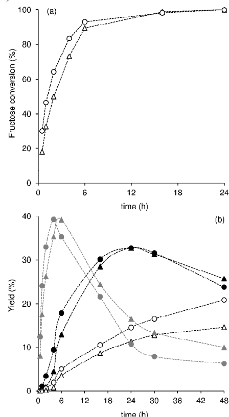
Fig. 8. (a) Kinetic profiles and (b) dependency of the yields of HMF (grey symbols), SEMF (black symbols) and EL (white symbols) on the time of reaction of fructose in the presence of C/SBA(45) (triangles) or C/MCF(63) (circles). Reaction conditions: 0.33 M fructose, water-ethanol (3:7 v/v ratio) solvent mixture, catalyst loading=10 g cat dm -3 , 140 °C. The dashed lines are visual guides.
