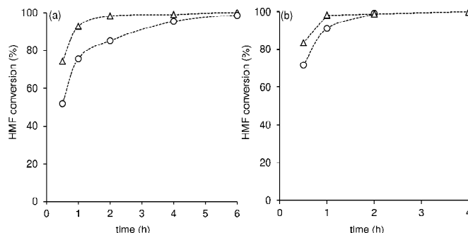
Fig. 6. Kinetic profiles of the reaction of HMF with ethanol in the presence of the composites (a) C/SBA-15 (C/SBA(45) ( \Delta ), C/SBA(14) (O)) or (b) C/MCF (C/MCF(63) ( \Delta ), C/MCF(40) (O)). Reaction conditions: 0.33 M HMF, catalyst loading = 10 \text{ g}_{\text{cat}} \text{ dm}^{-3} , 110 °C. The dashed lines are visual guides.
