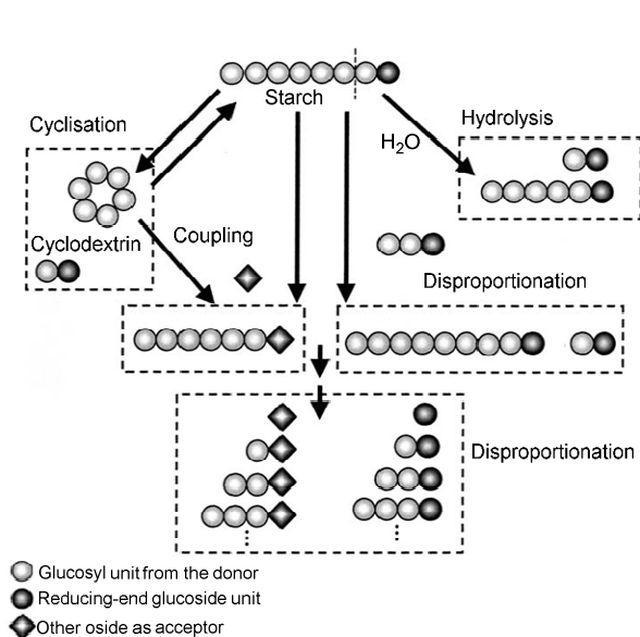
Fig. 1 Reactions catalyzed by cyclodextrin glucosyl transferases.
