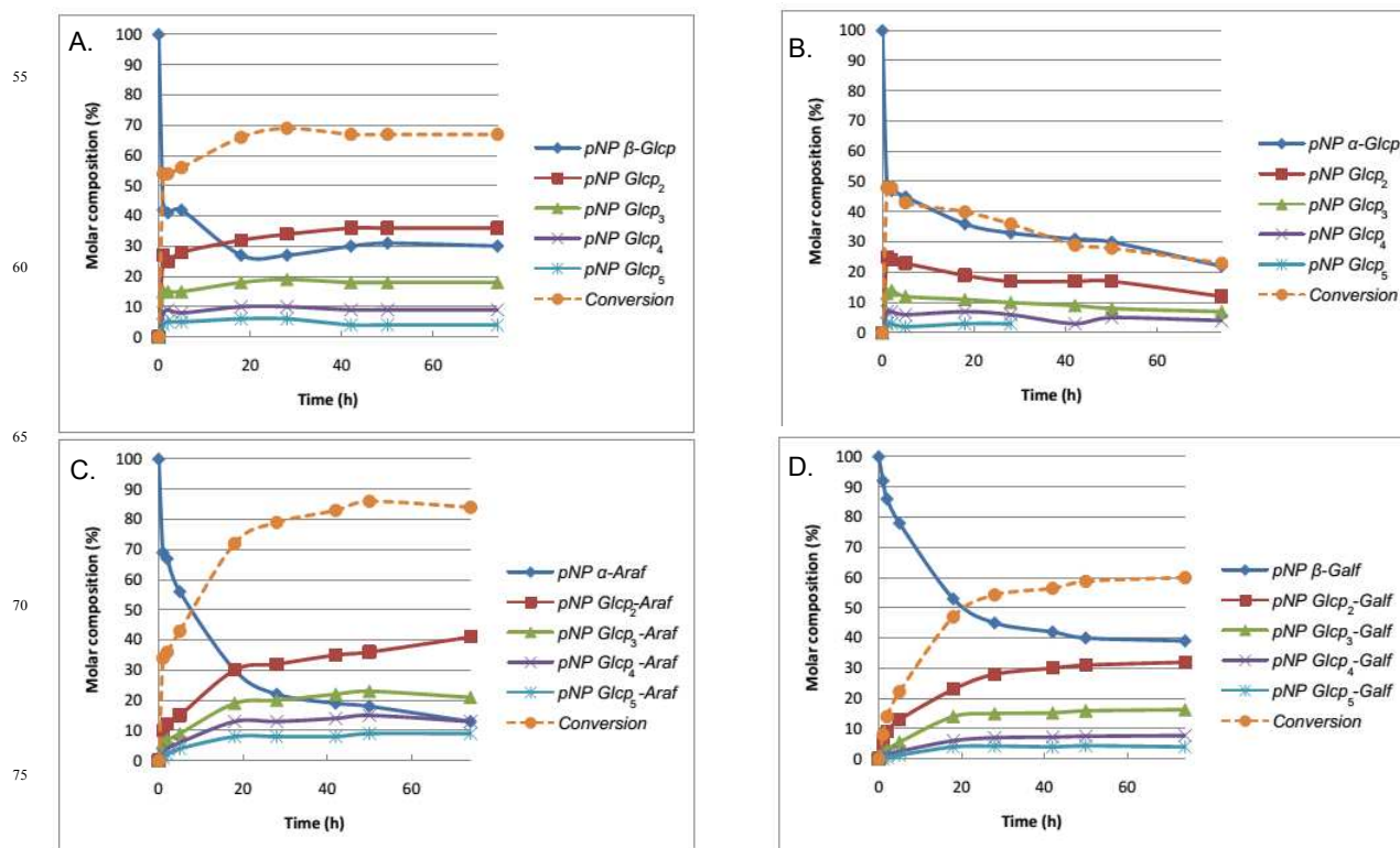
Fig. 3 Kinetic profile of the reaction catalyzed by CGTase between cyclodextrin and 1 (A.), 2 (B.), 3 (C.) and 4 (D.).
