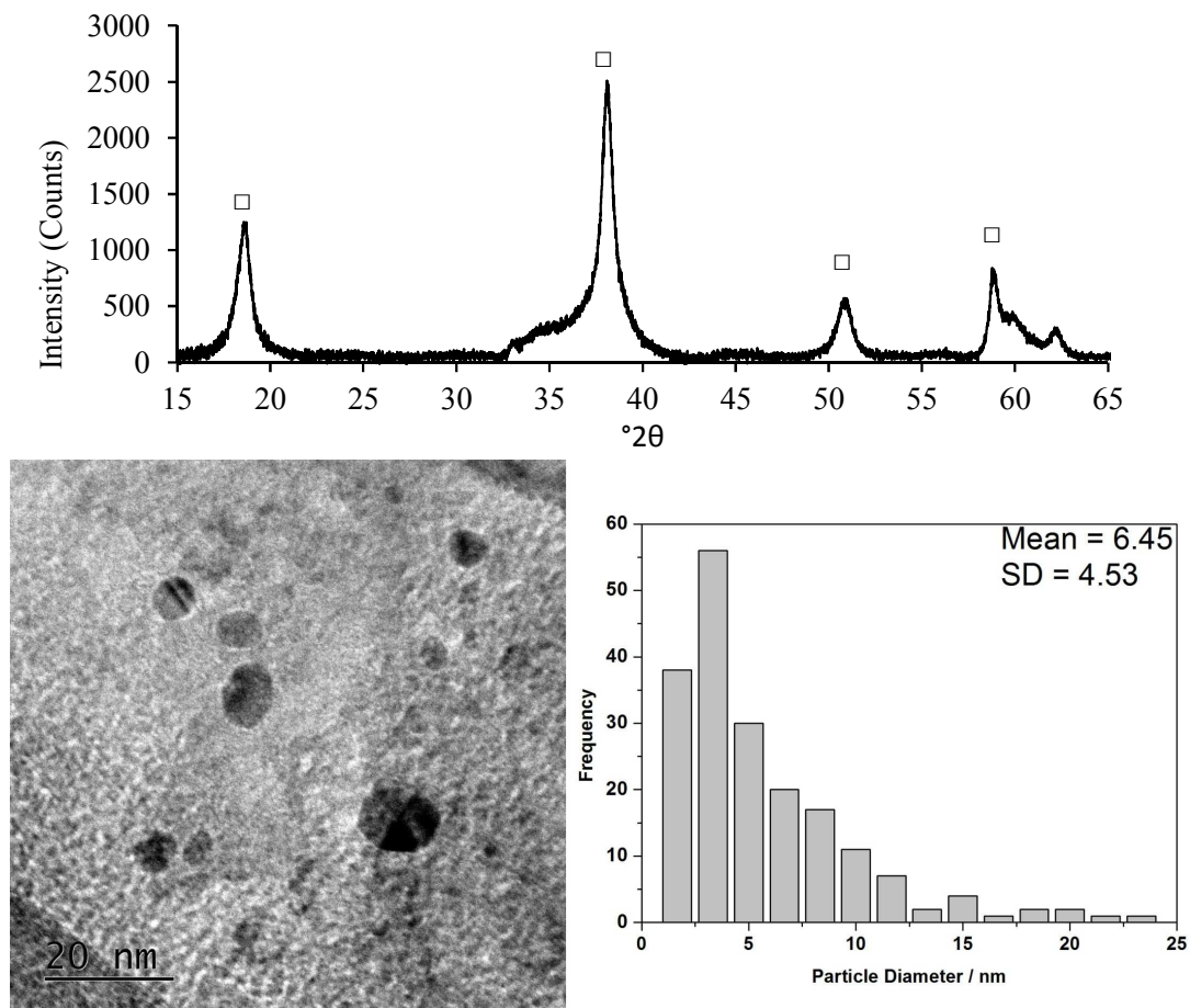
Figure 6: Characterisation of AuPd/MgO catalyst after use in the base free glucose oxidation reaction at 50 °C. Upper figure shows XRD diffraction pattern of catalyst with \square indicating reflections associated with \text{Mg}(\text{OH})_2 . Lower figures show a representative TEM image of metal nanoparticles on the used catalyst (left) and the corresponding particle size distribution.
