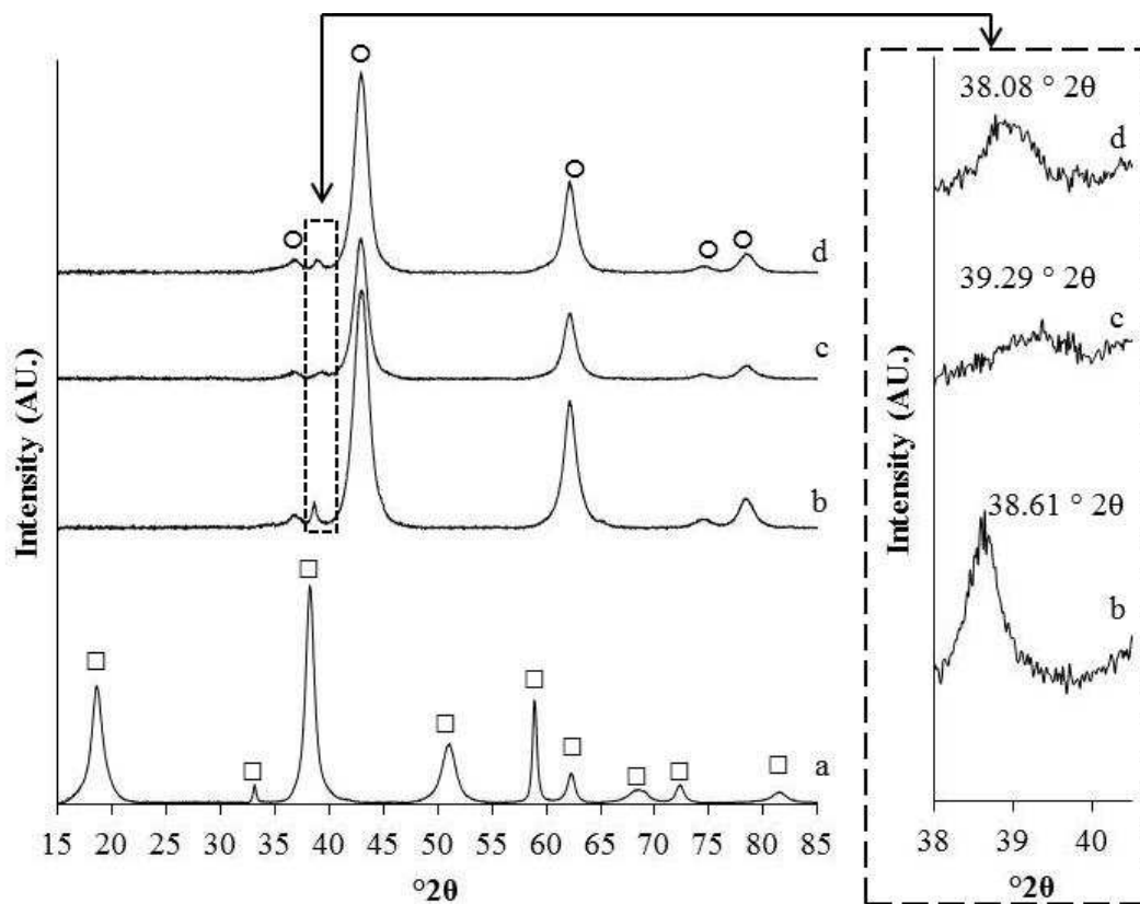
Figure 2: XRD patterns of the 0.5% Au-Pd/Mg(OH) 2 catalyst after various heat treatments; a) dried, b) dried with calcination at 450 °C, c) dried with heat treatment under nitrogen and d) dried with both heat treatments. Expanded region shows the position of [111] cubic metal phase reflection.
