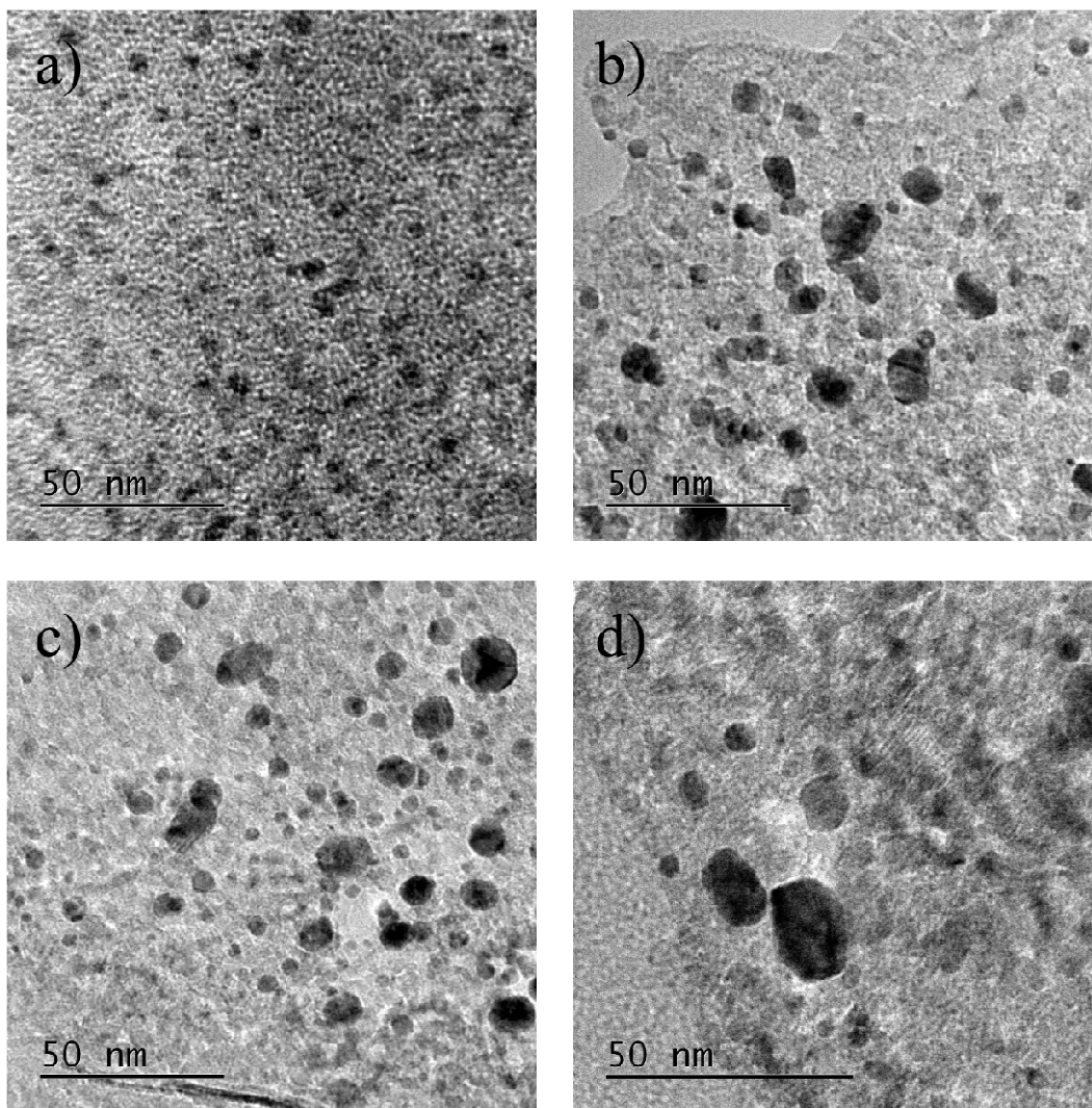
Figure 3: TEM images of the 0.5%Au-Pd/Mg(OH) 2 catalyst after various heat treatments; a) dried, b) dried with calcination at 450 °C, c) dried with heat treatment under nitrogen and d) dried with both heat treatments.
