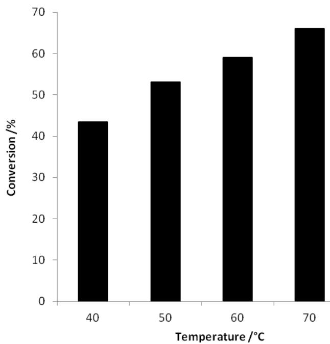
Figure 1: The conversion of glucose using Au-Pd/MgO (b) : Reaction conditions: glucose (5 ml, 0.5M), catalyst (0.06g), 24h at atmospheric pressure, selectivity 100% except at 70 °C which was 98%.
