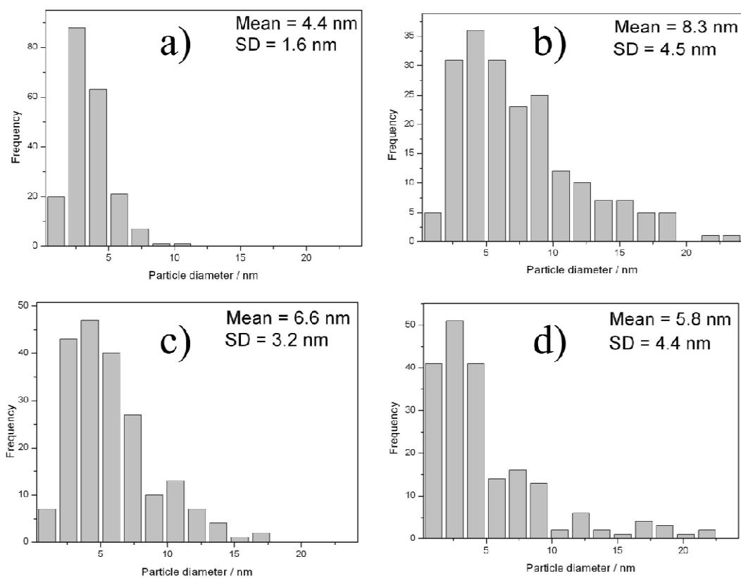
Figure 4: TEM particle size distributions of the 0.5%Au-Pd/Mg(OH) 2 catalyst after various heat treatments; a) dried, b) dried with calcination at 450 °C, c) dried with heat treatment under nitrogen and d) dried with both heat treatments.
