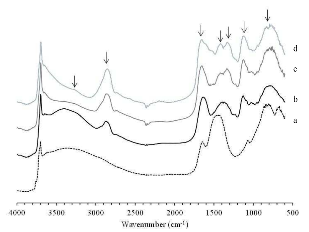
Figure 7. DRIFTS analysis of AuPd/MgO catalyst (a) before reaction, (b) after base free glucose oxidation reaction at 50 °C, (c) in situ spectra of post reaction sample heated to 115 °C and (d) in situ spectra of post reaction sample heated to 440 °C. In situ spectra were recorded on samples at designated temperature under vacuum. Arrows indicate bands associated with adsorbed organic species.
