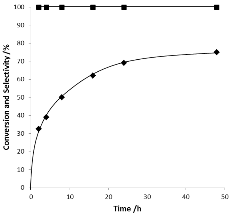
Figure 5: Time on line data for the oxidation of glucose using the 0.5% Au-Pd/MgO catalyst. Reaction condition: glucose (5 ml, 0.5M), catalyst (0.06g), 50 °C at atmospheric pressure.
