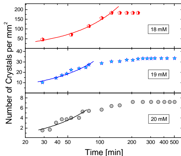
Fig. 4 Number of crystals as a function of time in a normalized area from Figure 3 for samples with 18 mM, 19 mM and 20 mM \text{CdCl}_2 . For the 19 and 20 mM plots, three series of picture sets were analyzed and averaged for better statistics.
