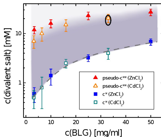
Fig. 2 Experimental phase diagram of BLG with \text{ZnCl}_2 and \text{CdCl}_2 31,47 . Both salts share the similar c^* , below and above which the protein solutions are clear and turbid, respectively. Further increasing salt concentration, samples become gradually less turbid, but not completely clear again, and this transition zone is denoted as pseudo – c^{**} . The black ellipse marks the conditions mainly used in this work (33 mg/ml BLG with 15-20 mM \text{CdCl}_2 ).
