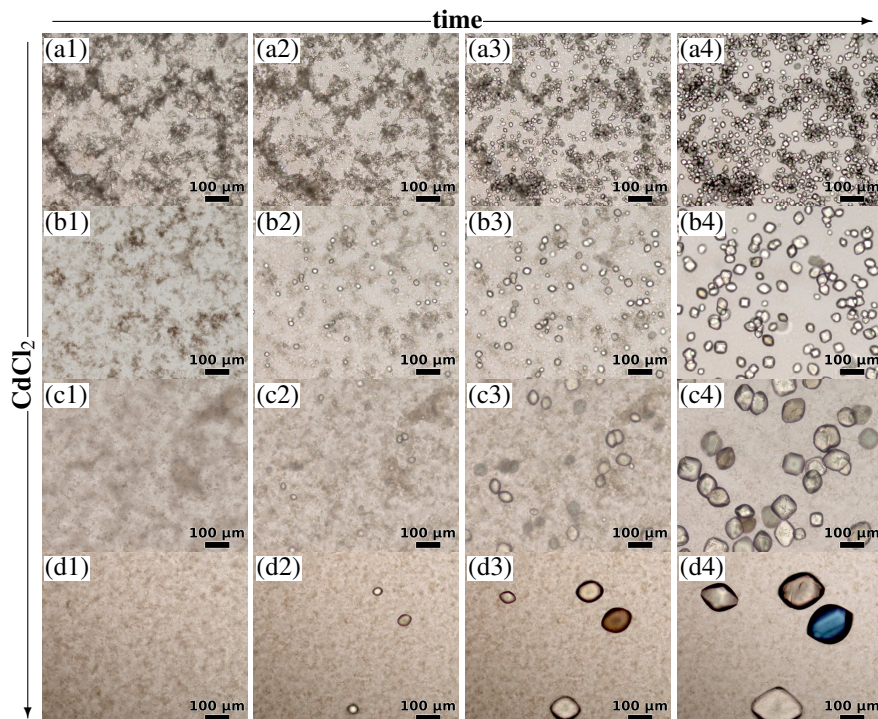
Fig. 3 Image series of protein crystallization for samples with a BLG concentration of 33 mg/ml and \text{CdCl}_2 at different time: (a) 17 mM, (b) 18 mM, (c) 19 mM and (d) 20 mM (increasingly less turbid). (a1) 0, (a2) 50 min (a3) 75 min (a4) 100 min after preparation. (b1) 0 (b2) 75 min (b3) 100 min (b4) 3 h. (c1) 0, (c2) 100 min, (c3) 3 h, (c4) 6 h. (d1) 0, (d2) 3 h, (d3) 6 h and (d4) 10 h. Videos of the crystallization process in (a) and (d) can be found in online supporting materials.
