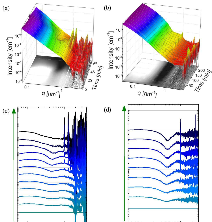
Fig. 7 Protein crystallization followed by real-time SAXS measurements. Samples contain 33 mg/ml BLG with 17 mM CdCl 2 (a&c) and 20 mM CdCl 2 (b&d), located in the transition zone of pseudo-c** (i.e. at the upper end of regime II). (a&b) Three-dimensional plot of I(q,t) . The bottom projections are created from I(q,t)/I(q,t=0) and thus monitor the evolution of the curves with time. (c&d) Selected I(q,t)/I(q,t=0) curves for the evolution of Bragg peaks and the amorphous peak. Data are shifted upward by a constant factor for better visibility.
