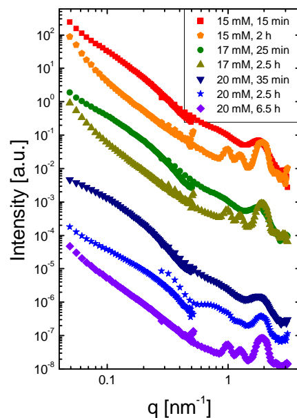
Fig. 6 BLG 33 mg/ml with 15, 17 and 20 mM \text{CdCl}_2 in \text{D}_2\text{O} measured by SANS. Data are shifted upward for clarity. The mismatch of the SANS curves (especially visible for 20 mM after 2.5 h) was caused by measurements at different detector positions together with the fast kinetics occurring in the sample.
