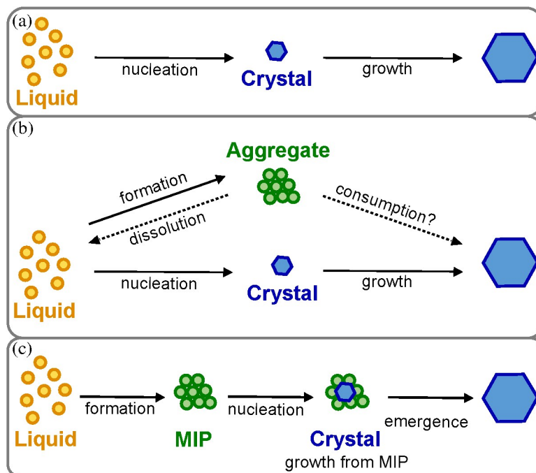
Fig. 1 Illustrations of different pathways of crystal nucleation and growth. (a) Classical one-step pathway. (b) Parallel process of aggregate formation and crystal nucleation. (c) Multi-step process with precursor (MIP) for nucleation.
