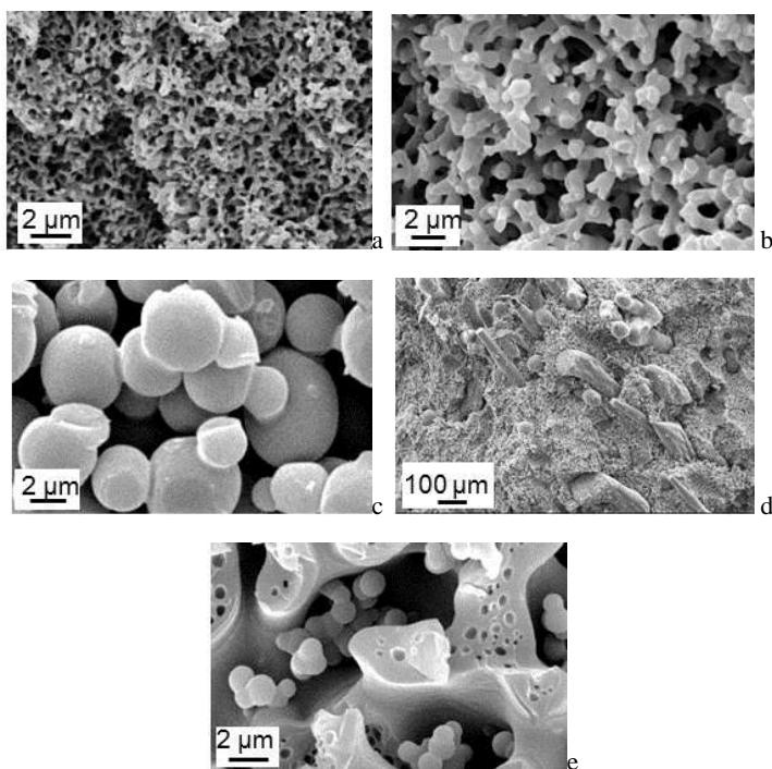
Fig. 8 Scanning electron micrographs of different types of structures; a, b – bicontinuous (a- VTM266 and b- MVR444 based); c, d, e - complex structure (MTM57 based); note that c,d is the same sample at different magnifications.
