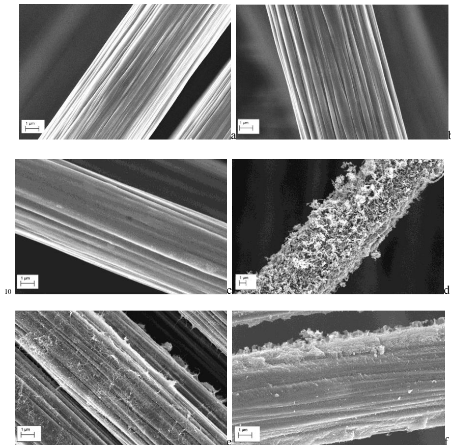
Fig. 2 Scanning electron micrographs of (a) as-received, (b) heat-treated, (c) KOH activated carbon fibres, (d) CNT grafted carbon fibres, (e) CNT sizing carbon fibres, (f) CAG modified carbon fibres.
