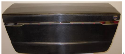
Fig. 11 Structural supercapacitor flat laminate (a); model car body (b) and trunk lid with added chrome trimming and lit LED lights (c).
