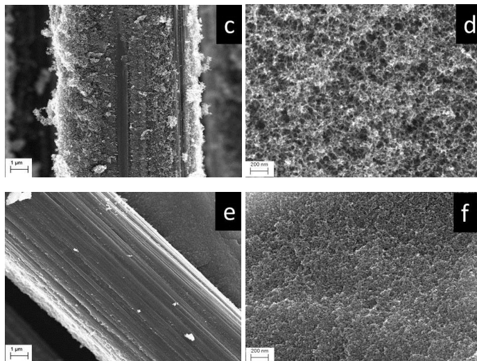
Fig. 5 Scanning electron micrographs of CAG modified carbon fibres prepared using different amounts of RF (a, b) 25wt%, (c, d) 40 wt% (d, e) 50 wt%. For each sample two different magnifications are presented.
