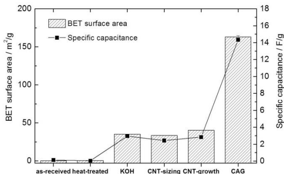
5 Fig. 1 Effect of different types of carbon fibres modifications on BET surface area and specific capacitance of CF/GF/CF composite. (Electrolyte used – 3M KCl; Specific capacitance was calculated from cyclic voltammetry, range -0.2V - +0.2V, scan rate 5 MV/s)
