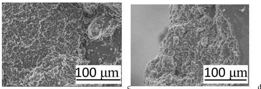
Fig. 10 Scanning electron micrographs of 50/MTM57 with and without different thixotropes; a – neat; b – Aerosil; c – Cab-o-sil; d – Garamite
