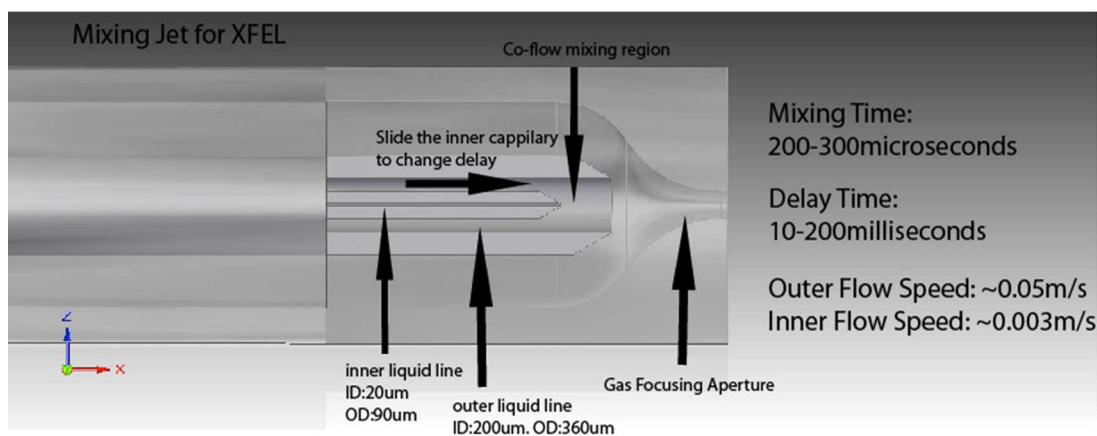
Figure 3. Mixing jet, showing three concentric tubes and nozzle. Two fluids are mixed in a short mixing time, then allowed to react for a delay time before emerging from the nozzle in jet a few microns in diameter. This is intercepted by the pulsed X-ray beam. By sliding the inner tube, the delay time can be adjusted.
