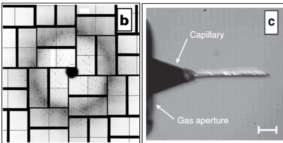
Figure 4. (b) Diffraction from serotonin receptor 5-HT 2B in cholesterol-doped 9.9 MAG + 7.9 MAG LCP. No sharp rings are visible suggesting that formation of L c phase has been avoided (X-ray intensity attenuated to 3.1% due to strong Bragg diffraction from 5x5x5 μm 3 sized crystals, 1.5 μm X-ray beam diameter, 50 fs pulse length, 9.5 keV, 50 μm LCP jet diameter, 190 nL/min flow rate, 120 Hz pulse rate). The resolution at the detector edge in both panels 2.5 Å. [12]
