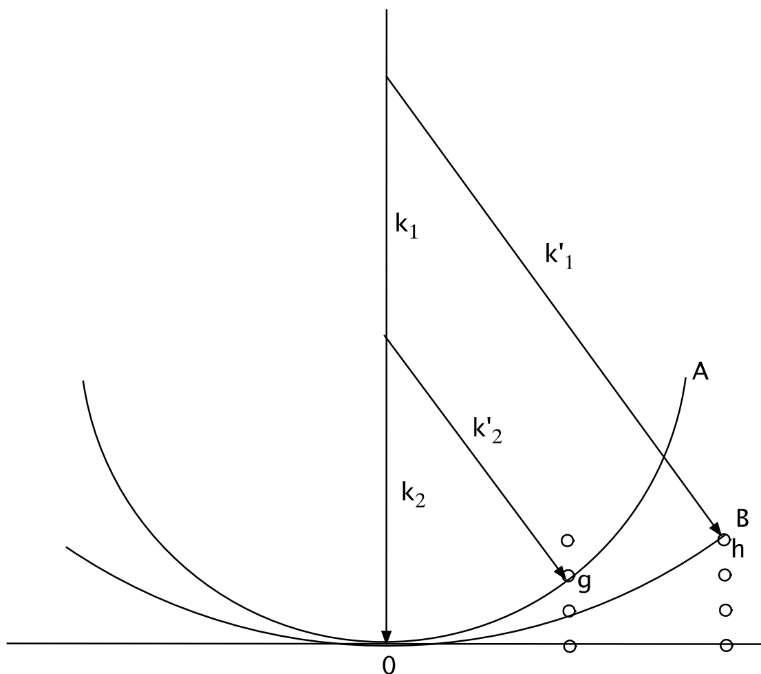
Figure 1. Ewald sphere scattering geometry for two wavelengths scattering from different reflections into the same detector pixel. With a bandwidth spanning wavevectors from \mathbf{k}_1 to \mathbf{k}_2 , all Bragg reflections falling within the area AOB are excited.
