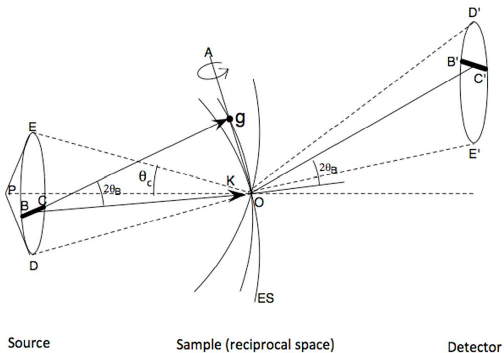
Figure 2. Coherent convergent-beam diffraction geometry, showing source DE, Ewald sphere ES and detector E'D'. Point source P fills illumination aperture DE coherently. Limiting Ewald sphere orientations (eg ES) are defined by marginal rays DO and EO. Plane-wave component K of converging spherical wave (with beam divergence \theta_B ) from midpoint of BC arrives at detector at midpoint of B'C'. Rotation of arrowed wavevectors originating along line BC about OA preserves the Bragg condition for reciprocal lattice vector g , defining line C'B' at detector along which the Bragg condition is satisfied, producing Bragg lines instead of spots. The disk E'D' is an inverted image of ED.
