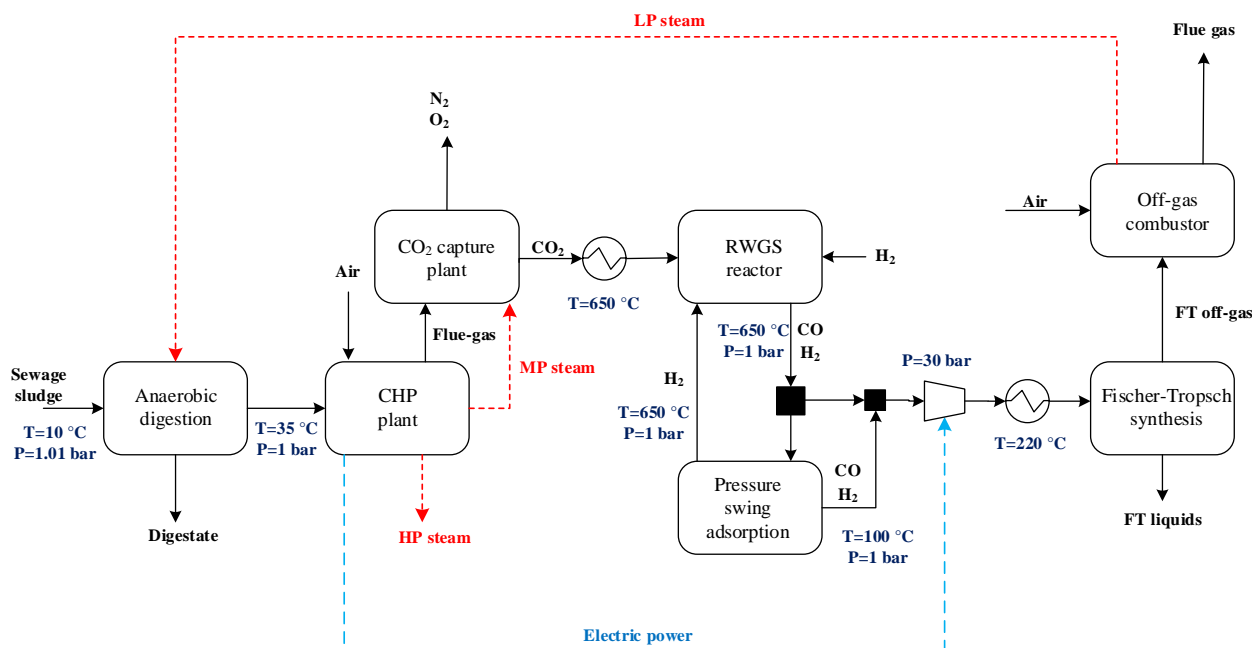
Fig. 5 Process flow diagram for PD-CHP3
