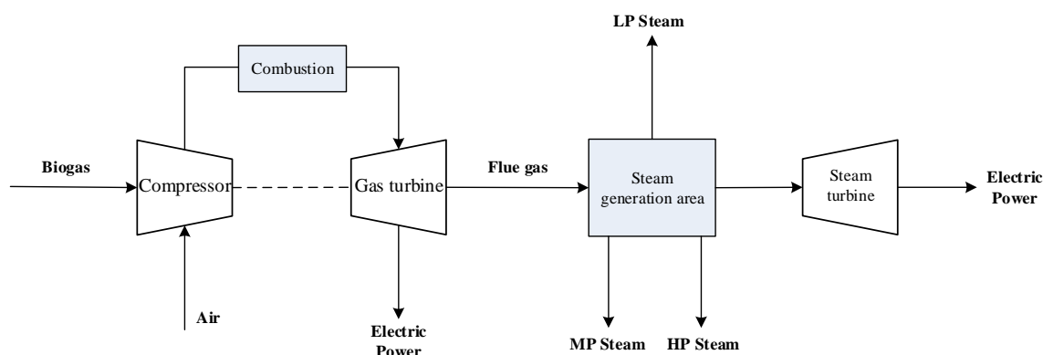
Fig. 7 Process flow diagram of the CHP plant
