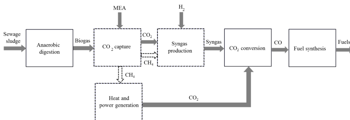
Fig. 1 An overview of the \text{CO}_2 utilisation system for production of synthetic fuels [MEA: monoethanolamine. Dashed lines represent steps which are not present in all design options; see Table 1 for details. In some design cases the heat and electricity generation plant is placed before \text{CO}_2 capture].
