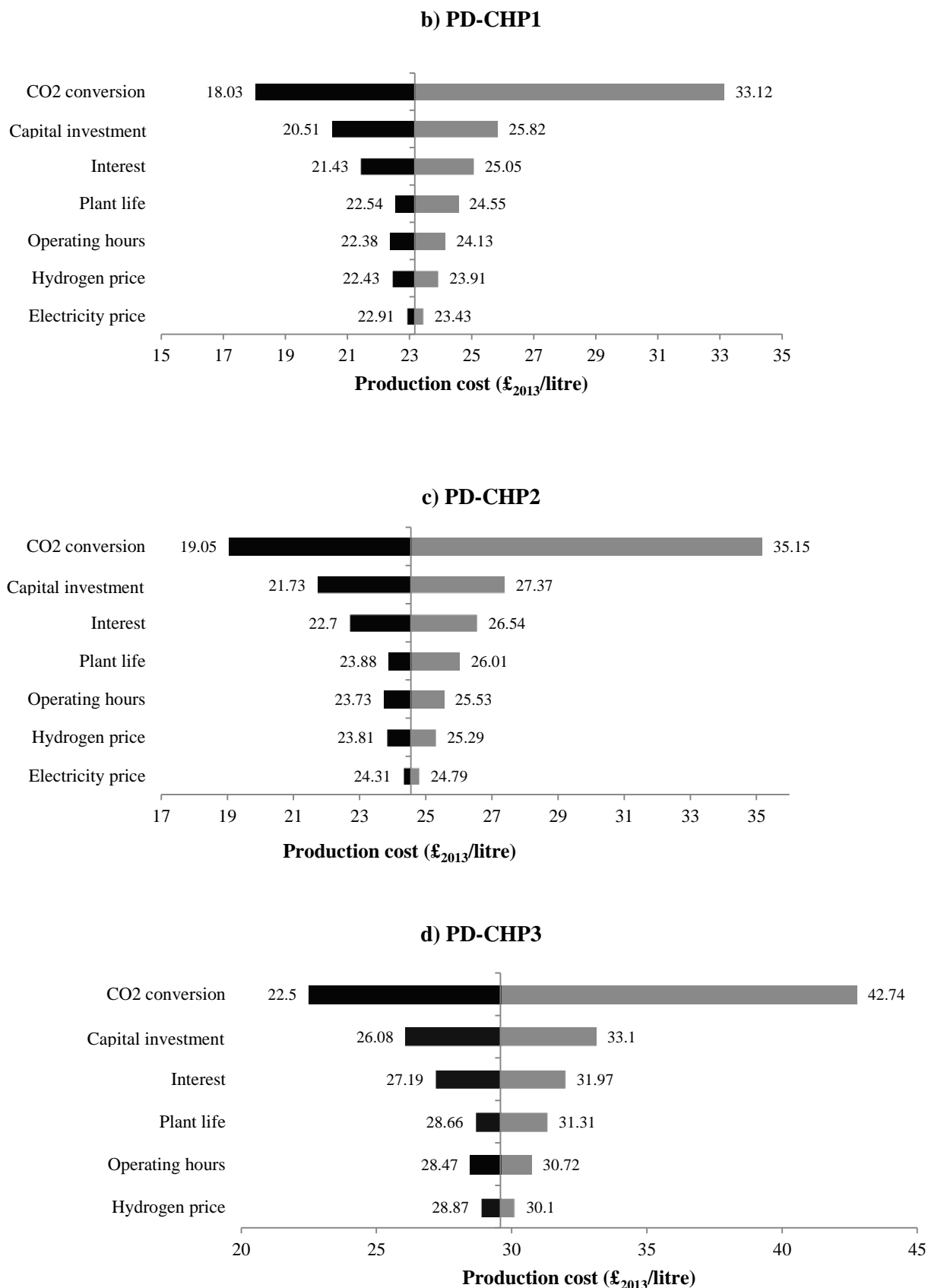
Fig. 12 Sensitivity of fuel production costs to variations of selected technical and economic parameters. [All parameters are varied by \pm 30\% , except for the plant operating hours which are varied by \pm 10\% . The vertical line in the graphs represents the production cost of the base case for the different designs.]
