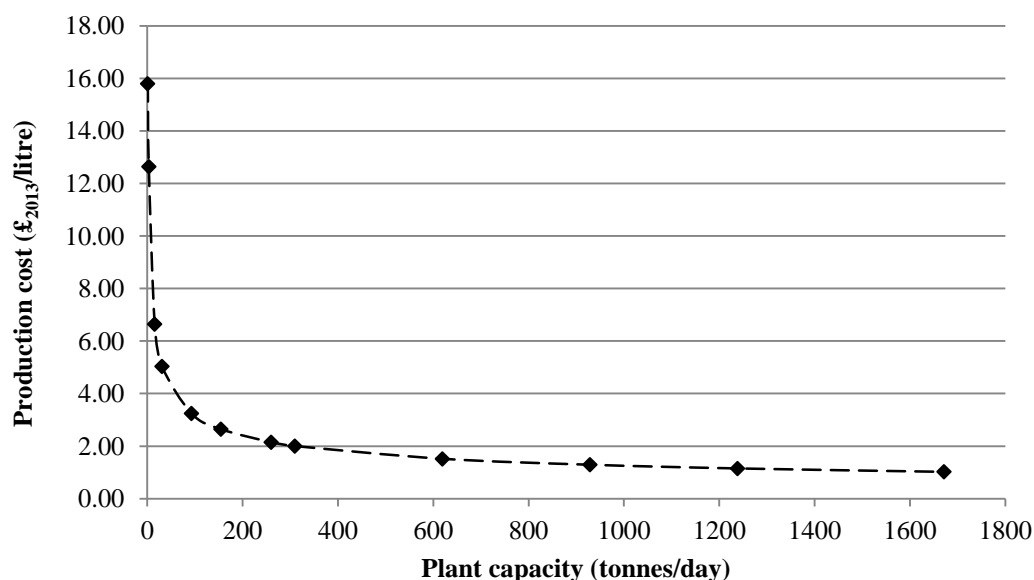
Fig. 10 Cost of liquid fuels in £/litre for different plant capacities for PD-MEA
