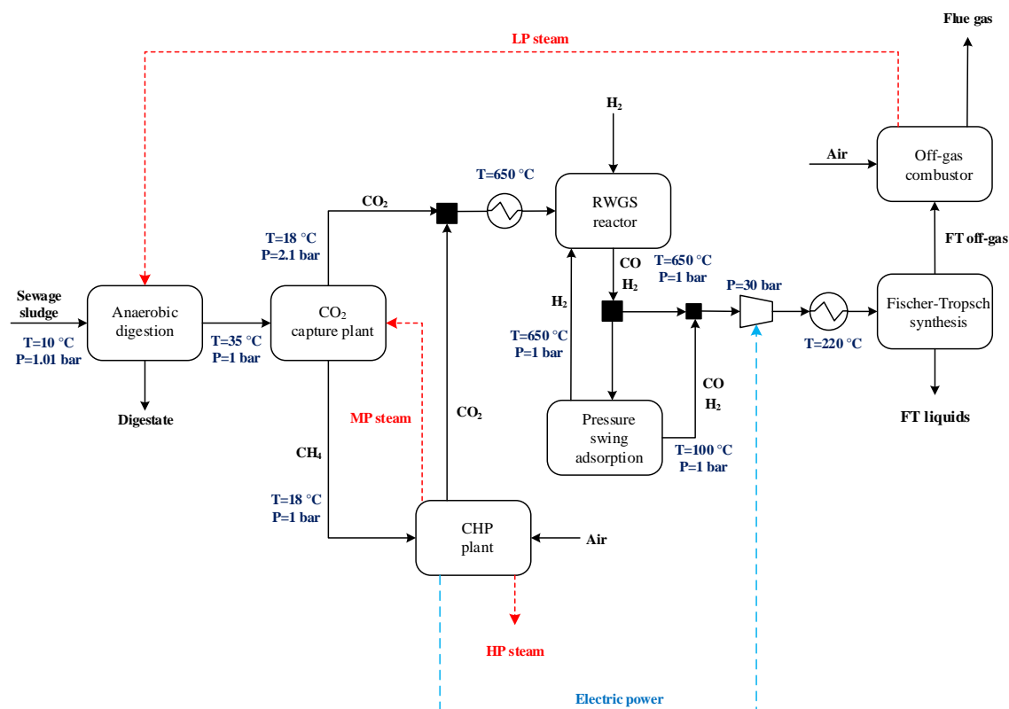
Fig. 4 Process flow diagram for PD-CHP2
