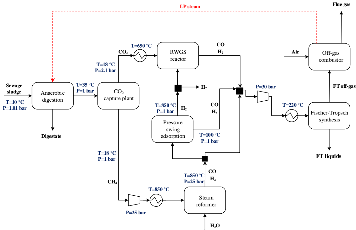
Fig. 2 Process flow diagram for PD-MEA
