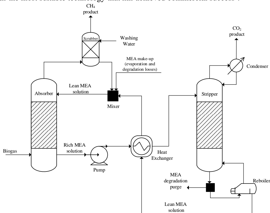
Fig. 6 Process flow diagram of CO 2 capture
