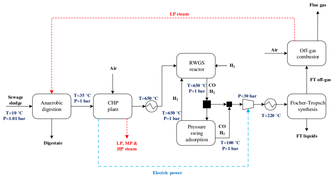
Fig. 3 Process flow diagram for PD-CHP1
