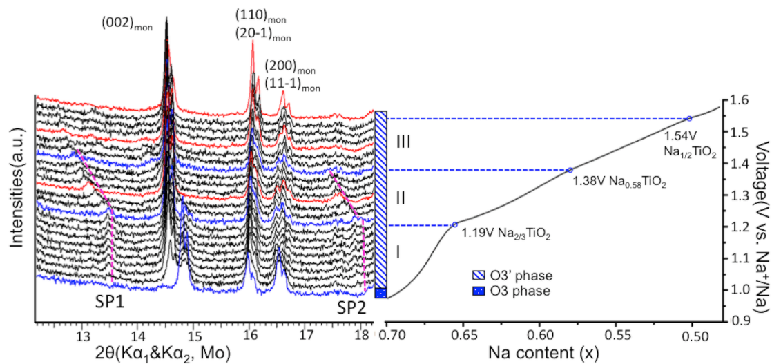
Figure 6. Superstructure evolution from in situ XRD during electrochemical test. In situ XRD was collected during PITT charge of 0.03-V step size with 4 hour (blue and black) or 10 hour (red) scan per spectrum. The purple dashed lines represent the evolution of the superstructures (SP1 and SP2). The galvanostatic charge curve is shown on the right to illustrate the three regions divided by the inflection points explained in Figure 5, as represented by the blue XRD spectra and dashed lines.
