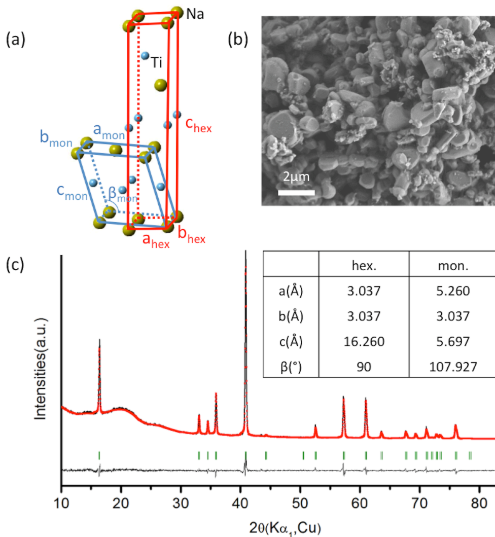
Figure 2. (a) Schematic illustration of O3-type and O'3-type structures. The yellow and blue spheres represent Na and Ti, respectively. (b) SEM image of as-prepared NaTiO 2 , which shows an average particle size of 1 to 2 \mu\text{m} . (c) X-ray diffraction pattern and Rietveld refinement of the as-prepared O3 NaTiO 2 . The Bragg peak positions are indicated by the short vertical lines. The black (red) line represents the experimental (calculated) data. The background and three broad peaks between 10^\circ - 30^\circ originate from the Kapton film used to seal the sample. The refinement results are performed in the R-3m space group and yield R_{\text{wp}} = 11.06\% and goodness of fit = 1.28. In the inset, lattice parameters in a monoclinic cell are given for comparison with that of the hexagonal cell.
