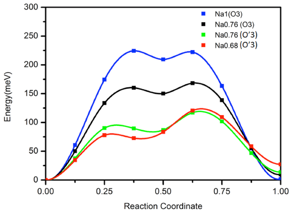
Figure 7. Calculated diffusion barrier for Na in the O3 and O'3 phases using the di-vacancy mechanism. Details of the calculation are given in the Methods.
