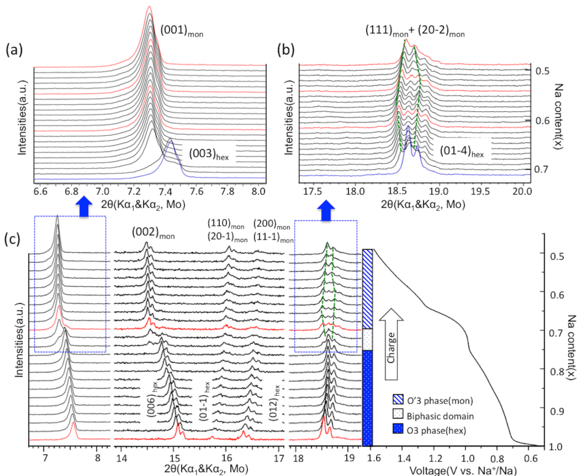
Figure 4. Structural evolution during electrochemical desodiation of O 3 -NaTiO 2 . (a),(b) In situ X-ray diffraction patterns recorded during the PITT experiments centered around the (003) hex , (001) mon reflections and (01-4) hex , (111) mon + (20-2) mon reflections, respectively. Note that X-ray source is Mo with K \alpha_1 and K \alpha_2 . The green dash lines illustrate the evolution of K \alpha_1 reflections in O'3 phase region. The red XRD spectra are further explained in Figure 6. (c) In situ XRD patterns during the first galvanostatic charge at a current rate of C/20 in the voltage range between 0.5 V and 1.6 V. The regions corresponding to (a)(b) are marked by the dashed boxes. Note that in the entire 2\theta range, preferred orientation for (00 l ) reflections exists because the electrode films were prepared using a dry method that involved multiple pressing and rolling processes.
