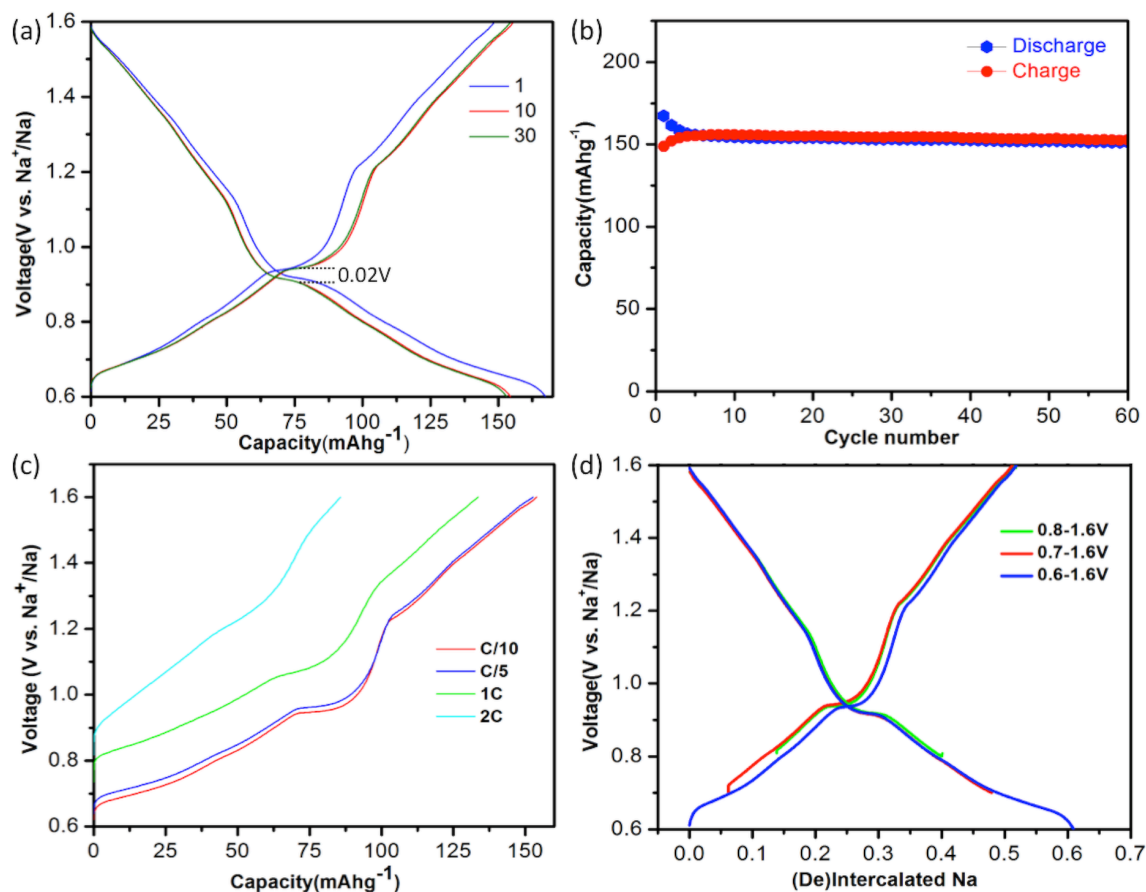
Figure 3. Electrochemical performance of NaTiO 2 . (a) The 1 st , 10 th and 30 th galvanostatic charge/discharge curves at a current rate of C/10 in the voltage range of 0.6-1.6 V versus Na + /Na. The voltage curve of the battery pre-discharged to 0.6 V is not shown for simplicity (see Supplementary Figure S1(b)). (b) Cyclability. The charge/discharge capacity versus cycle number at a current rate of C/10. (c). Rate capability. The battery was discharged to 0.6 V at a current rate of C/20 and then charged to 1.6 V at different rates from C/10 to 2C. (d) Comparison of the amount of cycled Na in voltage windows with lower cut-off voltages from 0.6- 0.8 V.
