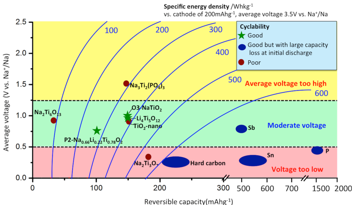
Figure 1. Average voltage versus reversible capacity for various reported anode materials for Na-ion batteries. Lines of constant specific energy density are also shown, assuming a cathode of 200mAh/g at 3.5 V average voltage. The specific energy density is calculated from full cells with a balanced weight of anode and cathode. The cycling performance is based on literature reports.
