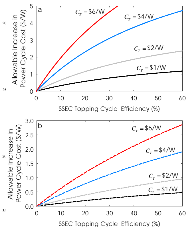
Fig. 5 Maximum Allowable Increase in Cost of a Power Cycle vs. Efficiency. a shows the maximum allowable increase in the cost/power ratio for a system where the SSEC rejects heat to a 40% efficient (i.e. steam Rankine) bottoming cycle. Each curve corresponds to a different CSP thermal system cost ranging from \$1\text{-}6/\text{W} . A combined SSEC/turbine power cycle with the corresponding SSEC efficiency shown on the horizontal axis can have a total cost/power ratio D , greater than the turbine itself D_1 , by any amount below the curve and will still reduce the overall system cost and LCOE. b shows the maximum allowable increase in combined power cycle cost, where the bottoming cycle is 60% efficient (i.e. a combined cycle Brayton and Rankine cycle in tandem).
