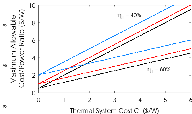
Fig. 6 Maximum Allowable Cost/Power Ratio D_{SSEC\_MAX} for a SSEC Topping Cycle vs. Thermal System Cost. The maximum allowable cost/power ratio for the SSEC device is given in Eq. 11 and is shown here for values of D_1 = \$0.5/\text{W} , \$1/\text{W} and \$2/\text{W} and turbine efficiencies of 40% (solid lines) and 60% (dashed lines). The corresponding value of D_1 for each line is given by the vertical axis intercept ( \$0.5/\text{W} , \$1/\text{W} , \$2/\text{W} ).
