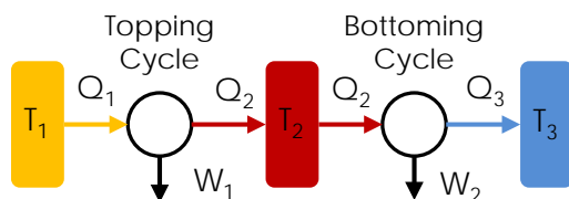
Fig. 3 Illustration of Tandem Heat Engine Configuration. The topping cycle is a high temperature heat engine, which rejects its waste heat to a
