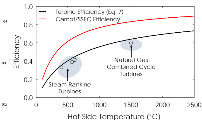
Fig. 2 Comparison of Estimated Maximum Efficiency for a Turbine and a Solid State Energy Conversion (SSEC) Device. The upper limiting efficiency for turbomachinery is lower than Carnot efficiency because it is based on a sensible heat input, while Carnot efficiency, which applies to SSEC devices, utilizes a constant temperature heat input.
