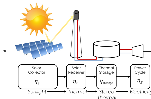
Fig. 1 Energy flow diagram for a concentrated solar power (CSP) plant
