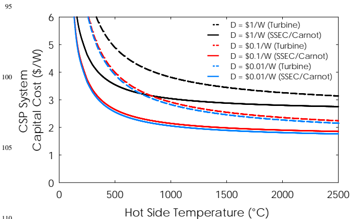
Fig. 4 CSP Capital Cost vs. Temperature. The capital cost is calculated using the following nominal values obtained from the SunShot vision study: 16 A = \$85/\text{m}^2 , S = 400 \text{ W}/\text{m}^2 , \eta_S \cdot \eta_T \cdot \eta_{storage} = 0.55 , F = 2.7 ,
