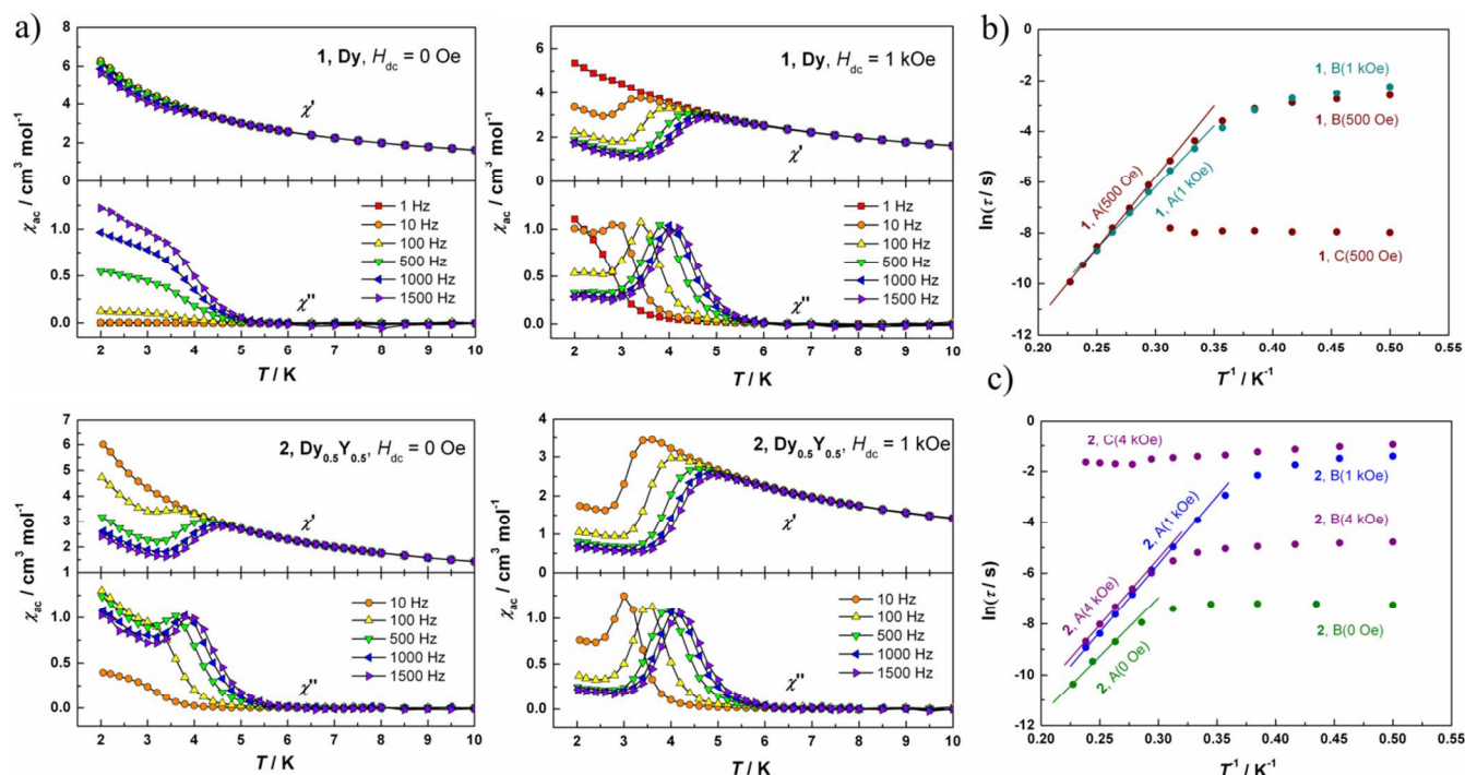
Fig. 3 a) Temperature dependence of the in-phase and out-of-phase ac susceptibility for 1 and 2 under 0 or 1 kOe dc field. b) Plots of \ln(\tau) vs. 1/T for 1 at H_{dc} = 500 \text{ Oe} and 1 \text{ kOe} . c) Plots of \ln(\tau) vs. 1/T for 2 at H_{dc} = 0, 1 \text{ kOe} and 4 \text{ kOe} . The solid lines represent Arrhenius fits of the frequency-dependent data.
