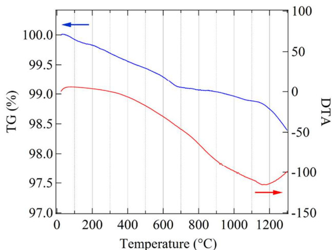
Fig. 2 TG and DTA curves for SrTaO 2 N in Ar flow.
