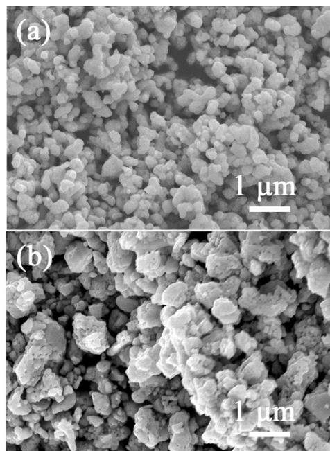
Fig. 1 SEM images of SrTaO 2 N powder produced by (a) direct synthesis at 950 °C in N 2 and by (b) SSR at 1000 °C in NH 3 . Reproduced with permission from ref. 14a. Copyright 2014 Elsevier.
