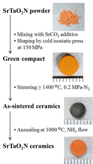
Fig. 3 Procedure of the pressureless sintering for SrTaO 2 N ceramics 9a,9c .
