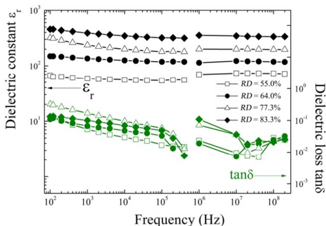
Fig. 4 Dielectric constant and dielectric loss versus frequency at room temperature for annealed SrTaO 2 N ceramics with various relative densities. Reproduced with permission from ref. 9c. Copyright 2014 John Wiley and Sons Ltd.
