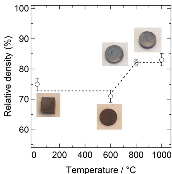
Fig. 5 Relative density of high-pressure SrTaO 2 N compacts as a function of the heating temperature when prepared under 7.7 GPa. Inset images show the colours of the compacts. Reproduced with permission from ref. 13. Copyright 2014 Elsevier.
