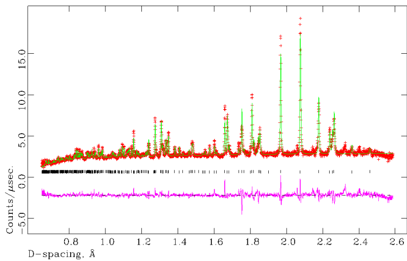
Figure 2. Rietveld fit (NPD) for single phase O-LaTaO 4 model at 100 °C. Overall \chi^2 = 6.67 for 37 refined variables.
