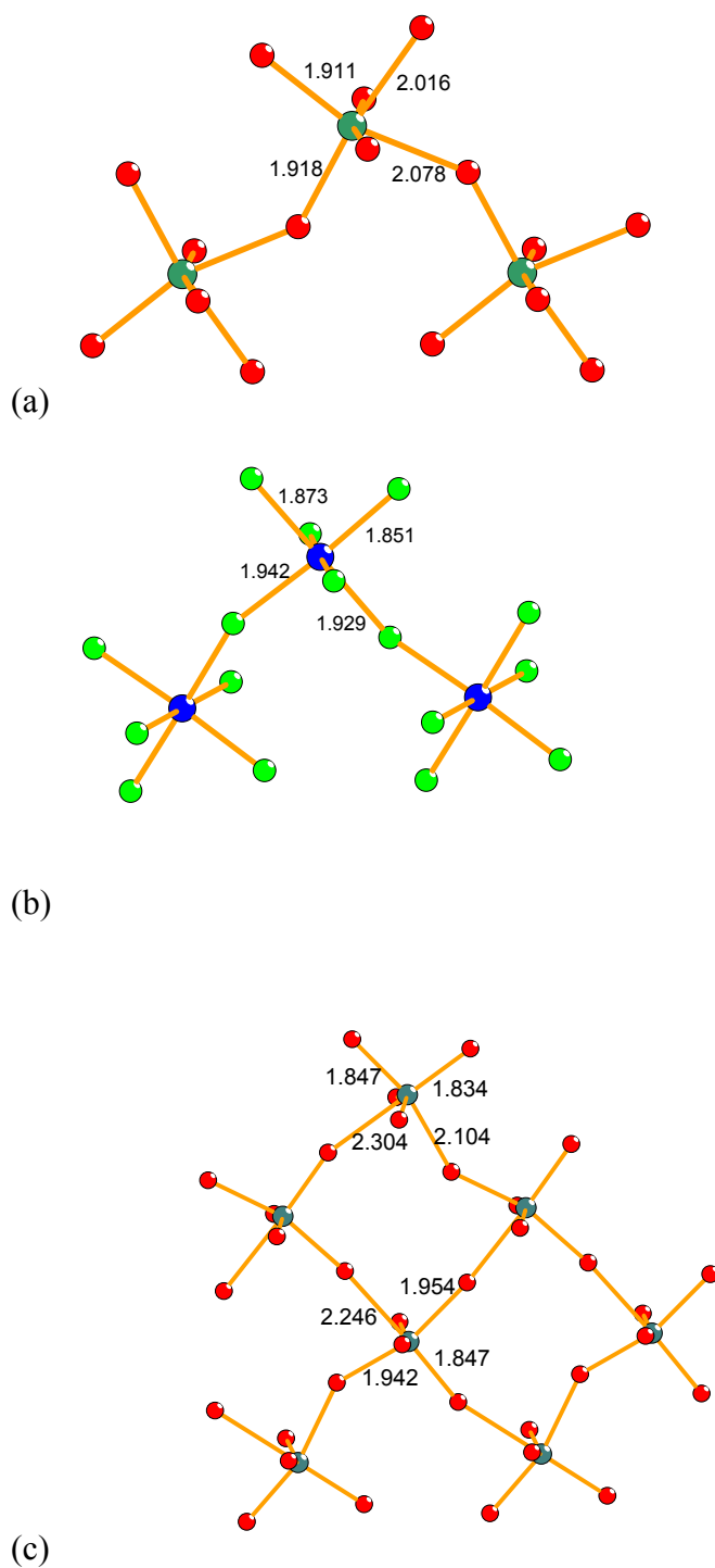
Figure 9. Nature of the octahedral distortions in selected members of the A_n B_n X_{3n+2} family: (a) O-LaTaO 4 at 100 °C (present study) (b) M-NaCrF 4 at 25 °C (ref. 23) (c) O-Sr 2 Nb 2 O 7 at 25 °C (ref. 24). Note that the latter contains two distinct octahedral sites.
