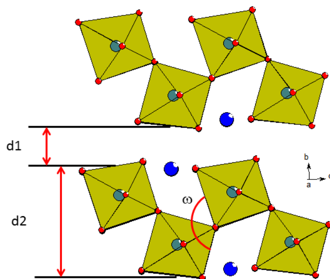
Figure 4. View of adjacent octahedral blocks in the O-LaTaO 4 structure, with the definitions of the parameters, d1 , d2 and \omega shown.
