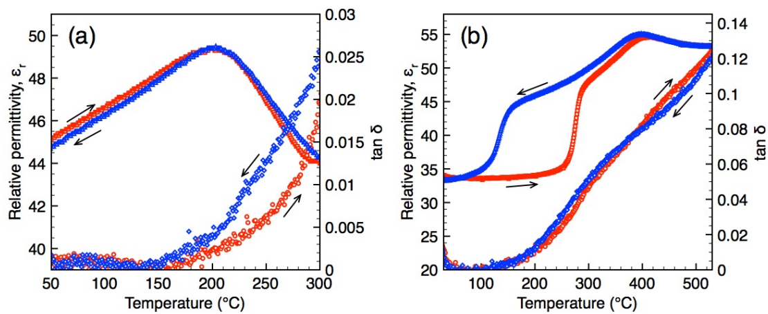
Figure 8. Dielectric data (obtained at 1 MHz) as a function of temperature for \text{LaTaO}_4 (a) and \text{La}_{0.90}\text{Nd}_{0.10}\text{TaO}_4 (b).
