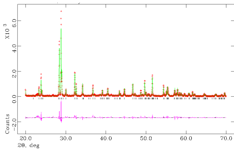
Figure 6. Rietveld fit (XPD) for \text{La}_{0.80}\text{Nd}_{0.20}\text{TaO}_4 (M-LaTaO 4 ) model at 25 °C. \chi^2 = 4.91 .
