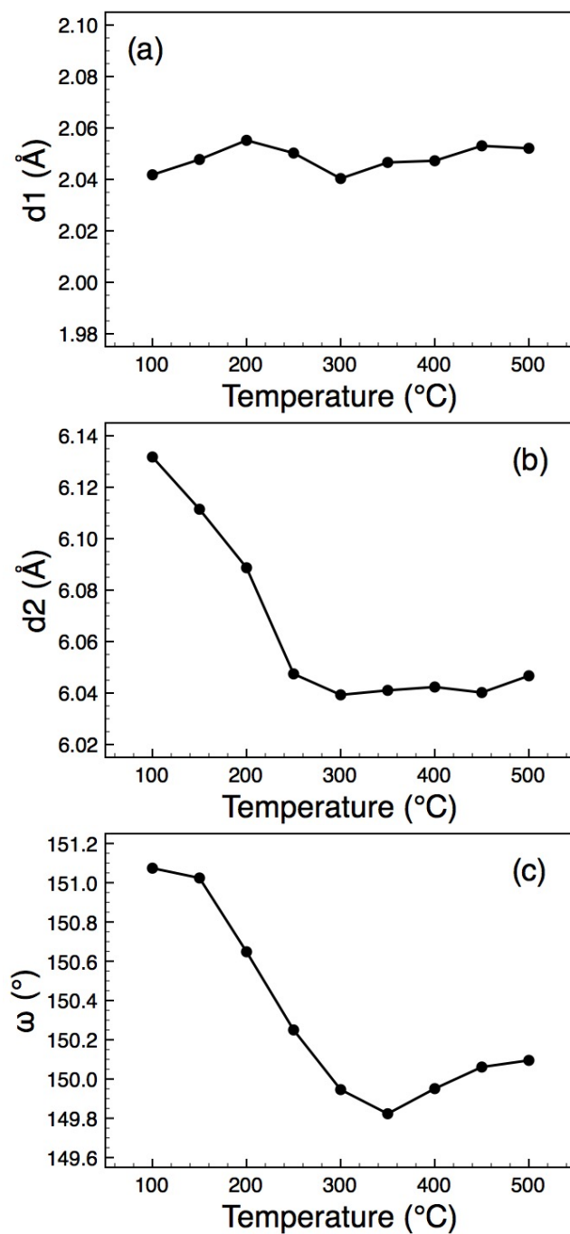
Figure 5. Thermal evolution of the distortion parameters (defined in Figure 4) for O-LaTaO 4 , (a) d1 , (b) d2 , (c) \omega .
