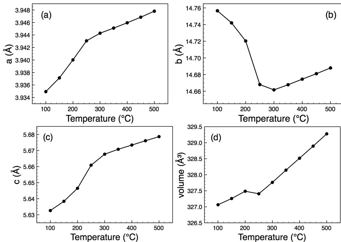
Figure 3. Thermal evolution of lattice parameters and unit cell volume for O-LaTaO 4 , derived from Rietveld refinement of NPD data.
