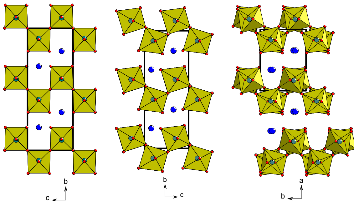
Figure 1. (a) Aristotype ABX_4 structure type, space group Cmc , with no octahedral tilting. (b) O-LaTaO 4 structure, space group Cmc2_1 : note that the c -axis polarity arises as a natural consequence of the ‘in-phase’ tilting around the a -axis. (c) M-LaTaO 4 structure, space group P2_1/c : in this case the ‘anti-phase’ tilting around c permits retention of centrosymmetry.
