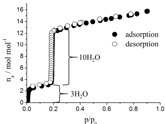
Fig. 6 Water sorption isotherm of CAU-14, measured at 298 K.
