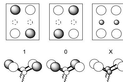
Fig. 6 The three Boolean states of a six-dot cell: 1, 0 and one null (X), depending on the charges localization (gray shading). The middle dots (dashed) have different ground-state energy: the null state is forced upon application of the clocking electric field. The cell is implemented by two paired molecules, each including three “quantum-dot” moieties such as 35 . Adapted from Ref. 57.
