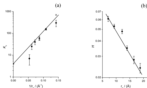
Fig. 2 (a) Comproportionation constant K_c (log scale) as a function of 1/r_g : (●) from redox titration; (×) from wave splitting. (b) Metal–metal coupling (log scale) H as a function of r_g in the hypothesis of a trans configuration of terminal ferrocene groups. Adapted with permission from Inorg. Chem. , 1996, 35 , 3735. Copyright 1996 American Chemical Society.
