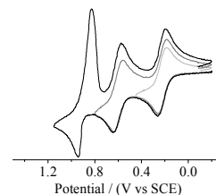
Fig. 8 CVs at different potential scan reversals of 72 in dichloromethane at Au disk electrode ( d = 0.5 mm), scan rate \nu = 0.5 V s -1 , T = 20 °C. Reprinted with permission from Angew. Chem., Int. Ed. , 2008, 47 , 5331. Copyright 2008 John Wiley & Sons, Inc.
