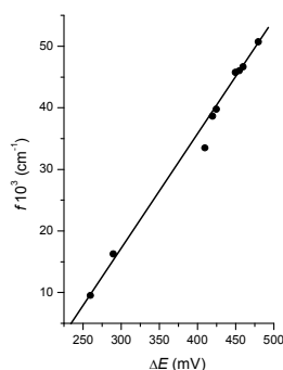
Fig. 4 Correlation of f with the \Delta E values of 16–24 ( R^2 = 0.987 ). Adapted with permission from Organometallics , 2013, 32 , 5640. Copyright 2013 American Chemical Society.
