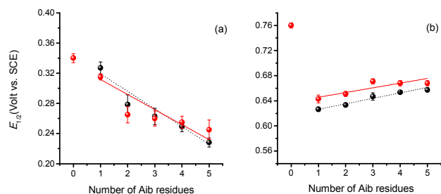
Fig. 5 E_{1/2} oxidation potentials of FcNHCOFc and 29–33 (red circles), and of Z-(Aib)_n-NH-Fc ( n = 1-5 ) (a, black circles) and Fc-CO-(Aib)_n-OMe ( n = 1-5 ) (b, black circles) peptides, obtained by CV in dichloromethane containing 0.1 M nBu_4NPF_6 as the supporting electrolyte; Au disk electrode ( d = 0.5 mm); scan rate 0.5 Vs^{-1} ; T 20 °C. Reprinted with permission from Biopolymers , 2013, 100 , 14. Copyright 2013 John Wiley & Sons, Inc.
