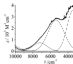
Fig. 9 NIR/IR spectrum of the 72 + cation in dichloromethane (straight line) and Gaussian deconvolution (dashed lines). Reprinted with permission from Angew. Chem., Int. Ed. , 2008, 47 , 5331. Copyright 2008 John Wiley & Sons, Inc.
