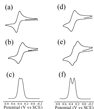
Fig. 3. Oxidative CVs in dichloromethane at 20 °C of 7a with (a) 0.1 M n Bu 4 NPF 6 , (b) 0.1 M n Bu 4 NB(C 6 F 5 ) 4 , (c) DPV with 0.1 M n Bu 4 NB(C 6 F 5 ) 4 . Oxidative CVs in dichloromethane of 7b with (d) 0.1 M n Bu 4 NPF 6 , (e) 0.1 M n Bu 4 NB(C 6 F 5 ) 4 , (f) DPV with 0.1 M n Bu 4 NB(C 6 F 5 ) 4 . Reprinted with permission from Organometallics , 2011, 30 , 1116. Copyright 2011 American Chemical Society.
