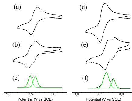
Fig. 7 Oxidative CVs in dichloromethane, scan rate \nu = 0.5 \text{ V s}^{-1} , of 53 with (a) 0.1 M n\text{Bu}_4\text{NPF}_6 , (b) 0.1 M n\text{Bu}_4\text{NB}(\text{C}_6\text{F}_5)_4 , (c) SWV with 0.1 M n\text{Bu}_4\text{NB}(\text{C}_6\text{F}_5)_4 . Oxidative CVs in dichloromethane of 54 with (d) 0.1 M n\text{Bu}_4\text{NPF}_6 , (e) 0.1 M n\text{Bu}_4\text{NB}(\text{C}_6\text{F}_5)_4 . (f) SWV with 0.1 M n\text{Bu}_4\text{NB}(\text{C}_6\text{F}_5)_4 . Reprinted with permission from Organometallics , 2013, 32 , 1029. Copyright 2013 American Chemical Society.
