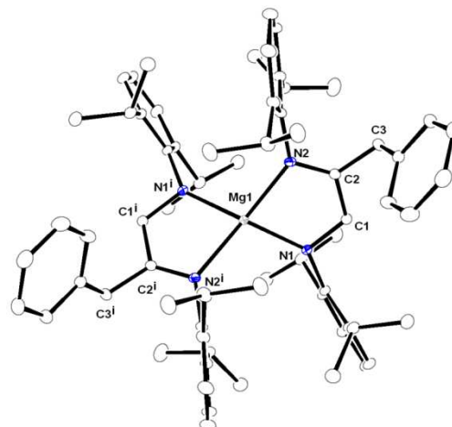
Figure 3. Solid-state structure of complex 4 and ellipsoids are drawn to encompass 30% probability. Hydrogen atoms are omitted for clarity. Selected bond lengths [Å] and bond angles[°]: Mg1–N1 2.0079(9), Mg1–N2 2.2079(10), Mg1–N1 i 2.0079(9), Mg1–N2 i 2.2079(10), N1–C1 1.4422(12), N2–C2 1.2915(13), C1–C2 1.4919(13), C2–C3 1.5151(14), N1–Mg1–N2 81.54(3), N1–Mg1–N1 i 153.44(6), N1–Mg1–N2 i 107.39(3), N1 i –Mg1–N2 i 81.54(3), N1 i –Mg1–N2 107.39(3), N2 i –Mg1–N2 141.43(5), C22–N1–Mg1 139.13(6), C1–N1–Mg1 112.82(6), C2–N2–Mg1 110.08(6), C10–N2–Mg1 133.34(6), C22–N1–C1 107.73(7), N2–C2–C1 119.23(9), C2–N2–C10 116.50(8), N2–C2–C3 125.66(9).
