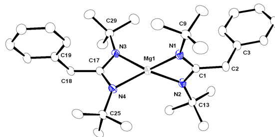
Figure 2. Solid-state structure of complex 3 and ellipsoids are drawn to encompass 30% probability. Hydrogen atoms are omitted for clarity. Selected bond lengths [Å] and bond angles[°]: Mg1–N1 2.052(4), Mg1–N2 2.044(4), Mg1–N3 2.055(4), Mg1–N4 2.044(3), N1–C1 1.347(5), N2–C1 1.349(5), N3–C17 1.334(5), N4–C17 1.345(5), C1–C2 1.523(5), C17–C18 1.519(5), N2–Mg1–N1 65.96(14), N4–Mg1–N3 65.73(14), N4–Mg1–N1 137.35(15), N4–Mg1–N2 134.18(15), N2–Mg1–N3 136.22(15), N1–Mg1–N3 131.51(15), C1–N1–Mg1 91.1(2), C1–N2–Mg1 91.4(2), C17–N3–Mg1 90.9(2), C17–N4–Mg1 91.1(2), N1–C1–N2 111.5(3), N1–C1–C2 124.1(4), N2–C1–C2 124.3(4), N3–C17–N4 112.2(3), N3–C17–C18 124.5(4), N4–C17–C18 123.1(3).
