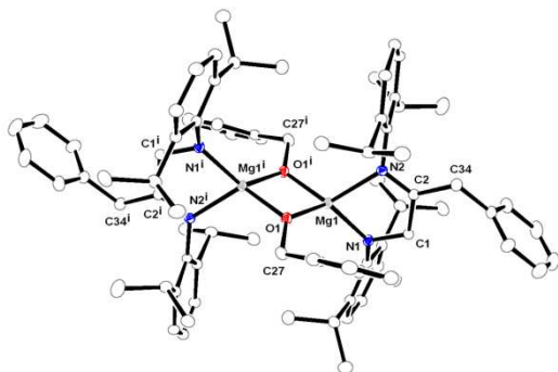
Figure 6. Solid-state structure of complex 7 and ellipsoids are drawn to encompass 30%. Hydrogen atoms are omitted for clarity. Selected bond lengths [Å] and bond angles[°]: Mg1–O1 1.9560(16), Mg1–O1 i 1.9602(17), O1–Mg1 i 1.9602(17), Mg1–N1 1.9788(19), Mg1–N2 2.1452(19), N1–C1 1.438(3), N2–C2 1.291(3), O1–C27 1.413(3), C1–C2 1.506(3), C(2)–C(34) 1.513(3), O(1)–C(27) 1.413(3), O1–Mg1–O1 i 84.53(7), O1–Mg1–N1 124.62(8), O1–Mg1–N1 i 133.37(8), O1–Mg1–N2 117.76(7), O1 i –Mg1–N2 117.70(7), N1–Mg1–N2 82.73(7), C1–N1–Mg1 111.17(13), C2–N2–Mg1 109.45(14), C27–O1–Mg1 134.31(14), C27–O1–Mg1 i 126.09(13), Mg1–O1–Mg1 i 95.47(7), N1–C1–C2 114.70(17), N2–C2–C1 118.47(18), N2–C2–C34 123.29(19), C1–C2–C34 118.23(18).
