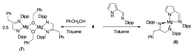
Scheme 5. Syntheses of magnesium complexes 6 and 7 .
