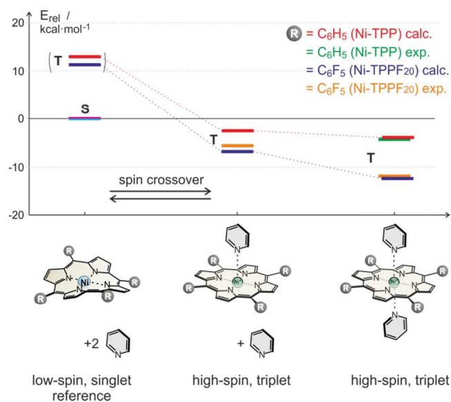
Figure 5. Calculated (B3LYP/def2TZVP//PBE/DZP) and experimental relative association energies (kcal mol -1 ) of pyridine to Ni-TPP (calc. red, exp. green) and Ni-TPPF 20 (calc. blue, exp. yellow) for the respective triplet (high-spin) complexes. The energies are relative to the corresponding porphyrin in its low-spin singlet state (including two unbound pyridine molecules). Note that the experimental 22 and calculated association energies agree quite well. The (very small) experimental binding enthalpy for the 1:1 complex of the Ni-tetraphenylporphyrin with pyridine could not be determined.
