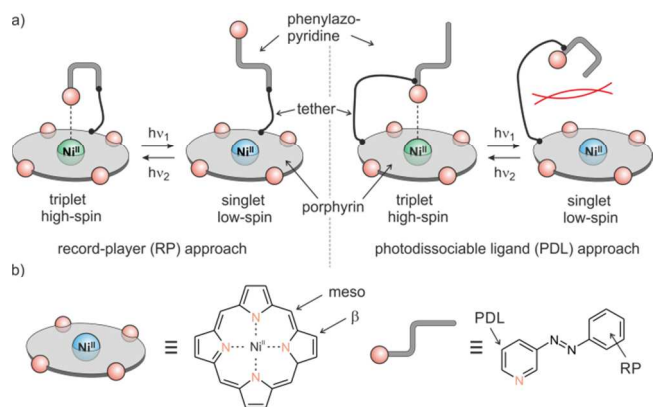
Figure 2. a) General design approaches (record player (RP), left), photodissociable ligand (PDL) right. b) Positions of tether attachment.
