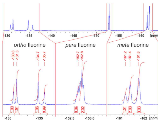
Figure 14. ^{19}\text{F} -NMR spectra of cis-2 (500 MHz, dichloromethane, 300 K).
