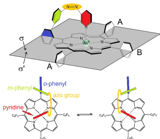
Figure 15. Top: Record player cis-2 para has two symmetry non-equivalent sides \sigma and \sigma' . Neither of the meso substituents (pentafluorophenyl and “tone arm”) rotate around the porphyrin plane on the NMR time scale at 300 K. For the sake of clarity the fluorine atoms at the meso positions A and B are omitted. Bottom: Top view on the conversion between the two enantiomers of cis-2 . The conformational equilibrium is fast on the NMR time scale at 300 K.
