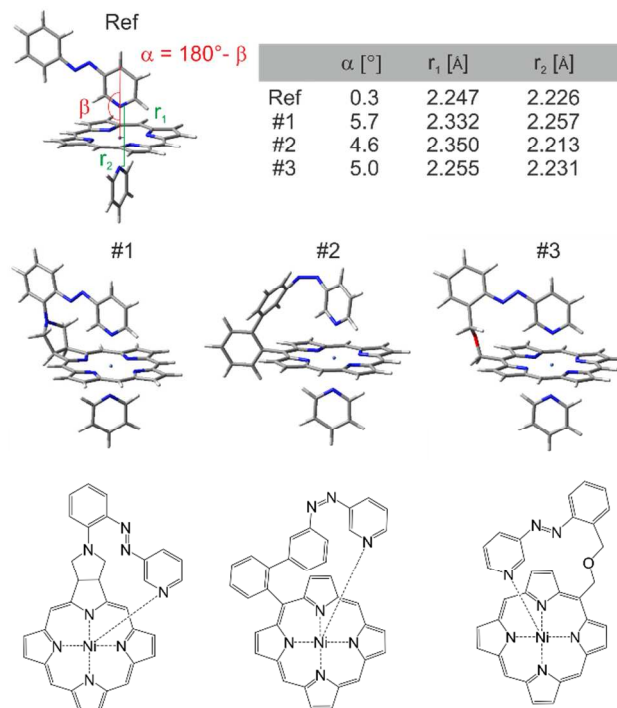
Figure 3. Geometry plots (B3LYP/6-31G*) and structures of Ni-porphyrin with 3-phenyl-azopyridine and pyridine as axial ligands. The reference compound (Ref) without tether is given on top left. and the three highest ranking “record player” structures for LD-CISSS are represented underneath. Note that structure #1 and #3 bind in trans configuration and #2 coordinates in its cis form. Pyridine has been included in the calculations as a second axial ligand because it is known that Ni-porphyrins prefer a 6-coordinate ligand field. It is assumed that upon changing the coordination number from 4 to 5 and concomitant switching from low-spin to high-spin a solvent molecule would coordinate to complete the square bipyramidal ligand field:
