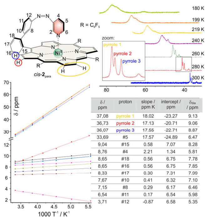
Figure 13. Temperature dependence of chemical shifts of cis-2 in ^1\text{H} NMR spectra (500 MHz, dichloromethane- d_2 ). Shifts of the pyrrole protons as a function of temperature are shown top right. The table bottom right shows the chemical shifts of all protons (except those of ortho pyridine #2 and #6) at 300 K ( \delta ), the slopes and intercepts of the corresponding Curie plots (bottom left) and the diamagnetic shifts of the corresponding zinc derivative ( \delta_{\text{dia}} ). 18
