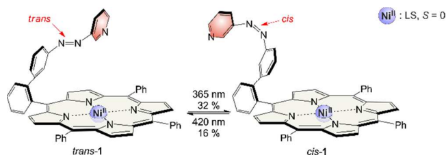
Figure 4. Record player #2 with phenyl groups in meso position ( 1 ) does not switch efficiently upon irradiation. The photostationary state (PSS) upon irradiation at 365 nm is 32% cis and at 420 nm 16% cis . Even though the geometry of the cis isomer is optimal for coordination, the “tone arm” doesn’t bind to the Ni 2+ .
