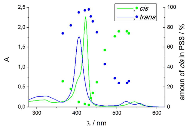
Figure 6. UV/Vis spectra of trans and cis record player 2 (blue and green line) and the photo steady states (blue and green points) after irradiation with the corresponding wavelength in dimethylsulfoxide (DMSO). The isomers were separated by HPLC.
