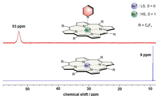
Figure 9. 1 H NMR spectra of Ni-TPPF 20 with (red) and without (blue) pyridine (500 MHz, acetonitrile, 300 K).
