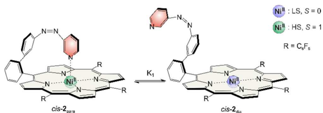
Figure 12. Equilibrium of the magnetic conformers cis-2 para (left) and cis-2 dia (right).
