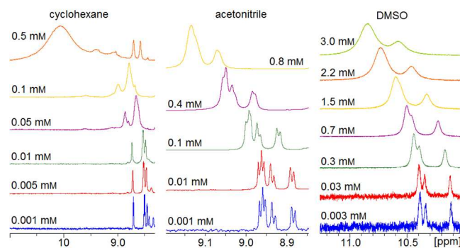
Figure 10. 1 H NMR spectra of record player 2 in trans configuration in different solvents (500 MHz, 300 K). The downfield shift and signal broadening indicates intermolecular coordination.
