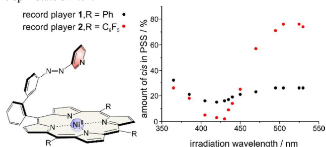
Figure 7. Switching properties of meso phenyl ( 1 ) and meso pentafluorophenyl ( 2 ) substituted record players.
