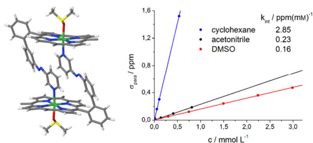
Figure 11. Crystal structure of trans-2 shows formation of dimers and a sixfold coordination sphere of Ni 2+ complemented by one axial DMSO molecule (left). The pentafluorophenyl groups at the porphyrin rings are omitted for clarity. For details see supporting information Figure S4. The linear correlation between paramagnetic shift of pyrrole signals ( \delta_{\text{para}} ) and concentration of trans-2 (right) confirms that there is also intermolecular coordination in solution.
