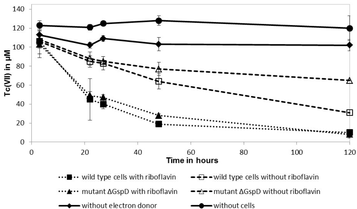
Fig. 2. Tc(VII) reduction kinetics, with and without added riboflavin, by wild type S. oneidensis MR-1 cells and a mutant with an in-frame deletion of gspD ( \Delta\text{gspD} ). 10 mM sodium lactate was supplied as the sole electron donor to pre-grown cells. Controls had no cells or no electron donor included.
