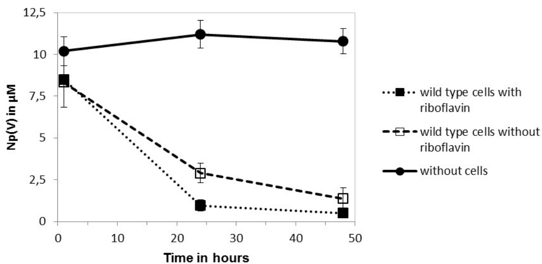
Fig. 3. Np(V) reduction kinetics with and without added riboflavin ( 10 \mu\text{M} ) by wild type cells of S. oneidensis MR-1 in the presence of 10 mM sodium lactate as the sole electron donor. Controls had no cells included.
