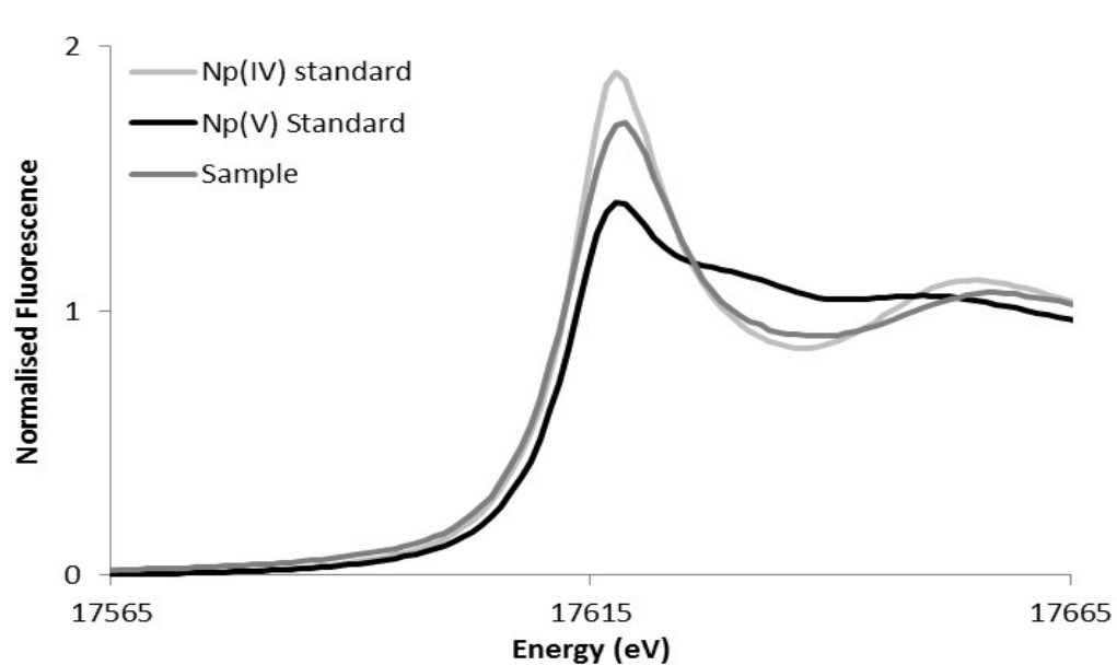
Fig. 4. Neptunium LIII-edge XANES spectra collected from the 50 \mu\text{M} Np experiment alongside pure oxidation state Np(V) and Np(IV) standards from the AcReDaS database 29,30 .
