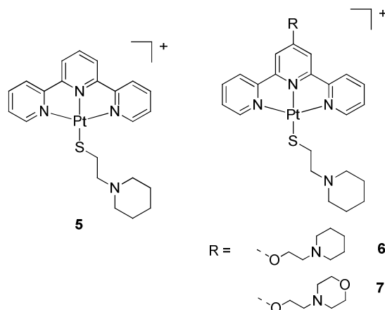
Fig. 3 Chemical structures of the platinum(II)-thiolate complexes 5-7. The counterion for complex 5 is \text{Cl}^- , while for 6 and 7 is \text{PF}_6^- .
