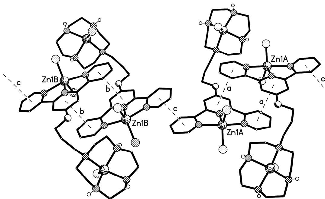
Fig. 9 Part of one of the \pi - \pi linked chains of cations present in the crystal of 8 . The \pi - \pi stacking interactions have centroid...centroid and mean interplanar separations ( \text{\AA} ) of a) 3.72, 3.33, b) 3.56, 3.42 and c) 3.65, 3.39 respectively.
