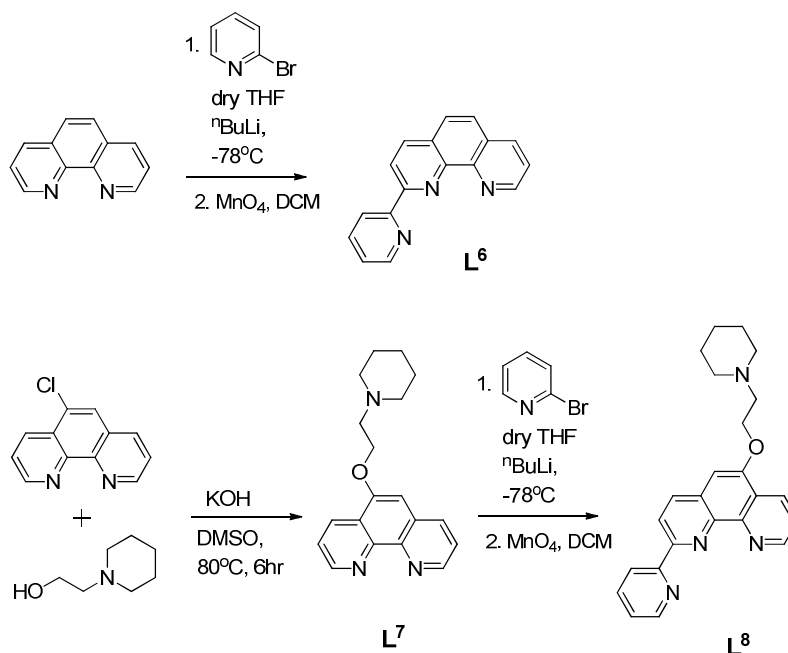
Scheme 2 Reaction schemes for the syntheses of ligands L 6 – L 8
