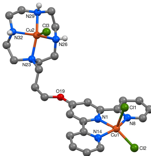
Fig. 10 The structure of the cationic complex present in the crystal of 9 .
