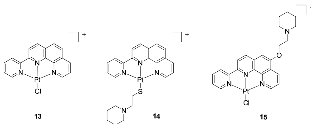
Fig. 5 Chemical structures of the platinum(II)-phenanthroline complexes 13-15 . The counterion for complex 13 is Cl - , while for 14 and 15 is PF 6 - .
