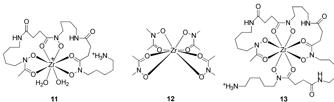
Figure 5: Left: Modelled coordination of Zr^{4+} by DFO ( 11 ); 20 Centre: Schematic structure of ZrL_4 ( HL = N -methylacetohydroxamic acid) ( 12 ), serving as a template for the design of new octadentate chelators for Zr^{4+} (note that disorder in the C and N orientations of the hydroxamate rings precludes determination of their preferred relative orientation and suggests that any such preferences are weak); 22 Right: Schematic structure of Zr^{4+} complex 13 of an octadentate DFO homologue. 23
