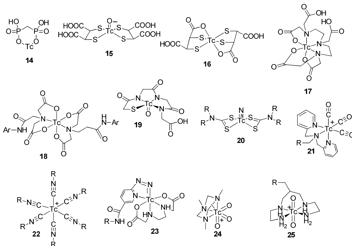
Figure 8: A selection of established ^{99\text{m}}\text{Tc} radiopharmaceuticals and core structures (if known): TcMDP ( 14 ), Tc(V)DMSA ( 15 ), TcDMSA ( 16 ), TcDTPA ( 17 ), TcHIDA ( 18 ) TcMAG3 ( 19 ), Tc(V)-nitridobis(dithiocarbamate) ( 20 ), Tc(I)-tricarbonyl ( 21 ), Tc(I)-hexakis(isonitrile) ( 22 ), Tc(V)-hynic ( 23 ), Tc(VII)-trioxo ( 24 ), and Tc(V)-dioxo ( 25 ). Structures of 15 , 19 , 20 , 21 , 22 , 24 and 25 are known and well defined; the others are not clearly defined.
