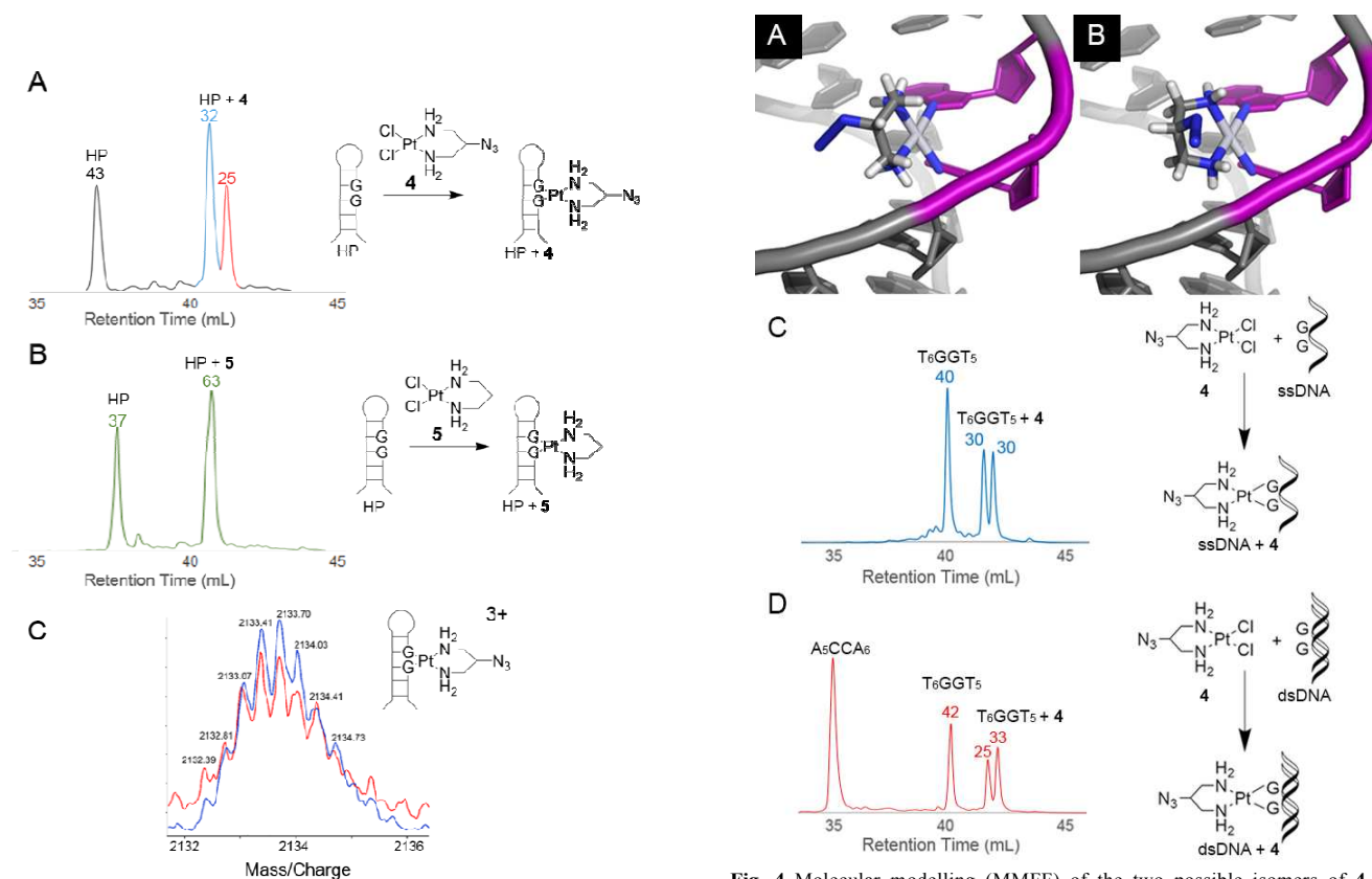
Fig. 3 HPLC absorbance traces at 260 nm for a short hairpin DNA sequence bound to (A) 4 and (B) 5. Peaks observed at ~37 mL eluent volume are identified as unbound DNA, and peaks between ~40 and ~42 mL are DNA-bound Pt (55–65% yield). When 4 is bound to DNA, two peaks are resolved indicating the presence of non-equivalent Pt-bound species. Reaction with azide-free 5 yields a single product band (B, 55–65% yield). Normalized areas are indicated above peaks of interest. Fractions were analysed via ESI-MS revealing both blue and red traces produce a peak correlating to the 3+ charged species of DNA bound by 4 (C).
