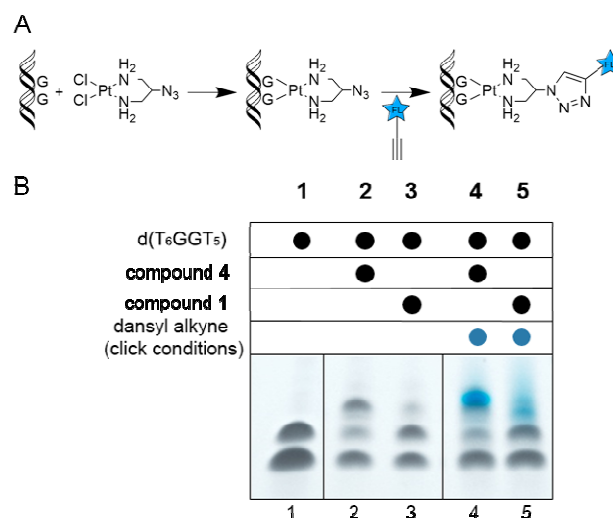
Fig. 2 (A) Reaction scheme for Pt binding and subsequent click to an alkyne fluorophore. (B) dPAGE analysis of dsDNA bound by picazoplatin ( 1 ) and cis -[Pt(2-azido-1,3-propanediamine)Cl 2 ] ( 4 ) and subsequently clicked to a dansyl alkyne fluorophore. The denatured DNA strands are visible in lane 1, while higher molecular weight Pt-bound species are visible in lanes 2 and 3. Click reaction results in fluorescence of the Pt-DNA band under UV light in lanes 4 and 5 (see ESI).
