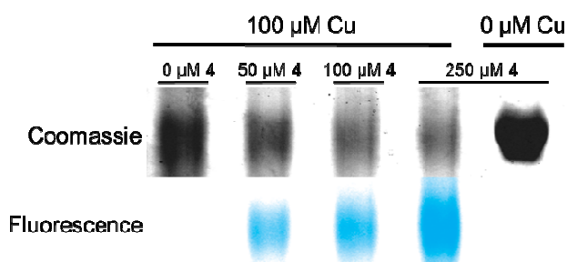
Fig. 5 Fluorescent labelling by click chemistry of 4 -treated bovine serum albumin (BSA) with a dansyl alkyne fluorophore. Lanes 2–4 contain BSA incubated in the presence of CuSO 4 post Pt treatment and show a dose-dependent increase in fluorescent signal with respect to the concentration of 4 . Lanes 1 and 5 shows that fluorescent labelling is also dependent on the presence of both 4 and the Cu catalyst.
