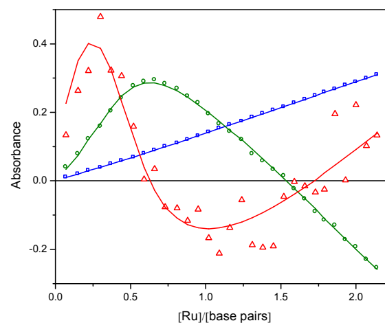
Fig. 7 The V -vectors corresponding to the first three singular values ( s_1 blue squares, s_2 green circles, s_3 red triangles) from the titration of Ru-tpy to a constant concentration of AT-DNA in 150 mM NaCl at 25°C. The fit of the model is shown as solid curves.
