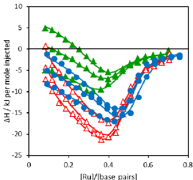
Fig. 5 ITC profiles with fitted traces for the binding of Ru-tpy (●), \Delta Ru-bpy (▲), and \Lambda Ru-bpy (△) to AT-DNA in 150 mM aqueous solution at 20, 25, and 30°C. Symbols indicate the normalized heat absorbed or evolved upon sequential injections (2 \mu\text{L} ) of complex into the 206 \mu\text{L} cell containing the DNA. The data has been corrected for heat of complex dilution. The corresponding ITC-profiles for \Delta - and \Lambda Ru-bpy are from Andersson et al. (2013). 10
