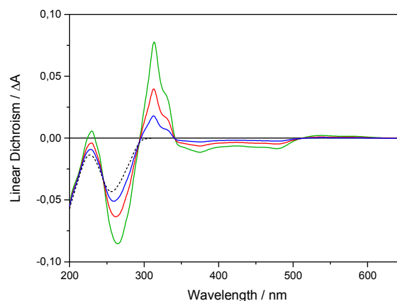
Fig. 3 Linear dichroism spectra of Ru-tpy in the presence of ctDNA at [base pairs] / [Ru] ratios 8 (blue), 4 (red) and 2 (green) in 10 mM NaCl solution, as well ctDNA alone (dotted). The concentration of ctDNA is 270 \mu M nucleotides.
