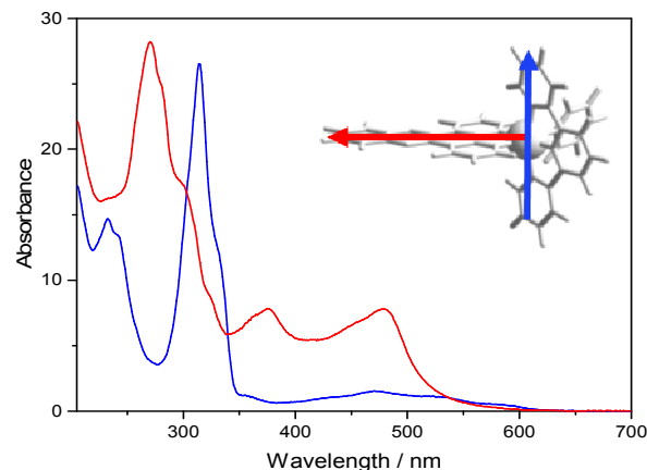
Fig. 4 Resolved spectra of the x and y (red) and the z (blue) polarized absorption bands of Ru-tpy bound to ctDNA. The Y-axis units are
