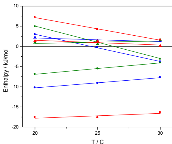
Fig. 9 The standard binding enthalpy \Delta H^\circ_b (■), standard nearest neighbor interaction enthalpy \Delta H^\circ_{nm} (●), and \Delta H^\circ_{baseline} (▲) for binding of Ru-tpy (blue), \Delta Ru-bpy (green), and \Lambda Ru-bpy (red) to AT-DNA in 150 mM NaCl. The slopes of the fitted lines correspond to the \Delta C_p for the reactions.
