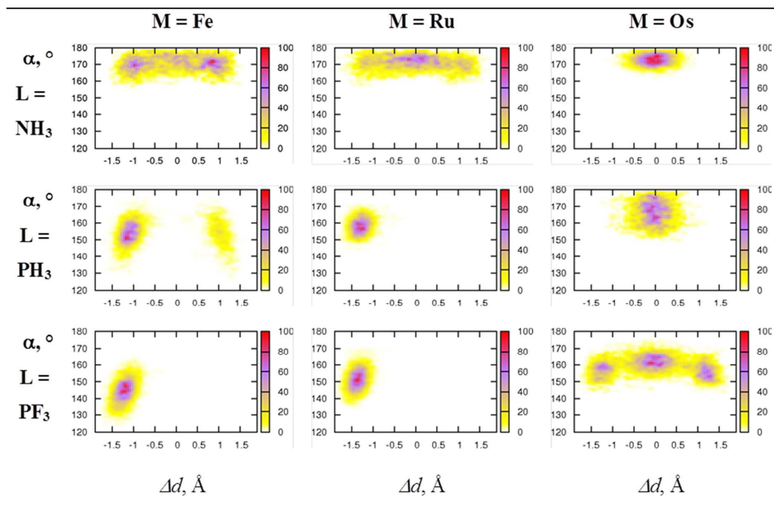
Figure 2: Correlation frequency maps between the angle L_{\text{axial}}\text{-M-L}_{\text{axial}} ( \alpha ) and d(\text{H}_1\cdots\text{H}_2) - d(\text{H}_3\cdots\text{H}_4) ( \Delta d ) for complexes \text{MH}_4(\text{L})_3 .
