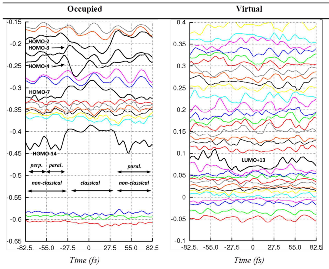
Figure 4: Time evolution of the eigenvalues (in Hartree) of the molecular orbitals in [\text{FeH}_4(\text{PH}_3)_3] during the scrambling process. “ perp. ” and “ paral. ” denote a perpendicular ( \phi = 90^\circ ) and parallel ( \phi = 0^\circ ) orientation of the \text{H}_2 ligand. Since HOMO-3 and HOMO-4 cross during the rotation of \text{H}_2 (at t = -55 fs), we labelled the molecular orbitals according to their order from t > 55 fs.
