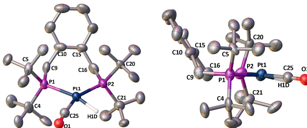
Figure 3. Crystal structure of [Pt(L_a)(H)(CO)][B(C_6F_5)_4] ( 5a ). The view on the right shows the chelate ring conformation. Only one of the two Pt-containing moieties in the asymmetric unit is shown and only one position of the disordered CO/H combination. For clarity all of the hydrogen atoms (apart from the hydride H1D) are omitted along with the [B(C_6F_5)_4]
