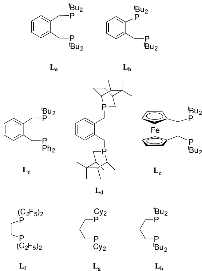
Chart 1. Structures of ligands discussed.
