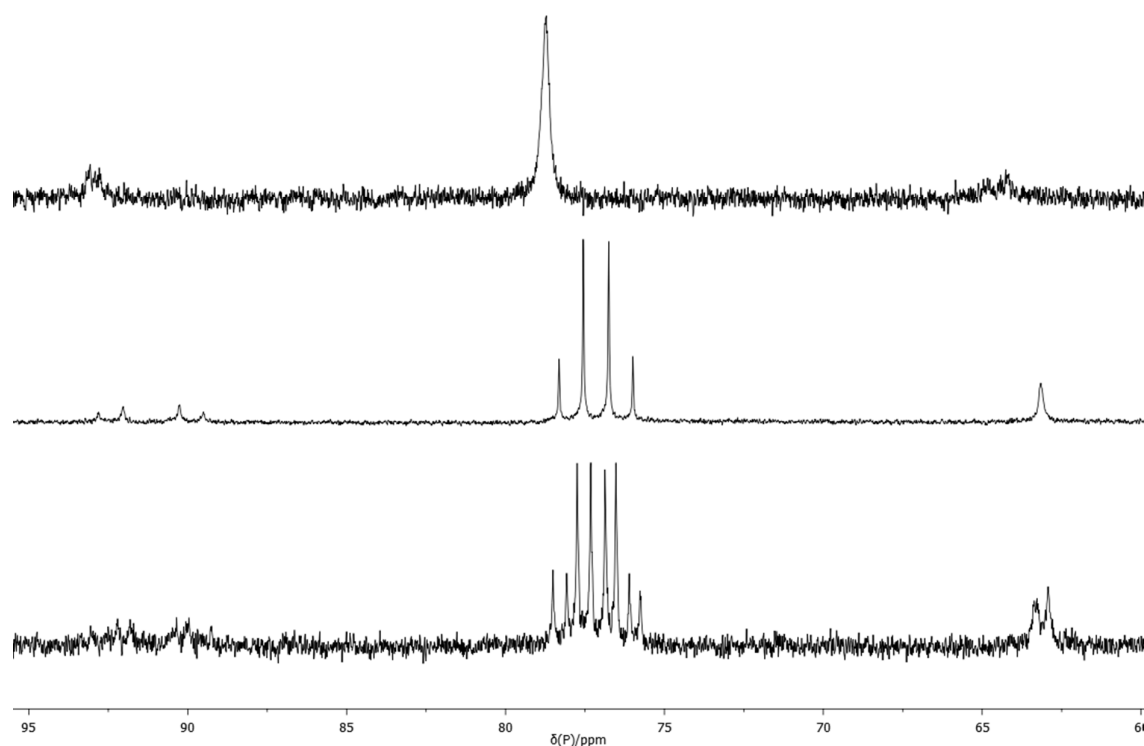
Figure 1. Variable temperature ^{31}\text{P} NMR spectra: top, 2b , room temperature; middle, 2b , -90\text{ }^\circ\text{C} ; bottom, 2b *, -90\text{ }^\circ\text{C} .
