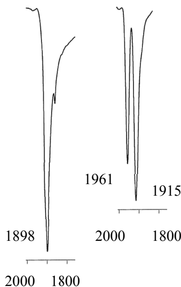
Figure 2. Solid state IR spectra in the \nu(\text{CO}) region for monocarbonyl 2b (left) and dicarbonyl 3b (right).
