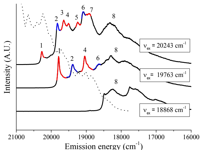
Fig. 4. Selected LLN spectra of \text{UO}_2^{2+} sorbed on a C-S-H phase (C:S = 1.07) in ACW at pH = 13.3 recorded at three different excitation energies ( \nu_{\text{ex}} = 20'243\text{ cm}^{-1} , 19'763\text{ cm}^{-1} , and 18'868\text{ cm}^{-1} ). Delay time = 10 \mu\text{s} . Gate width = 10 ms. The numbered transition lines are described in the text and in Table 1. Red = lines assigned to species U1, blue = lines assigned to species U2
