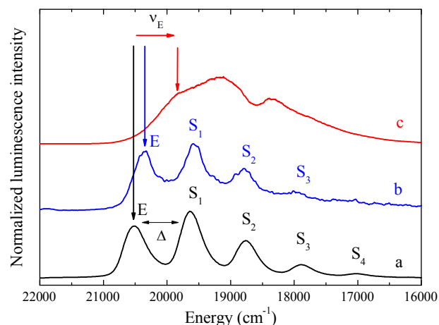
Fig. 2. Non-selective luminescence spectra recorded at 15 K of a) 10^{-5} \text{ M UO}_2^{2+} in 0.1 M \text{HNO}_3 , \text{pH} \sim 1.0 , b) 10^{-5} \text{ M UO}_2^{2+} in 0.5 M TMAOH, \text{pH} = 13.5 , c) \text{UO}_2^{2+} sorbed onto C-S-H phases (C:S = 1.07, in ACW at \text{pH} = 13.3 ); loading = 10^{-3} \text{ mol kg}^{-1} . \nu_{\text{ex}} = 24'390 \text{ cm}^{-1} . Delay time = 10 \mu\text{s} , gate width = 1.0 ms.
