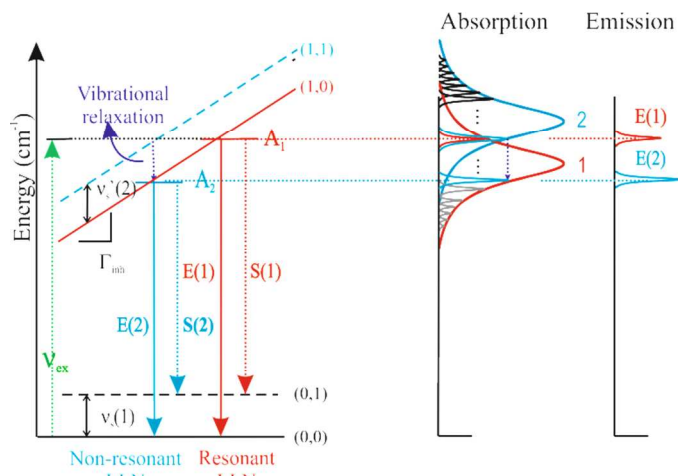
Fig. 1. Energy-level diagram illustrating resonant ALN E(1) and non-resonant LLN E(2) after site-selective laser excitation at an energy, ν ex (diagram adapted from Jankowiak 35 ). See text for a detailed explanation
