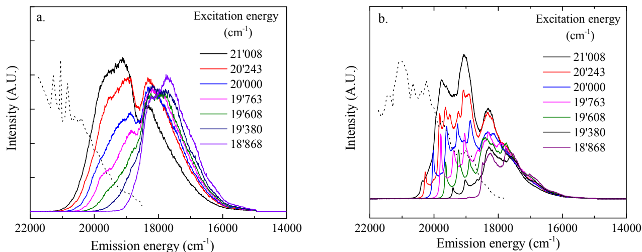
Fig. 3: Excitation spectra (dotted lines) and selected LLN spectra of \text{UO}_2^{2+} sorbed on a C-S-H phase (C:S = 1.07) in ACW at pH = 13.3. \text{UO}_2^{2+} loading = 10^{-3} \text{ mol kg}^{-1} . Excitation energy: 21'008 \text{ cm}^{-1} < \nu_{\text{ex}} < 18'868 \text{ cm}^{-1} . Delay time = 10 \mu\text{s} . Gate width = 10 \mu\text{s} (a) and 10 \text{ms} (b). The intensities of the excitation spectra in Fig. 3a. and 3b. are divided by a factor 50 and 40, respectively.
