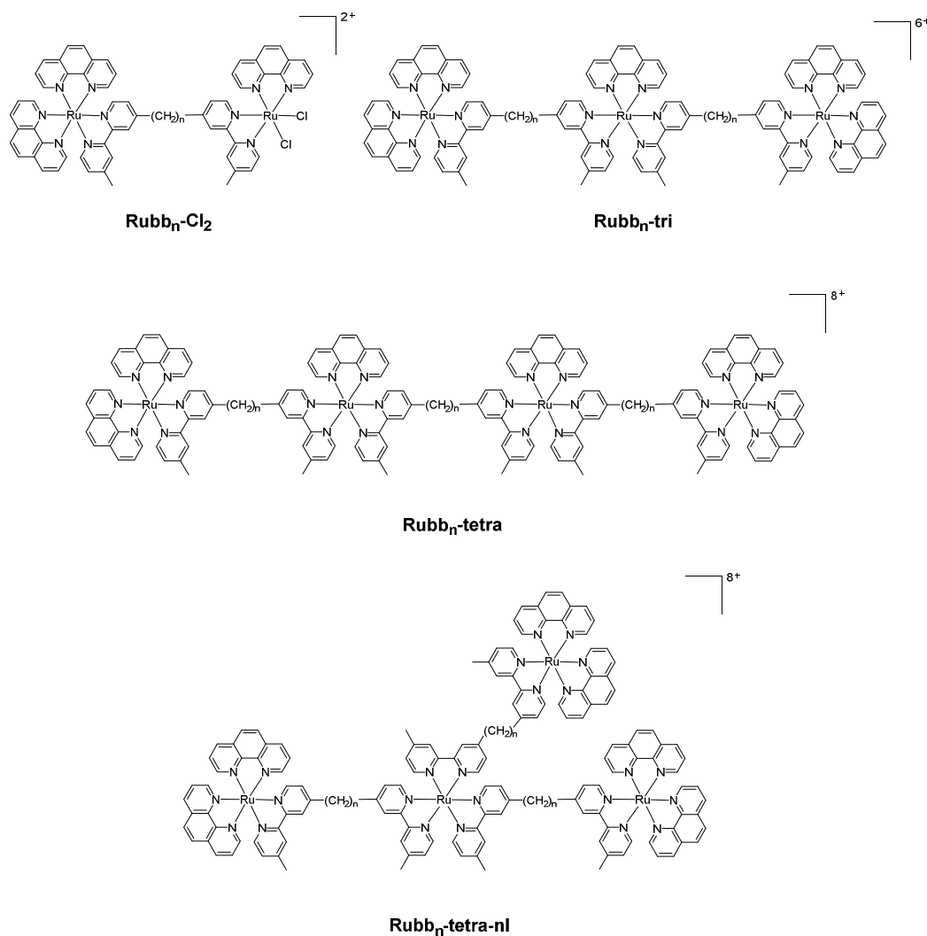
Figure 1. Chlorido-containing dinuclear complexes ( \text{Rubb}_n\text{-Cl}_2 ); and the inert trinuclear ( \text{Rubb}_n\text{-tri} ) and tetranuclear (linear \text{Rubb}_n\text{-tetra} , and non-linear \text{Rubb}_n\text{-tetra-nl} ) ruthenium(II) complexes
