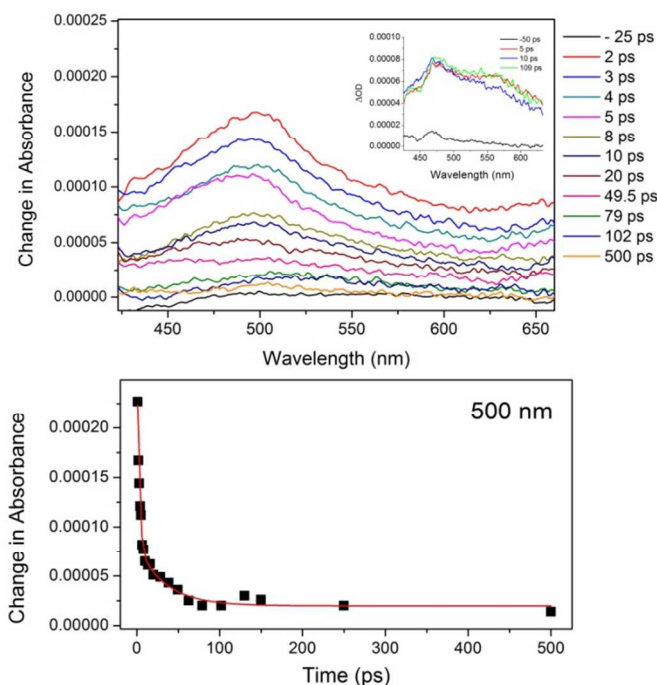
Fig. 2 (a) ps-TA of 800 μM rac -[Cr(phen) 2 dppz] 3+ in presence of 2 mM [d(GCGCGCGCGC)] in 50mM phosphate buffer solution, pH = 7.4. Inset: ps-TA for 400 nm excitation rac -[Cr(phen) 2 dppz] 3+ in D 2 O. (b) Biexponential fit for the loss of absorbance at 500 nm. Excitation at 400 nm, 1 μJ.
