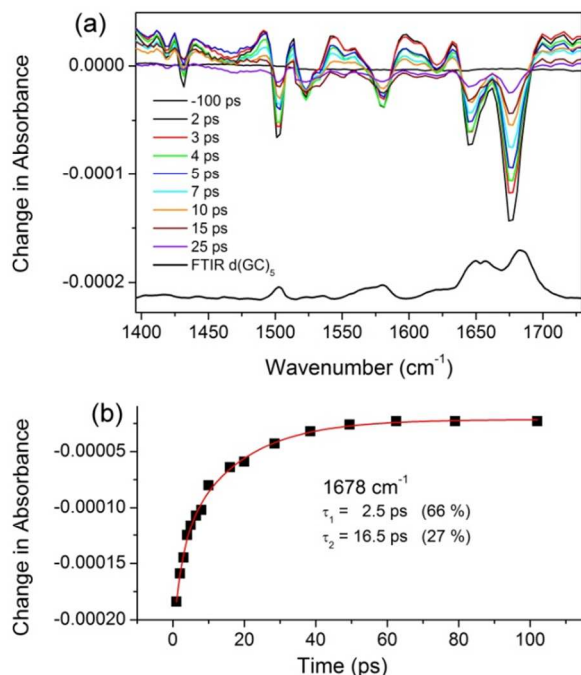
Fig. 3 (a) ps-TRIR of 400 \mu\text{M} \text{rac}[\text{Cr}(\text{phen})_2(\text{dppz})]^{3+} in presence of 2 mM d(GCGCGCGCGCGC) in 50mM phosphate buffer solution, pH=7.4. (b) Biexponential fit for the recovery of the guanine at 1678 \text{cm}^{-1} . Excitation at 400 nm, 1 \mu\text{J} .
