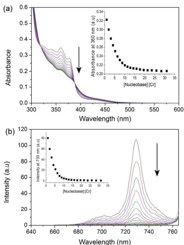
Fig. 1 (a) UV-visible absorption spectra of rac -[Cr(phen) 2 dppz] 3+ (24 μM in 50 mM phosphate buffer solution, pH = 7.4) in the presence of increasing concentrations of [d(GCGCGCGCGC)]. Inset: Change in absorbance at 360 nm. (b) The corresponding phosphorescence spectra ( \lambda_{\text{ex}} = 388 nm). Inset: Change in the emission at 730 nm.
