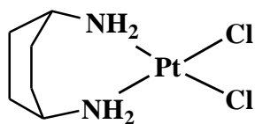
[PtCl 2 ( cis -1,4-DACH)] (Kiteplatin)
