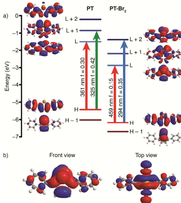
Fig. 1 a) Excited state transitions of PT and PT-Br 2 with oscillator strength greater than 0.1 as predicted by TD-DFT, and their associated MOs (isocontour value of 0.02; H refers to HOMO, L refers to LUMO). b) Front and top view of the calculated LUMO for PT-Br 2 .
