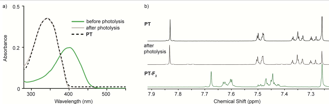
Fig. 4 a) Photolysis of PT-F 2 with 447.5 nm light over time monitored by a) optical absorption spectroscopy and b) 1 H NMR spectroscopy.
