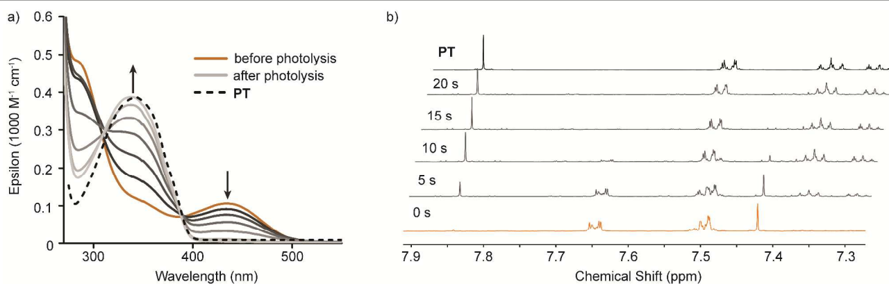
Fig. 3 a) Photolysis of PT-Br 2 with 447.5 nm light over time monitored by a) optical absorption spectroscopy and b) 1 H NMR spectroscopy.
