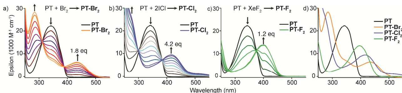
Fig. 2 Optical absorption titration experiments. a) Br 2 titration; b) ICl titration; c) XeF 2 titration; d) Comparison of absorption spectra of PT and its halogenated adducts.
