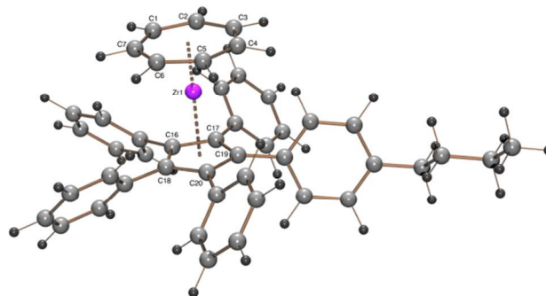
Figure 8. ORTEP plot of the calculated structure of 9 . Calculated bond length (Å) and angles (°): Zr–C1 2.345, Zr–C2 2.351, Zr–C3 2.348, Zr–C4 2.346, Zr–C5 2.349, Zr–C6 2.347, Zr–C7 2.342, Zr–C16 2.541, Zr–C17 2.542, Zr–C18 2.544, Zr–C19 2.542, Zr–C20 2.541, Zr–Cp cent 2.233, Zr–CHT cent 1.679, CHT cent –Zr–Cp cent 179.43.
