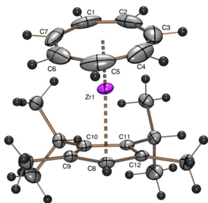
Figure 4. ORTEP plot of the molecular structure of 5 . Atomic displacement parameters have been drawn at 50 % probability. Selected bond length (Å) and angles (°): Zr–C1 2.349(2), Zr–C2 2.352(2), Zr–C3 2.345(2), Zr–C4 2.321(2), Zr–C5 2.310(2), Zr–C6 2.310(2), Zr–C7 2.325(2), Zr–C8 2.4714(16), Zr–C9 2.4928(17), Zr–C10 2.25358(16), Zr–C11 2.5164(16), Zr–C12 2.4998(16), Zr–C pcent 2.192, Zr–CHT cent 1.677, CHT cent –Zr–C pcent 167.98.
