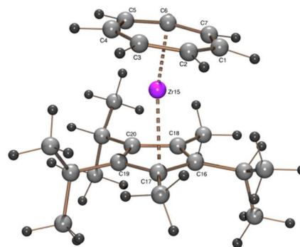
Figure 6. ORTEP plot of the calculated structure of 7 . Calculated bond length (Å) and angles (°): Zr–C1 2.340, Zr–C2 2.349, Zr–C3 2.359, Zr–C4 2.366, Zr–C5 2.358, Zr–C6 2.346, Zr–C7 2.338, Zr–C16 2.518, Zr–C17 2.521, Zr–C18 2.515, Zr–C19 2.517, Zr–C20 2.506, Zr–C pcent 2.202, Zr–CHT cent 1.683, CHT cent –Zr–C pcent 172.05.
