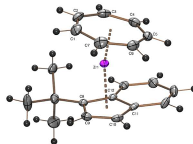
Figure 9. ORTEP plot of the molecular structure of 10 . Atomic displacement parameters have been drawn at 50 % probability. Selected bond length (Å) and angles (°): Zr–C1 2.345(2), Zr–C2 2.354(2), Zr–C3 2.349(2), Zr–C4 2.319(2), Zr–C5 2.312(2), Zr–C6 2.319(2), Zr–C7 2.334(2), Zr–C8 2.507(2), Zr–C9 2.492(2), Zr–C10 2.494, Zr–C11 2.5335(19), Zr–C12 2.544(2), Zr–Cp cent 2.202, Zr–CHT cent 1.661, CHT cent –Zr–Cp cent 167.55.
