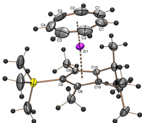
Figure 5. ORTEP plot of the molecular structure of 6 . Atomic displacement parameters have been drawn at 50 % probability. Selected bond length (Å) and angles (°): Zr–C1 2.356(3), Zr–C2 2.345(3), Zr–C3 2.322(3), Zr–C4 2.308(4), Zr–C8 2.488(3), Zr–C9 2.502(2), Zr–C10 2.5121(19), Zr–C pcent 2.187, Zr–CHT cent 1.673, CHT cent –Zr–C pcent 176.75.
