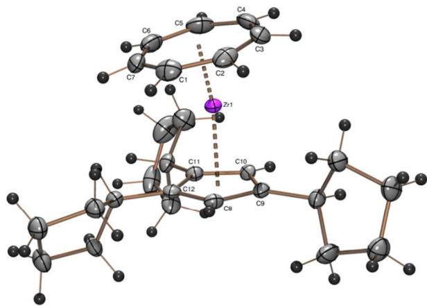
Figure 1. ORTEP plot of the molecular structure of 2 . Atomic displacement parameters have been drawn at 50 % probability. Selected bond length (Å) and angles (°): Zr–C1 2.327(3), Zr–C2 2.339(3), Zr–C3 2.363(3), Zr–C4 2.348(3), Zr–C5 2.341(4), Zr–C6 2.327(3), Zr–C7 2.328(4), Zr–C8 2.482(3), Zr–C9 2.515(3), Zr–C10 2.491(3), Zr–C11 2.511(2), Zr–C12 2.496(3), Zr–Cp cent 2.191, Zr–CHT cent 1.673, CHT cent –Zr–Cp cent 172.03.
