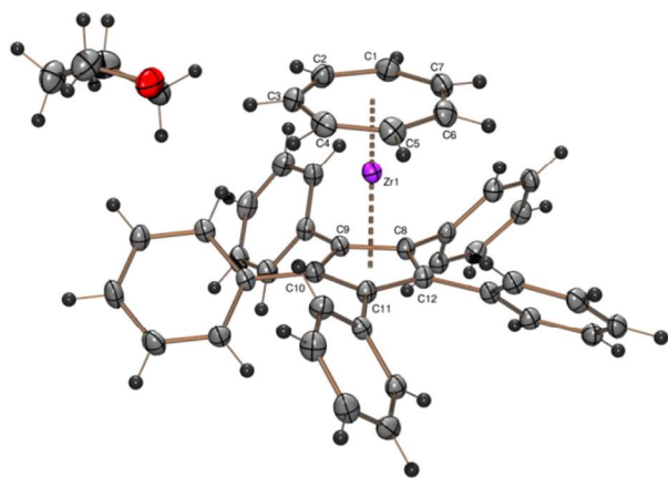
Figure 7. ORTEP plot of the molecular structure of 8 . Atomic displacement parameters have been drawn at 50 % probability. Selected bond length (Å) and angles (°): Zr–C1 2.339(2), Zr–C2 2.333(2), Zr–C3 2.338(2), Zr–C4 2.342(2), Zr–C5 2.335(2), Zr–C6 2.334(2), Zr–C7 2.339(2), Zr–C8 2.534(2), Zr–C9 2.536(2), Zr–C10 2.526(2), Zr–C11 2.528(2), Zr–C12 2.536(2), Zr–Cp cent 2.220, Zr–CHT cent 1.666, CHT cent –Zr–Cp cent 178.9.
