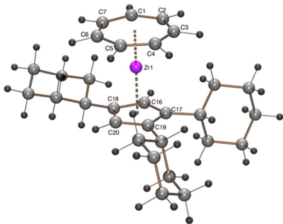
Figure 2. ORTEP plot of the calculated structure of 3 . Calculated bond length (Å) and angles (°): Zr–C1 2.352, Zr–C2 2.353, Zr–C3 2.349, Zr–C4 2.347, Zr–C5 2.353, Zr–C6 2.351, Zr–C7 2.353, Zr–C16 2.511, Zr–C17 2.535, Zr–C18 2.523, Zr–C19 2.529, Zr–C20 2.508, Zr–Cp cent 2.213, Zr–CHT cent 1.684, CHT cent –Zr–Cp cent 178.06.
