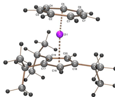
Figure 3. ORTEP plot of the calculated structure of 4 . Calculated bond length (Å) and angles (°): Zr–C1 2.349, Zr–C2 2.360, Zr–C3 2.356, Zr–C4 2.346, Zr–C5 2.344, Zr–C6 2.339, Zr–C7 2.342, Zr–C16 2.508, Zr–C17 2.522, Zr–C18 2.515, Zr–C19 2.524, Zr–C20 2.505, Zr–Cp cent 2.205, Zr–CHT cent 1.679, CHT cent –Zr–Cp cent 174.20.
