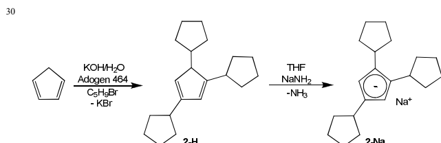
Scheme 1. Synthesis of sodium tri(cyclopentyl)cyclopentadienide NaCp cpent (2-Na).
