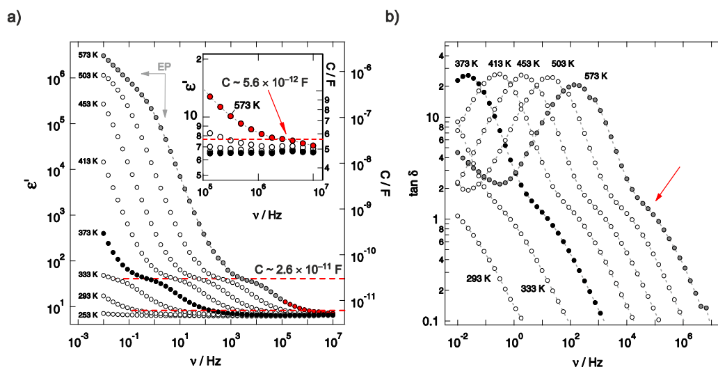
Fig. 5 a) Real part of the permittivity as a function of frequency showing two distinct plateaus with characteristic capacities for bulk conduction processes, see the horizontally drawn dashed lines. This is particularly illustrated in the inset; see the isotherm recorded at 573 K. b) Plot of the dielectric loss, \tan \delta , versus frequency, likewise showing an additional peak as a shoulder in the spectra as indicated by the arrow. EP denotes contributions from electrode polarisation.
