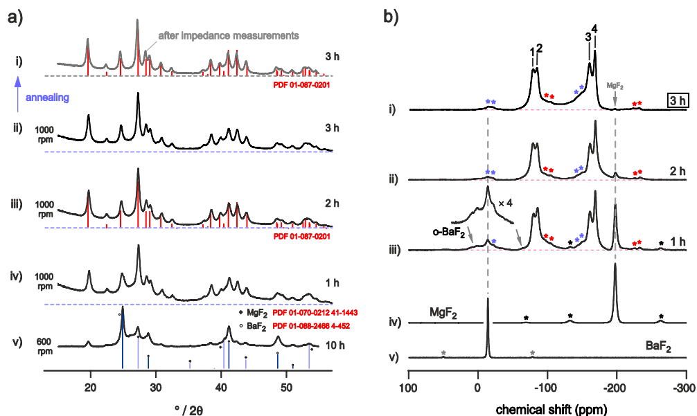
Fig. 2: X-ray powder diffraction patterns of the ball-milled reaction mixture after 1 h, 2 h, and 3 h of milling at 1000 rpm in \text{ZrO}_2 beakers; reflections of a \text{BaMgF}_4 single crystal are indicated by vertically drawn (red) lines. The patterns are stacked with a constant pitch. For comparison, the powder pattern obtained when the milling conditions are changed to 600 rpm and 10 h, that is lower mechanical impact but longer milling time, is also shown, see v). The pattern labelled i) is obtained after impedance measurements. b) ^{19}\text{F} MAS NMR spectra of the reaction mixture at different stages of milling. Spectra were recorded at a spinning speed of 30 kHz. Asterisks indicate the various spinning side bands of the \text{BaMgF}_4 signal as well as those originating from the starting materials. iv) and v) show reference NMR spectra of the non-treated starting materials \text{BaF}_2 and \text{MgF}_2 . Small arrows indicate those NMR lines that can be assigned to orthorhombic \text{BaF}_2 . In iii) the region from 50 ppm to -50 ppm is enlarged to illustrate additional NMR intensities near the ^{19}\text{F} signal of \text{BaF}_2 .
