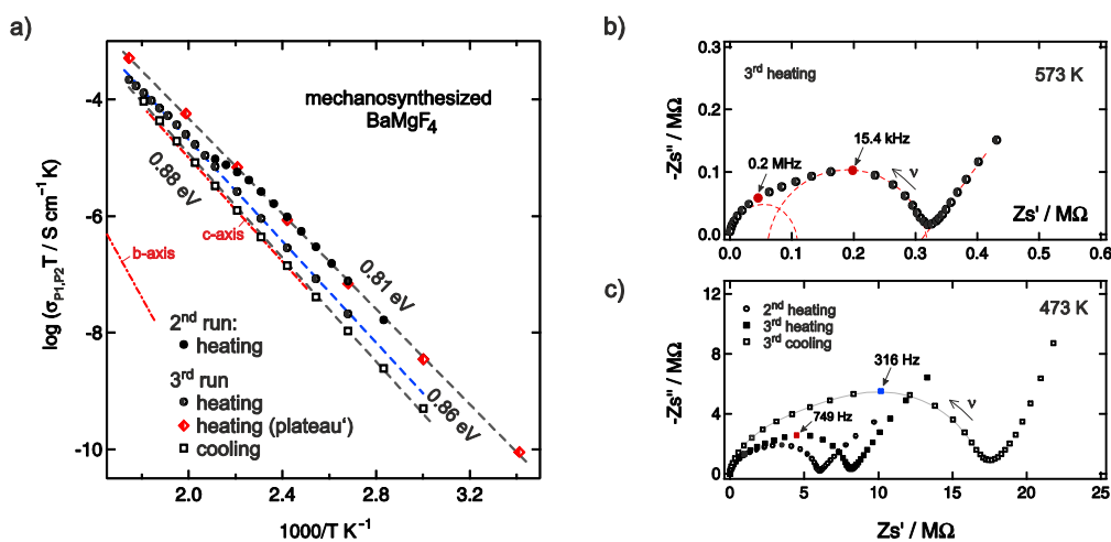
Fig. 4: a) Arrhenius diagram showing the temperature dependence of the dc-conductivity and of the additional plateau value of Fig. 3 b). The dashed lines show Arrhenius fits. For comparison, the dashed-dotted line represents the conductivity of a single crystal along the b-axis; the values for conduction along the c-axis coincide with our data found for the third cooling cycle. b,c) Complex plane plots of the real part vs the imaginary part of the impedance show depressed, overlapping semi-circles for the ball milled, nanocrystalline samples. The coloured symbols (to which the arrows point) represent the frequency at the maximum of the semicircle. b) The red, dashed semicircles schematically represent two different diffusion processes corresponding to the plateaus P1 and P2 in Fig. 3 b). c) The grey, solid line serves as a guide to the eye.
