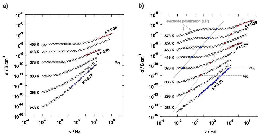
Fig. 3: Conductivity isotherms (real part of complex conductivity vs frequency) recorded of the sample obtained after three hours of milling. a) data obtained from the second heating run up to 473 K and (b), from the third heating run up to 573 K. All the spectra shown reveal characteristic dc-conductivity plateaus at elevated temperatures. Additional plateaus, however, show up at higher frequencies. They are highlighted in (b) by red circles. Conductivities at the highest frequencies can be approximated with power laws. \kappa values indicate the corresponding power law exponents. Arrows in (b) mark polarisation effects due to the ion blocking electrodes applied.
