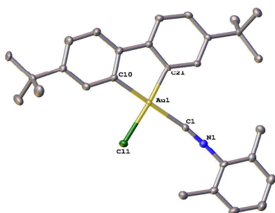
Figure 2. Molecular structure of [\text{Au}(\text{}^t\text{Bu}_2\text{Bip})(\text{XyNC})] ( 5 ). Hydrogen atoms have been omitted for clarity.
