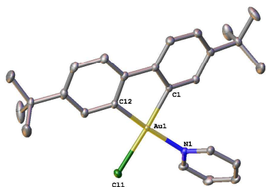
Figure 1. Molecular structure of [\text{Au}(\text{}^t\text{Bu}_2\text{Bip})(\text{Py})] ( 3 ). Only one of the two independent molecules of the asymmetric unit is shown. Hydrogen atoms have been omitted for clarity.
