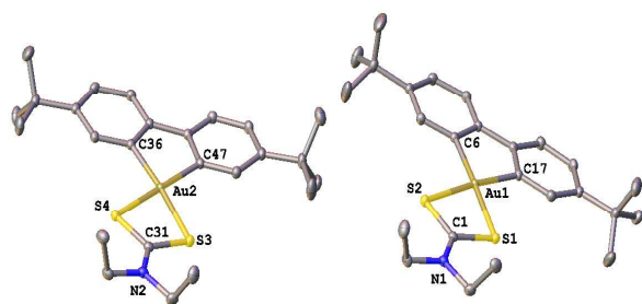
Figure 3. Molecular structure of [\text{Au}(\text{}^t\text{Bu}_2\text{Bip})(\text{S}_2\text{CNET}_2)] ( 8 ). Hydrogen atoms have been omitted for clarity.
