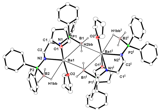
Figure 6. Solid state structure of compound 7 , ellipsoids are drawn to encompass 30 per cent probability, omitting hydrogen atoms (except in the borane groups) for clarity.
