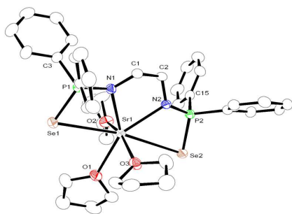
Figure 2. Solid-state structure of compound 3 , ellipsoids is drawn to encompass 30 per cent probability, omitting hydrogen atoms for clarity. Selected bond lengths [ \text{\AA} ] and bond angles[ ^\circ ]:
