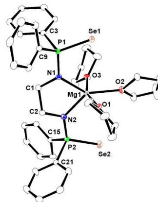
Figure 4. Solid-state structure of compound 5 , ellipsoids is drawn to encompass 30 per cent probability, omitting hydrogen atoms for clarity. Selected bond lengths [Å] and bond angles[°]: P1–N1 1.606(3), P1–Se1 2.1308(10), P1–C3 1.831(3), P1–C9 1.825(3), N1–C1 1.477(4), P2–N2 1.612(3), P2–Se2 2.1240(10), P2–C15 1.833(3), P2–C21 1.834(3), N2–C2 1.482(4), C1–C2 1.524(4), Mg1–N1 2.083(3), Mg1–N2 2.066(3), Mg1–O1 2.124(3), Mg1–O2 2.137(2), Mg1–O3 2.106(2), C2–C1–N1 108.9(3), N1–P1–C9 112.57(15), N1–P1–Se1 110.69(10), N1–P1–C3 111.46(15), P1–N1–C1 121.0(2), Se1–P1–C9 109.18(11), Se1–P1–C3 111.65(11), C1–C2–N2 109.0(3), N2–P2–C15 111.99(15), N2–P2–Se2 111.98(11), N2–P2–C21 110.05(15), P2–N2–C2 118.6(2), Se2–P2–C15 109.14(11), Se2–P2–C21 110.70(11), N1–Mg1–N2 83.40(12), O1–Mg1–O2 80.49(10), O1–Mg1–O3 160.13(11), O2–Mg1–O3 80.11(10), N1–Mg1–O1 94.85(11), N2–Mg1–O1 99.30(11), N1–Mg1–O3 97.76(11), N2–Mg1–O2 134.70(12), N2–Mg1–O1 99.30(11), N2–Mg1–O3 97.36(11).
