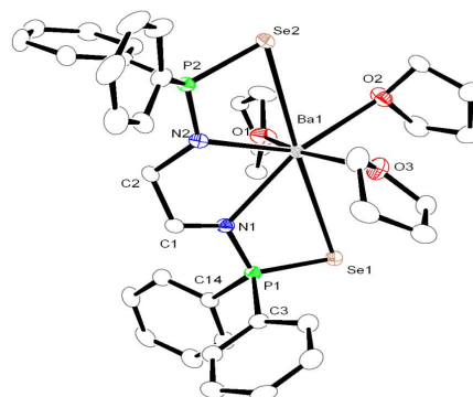
Figure 3. Solid-state structure of compound 4 , ellipsoids is drawn to encompass 30 per cent probability, omitting hydrogen atoms for clarity.
