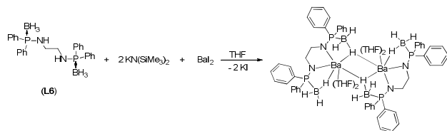
Scheme 4. Synthesis of barium complex 7
