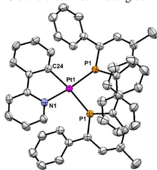
Fig. 2 View of the molecular structure of the cation in the crystal of complex 1 , exhibiting coordination of two phosphinine ligands to the “Pt(ppy)” unit. The H atoms and the triflate anion are omitted for clarity.
