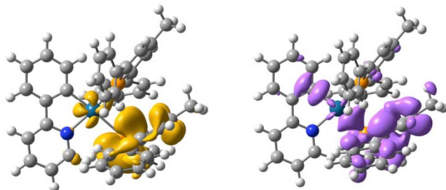
Fig. 4 Density difference plots for the lowest triplet excitation of complex 1 in CH 2 Cl 2 , calculated at the optimised T 1 geometry, using PBE0 and the polarised continuum model for the solvent. Yellow and purple represent zones of depletion and augmentation of electron density in the T 1 excited state versus the S 0 ground state.
