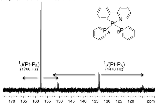
Fig. 1 ^{31}\text{P}\{^1\text{H}\} NMR spectrum of [\text{Pt}(\text{ppy})(\text{L}_p)_2]\text{CF}_3\text{SO}_3 ( 1 ) (the methyl and phenyl substituents as well as the triflate anion are omitted for clarity).
