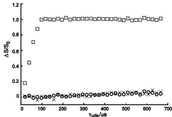
Fig. 10 ^{31}\text{P}\{^1\text{H}\} C-REDOR experiment of \text{Rb}_4\text{P}_4\text{O}_{12} , measured at a spinning frequency of 25 kHz; circles belong to the peak 1 , crosses to peak 2 and squares to peak 3 as shown in Figure 7. 37,38
