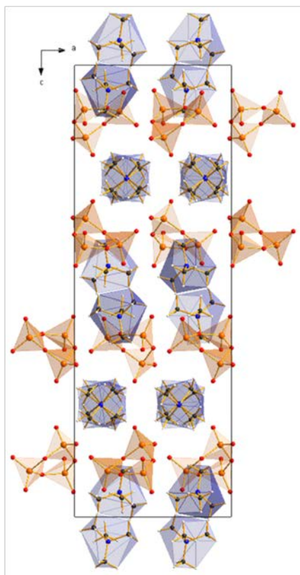
Fig. 6 Crystal structure of (\text{TMA})_2\text{HP}_3\text{O}_9 viewed along [010] . Blue polyhedra: TMA, orange polyhedra: cyclotriphosphate. Orange spheres: phosphorus, red spheres: oxygen, blue spheres: nitrogen, black spheres: carbon, white spheres: hydrogen.
