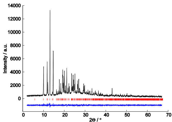
Fig. 1 Observed (black line) powder diffraction pattern of (\text{TMA})_2\text{HP}_3\text{O}_9 ( \text{CuK}\alpha 1 , 154.06 pm) as well as the difference profile (blue line) of the Rietveld refinement. Peak positions are marked by vertical red lines.
