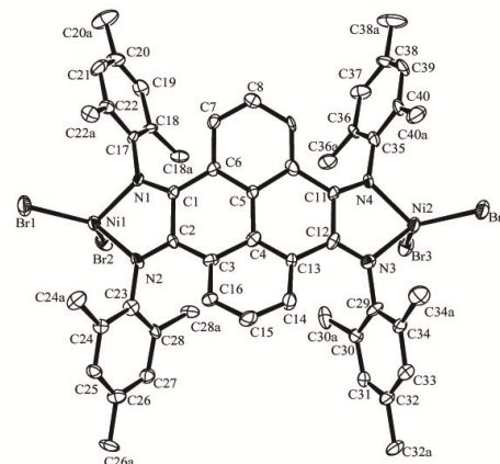
Fig. 2 ORTEP drawing of Ni2 . Thermal ellipsoids are shown at the 30 % probability level. Hydrogen atoms have been omitted for clarity.
