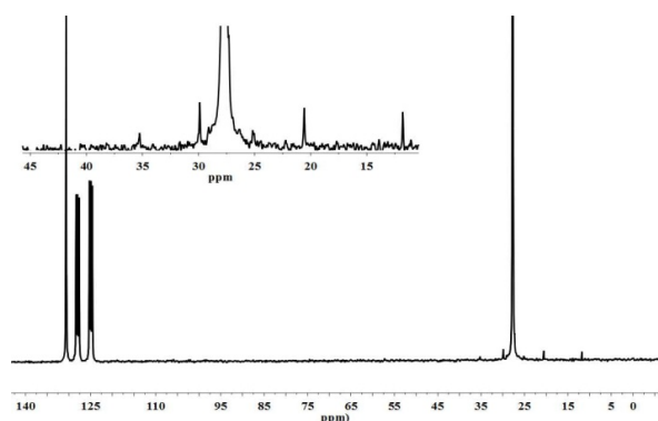
Fig. 7 The 13 C NMR spectra of the polyethylene (entry 1 in Table 3).
