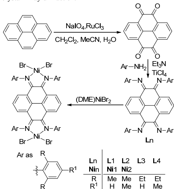
Scheme 2 Synthesis procedures
