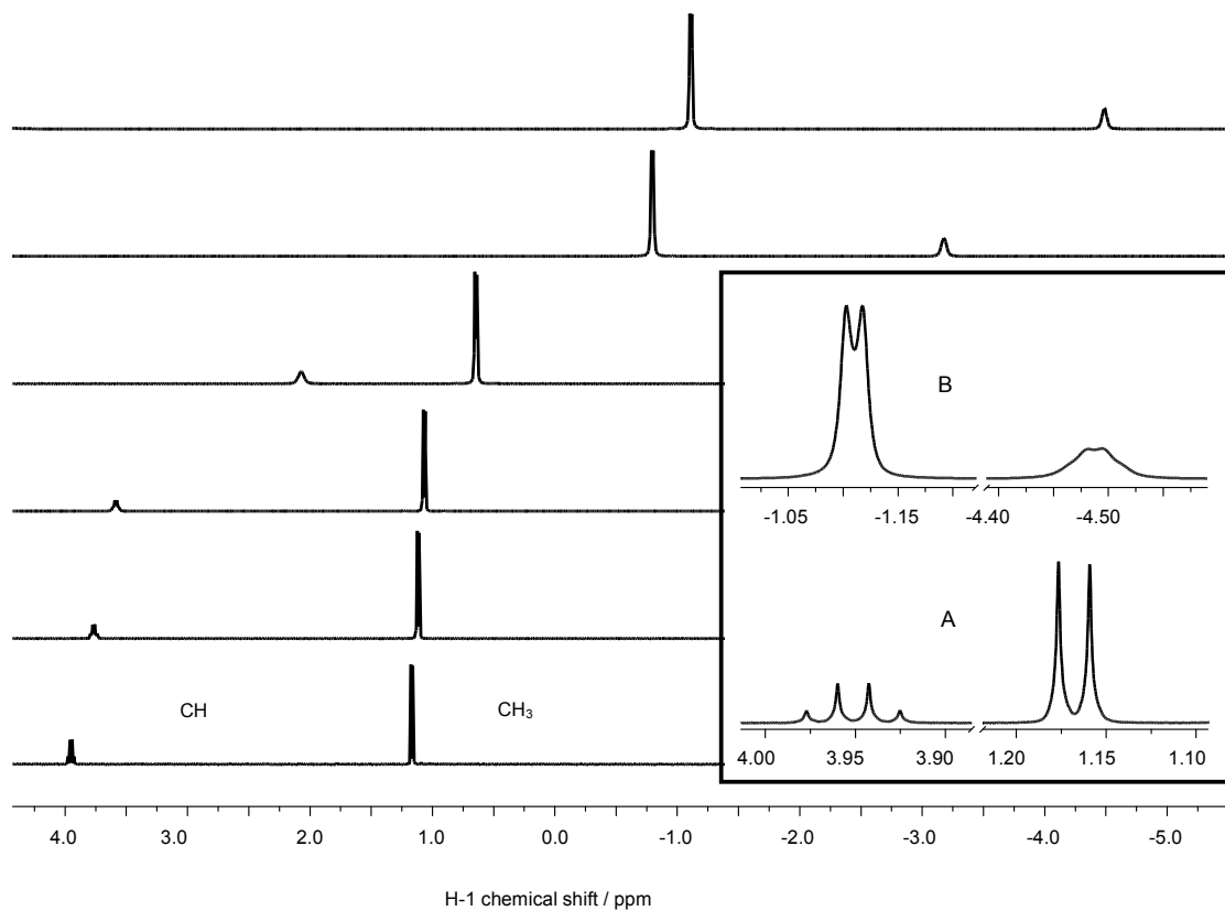
Figure 8. ^1\text{H-NMR} spectra of 0.1 M lactate with varying \text{Eu(III)} concentration (from bottom to top: 0, 1, 5, 10, 50, 100 mM). The inset shows expansions of lactate samples without \text{Eu} (A) and with equimolar concentration of \text{Eu} (B).
