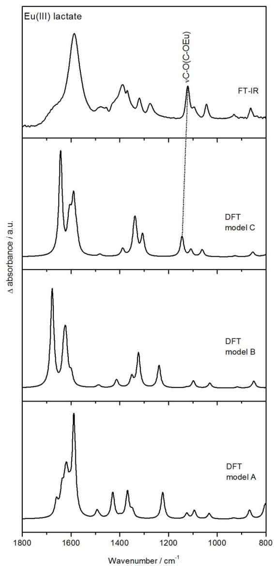
Figure 7. Experimental (ATR FT-IR) and calculated (DFT) spectra of Eu(III) lactate. Calculations were done for structures A, B, and C (from Figure 5). 80x154mm (300 x 300 DPI)
