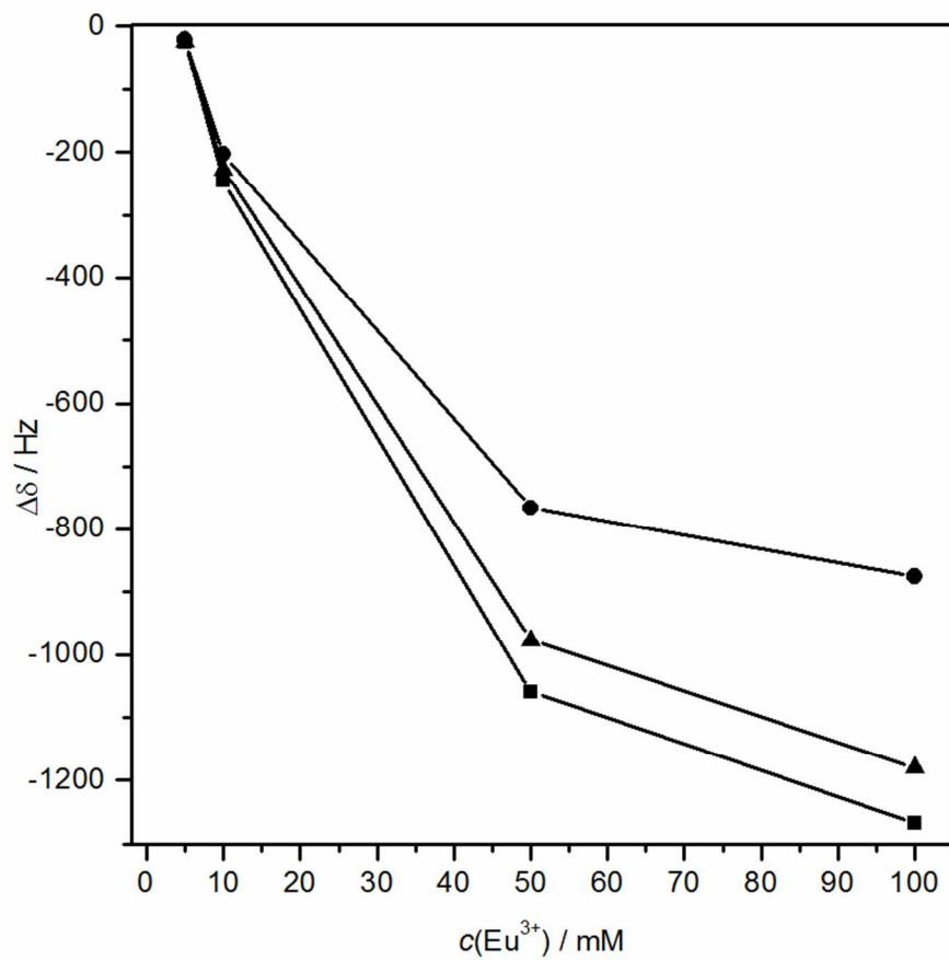
Figure 10. Plot of ^{13}\text{C} chemical shift differences vs. Eu(III) concentration. \blacksquare CH, \blacktriangle COO, \bullet CH 3 , lines drawn for better visualization. 80x74mm (300 x 300 DPI)
