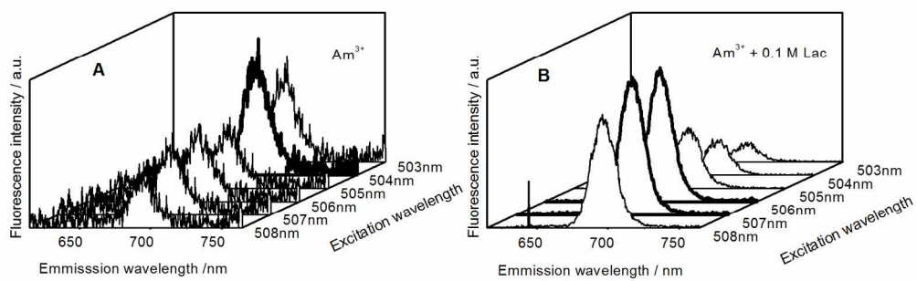
Figure 2. Emission spectra of (A) 5 \mu\text{M} Am(III) and (B) 5 \mu\text{M} Am(III) + 0.1 M lactate in dependence of the excitation wavelength. 160x54mm (300 x 300 DPI)
