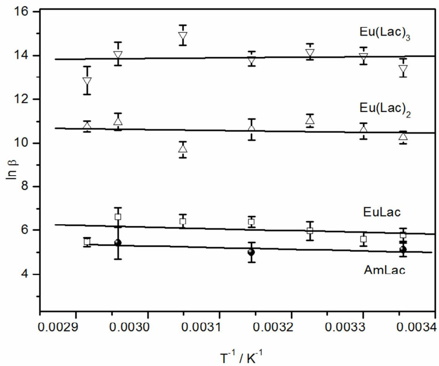
Figure 4. Van't Hoff plots of the Am(III) lactate and Eu(III) lactate complex formation. 80x64mm (300 x 300 DPI)
