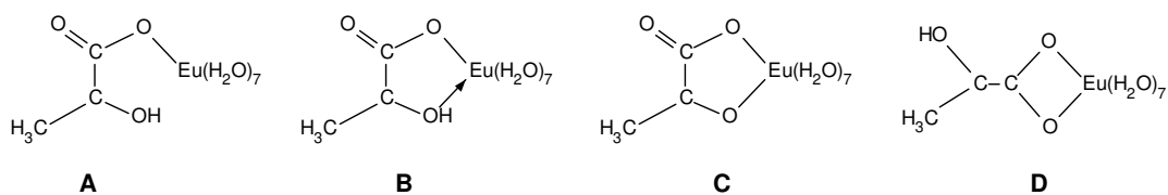
Figure 5. Possible structures of the Eu(III) lactate 1:1 complex: A) monodentate, B) bidentate with coordinating hydroxyl group, C) bidentate with deprotonated hydroxyl group, D) bidentate binding of the carboxylate group.
