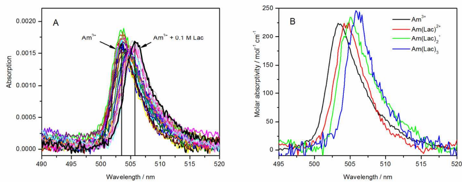
Figure 1. Absorption spectra of 5 μM Am(III) in dependence of the lactate concentration (50 μM to 0.1 M), pH = 6.0, I = 0.1 M, T = 25 °C (left), deconvoluted spectra of the single species (right). 169x70mm (300 x 300 DPI)
