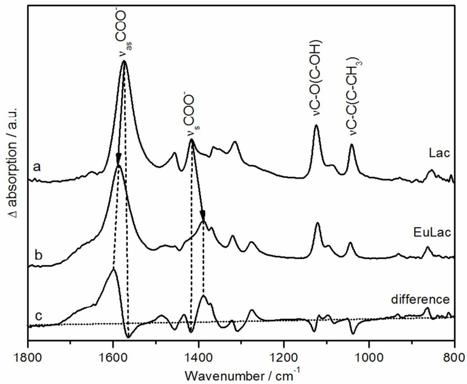
Figure 6. Experimental infrared spectra of lactate at pH 5 (a), Eu(III) lactate at pH 5 (b), and the calculated difference spectrum Eu(III) lactate minus lactate (c). 80x70mm (300 x 300 DPI)
