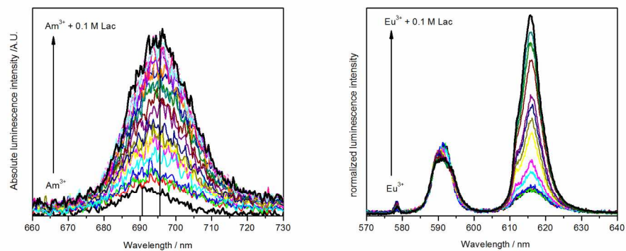
Figure 3. Emission spectra of 5 μM Am(III) (left) and 10 μM Eu(III) (right) in dependence of lactate concentration (10 μM to 0.1 M each, pH = 6.0, I = 0.1 M, T = 25 °C). 169x70mm (300 x 300 DPI)
