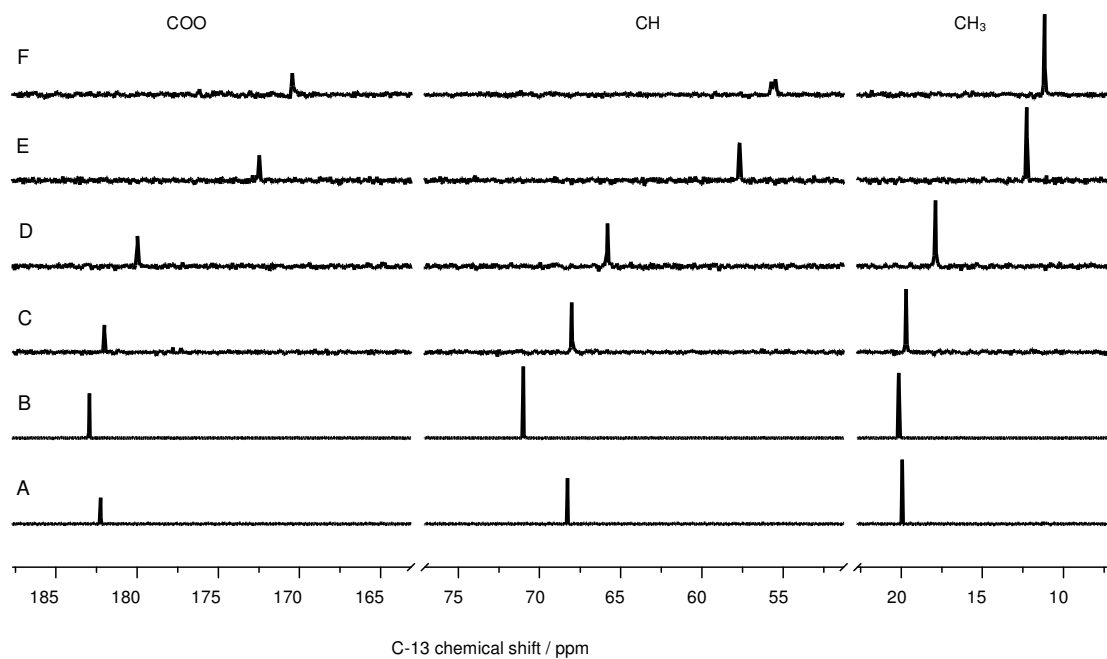
Figure 9. ^{13}\text{C} -NMR spectra of 100 mM lactate, (A) without metal, (B) containing 120 mM \text{La(III)} , and (C) 5, (D) 10, (E) 50, (F) 100 mM \text{Eu(III)} .
