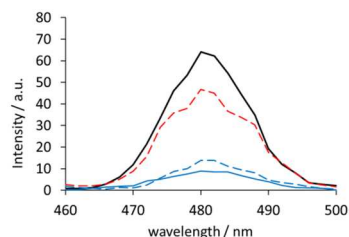
Fig. 5 PTIR 475 UCP emission ( \lambda_{\text{exc}} = 980 nm) in anaerobic solution before (black line) and after (blue line) addition of 100 \mu M PETNR, followed by reduction of the enzyme with 200 \mu M NADPH (red dashed line) and subsequent reoxygenation in air (blue dashed line).
