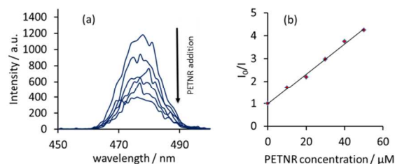
Fig. 4 a) Variation of UCP emission spectra upon incremental addition of PETNR, with only the 475 nm emission band of interest shown; b) Stern-Volmer analysis of the 475 to 800 nm emission intensity ratio as a function of PETNR concentration, where I_0 is the emission intensity before enzyme addition and I is the intensity upon x \mu M PETNR addition.
