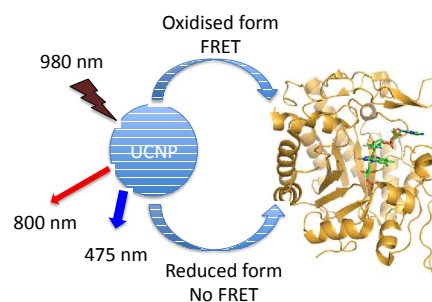
Fig. 1 Schematic illustration of ‘on-off’ FRET process based on UCPs and PETNR. Reduction of the enzyme inhibits FRET and alters the intensity of the 475 nm band in the UCP emission spectrum.
