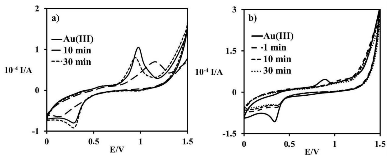
Figure 8. Cyclic voltammograms recorded during the first 30 min of the reaction between 1 mM [\text{AuCl}_4]^- and a) 1 mM pyridine; b) 20 mM pyridine, in 0.4 M NaCl aqueous solution; GCE; E = 0.1 \text{ V s}^{-1} .
