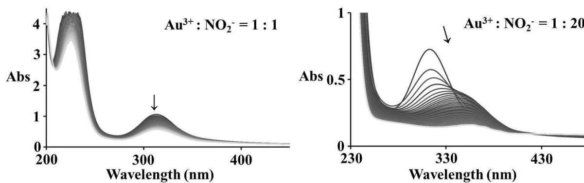
Figure 6. Spectral changes observed during the reaction of 2 \times 10^{-4} M [\text{AuCl}_4]^- and different concentrations of \text{NO}_2^- in 0.4 M NaCl aqueous solution; the arrows show the reaction progress during 2 h (left) and 1 h (right).
