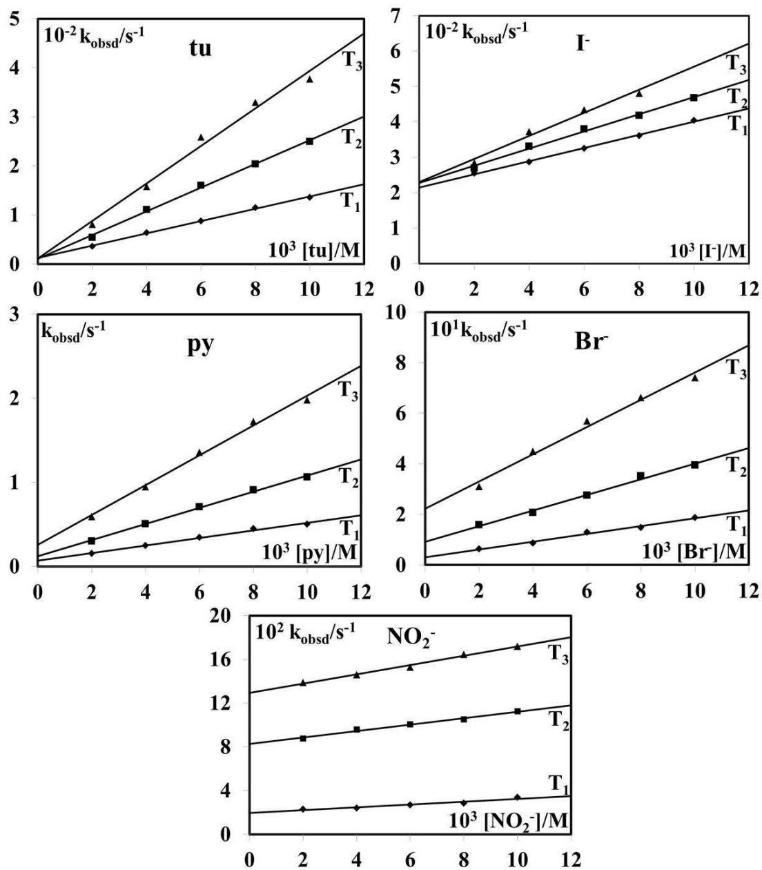
Figure 12. Pseudo-first-order rate constants as a function of nucleophile concentration, for the reaction of [\text{AuCl}_4]^- with thiourea, iodide, bromide, pyridine and nitrite in 0.4 M NaCl aqueous solution, at three different temperatures: T_1 (288 K), T_2 (298 K), T_3 (310 K).
