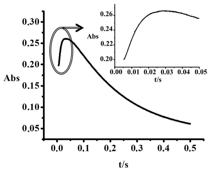
Figure 11. Kinetic trace obtained for the reaction of 1 \times 10^{-4} M [\text{AuCl}_4]^- with a hundred-fold excess of thiourea, T = 287.9 K; \lambda = 300 nm.
