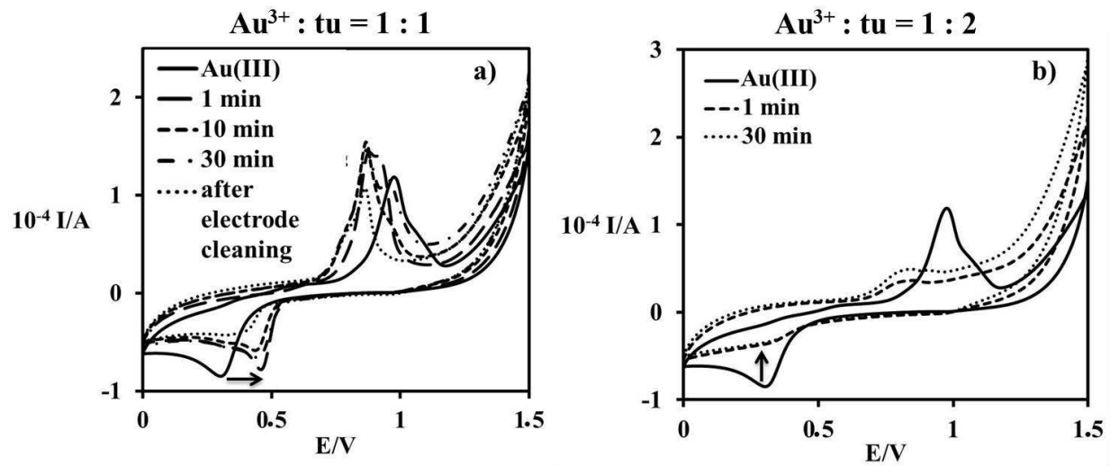
Figure 3. Cyclic voltammograms for the reaction of 1 mM [\text{AuCl}_4]^- and different concentrations of thiourea: a) 1 mM, b) 2 mM; in 0.4 M NaCl; T = 298 \text{ K} ; GCE; E = 0.1 \text{ V s}^{-1} .
