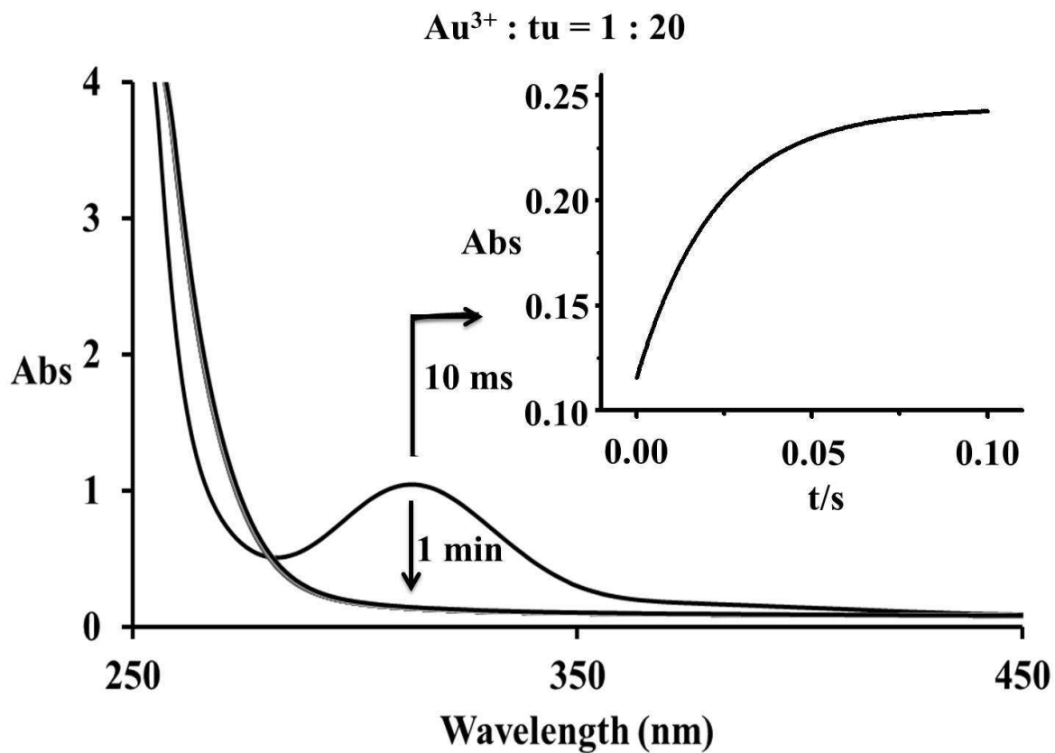
Figure 2. Spectral changes observed for the redox reaction of 1 \times 10^{-4} M [\text{AuCl}_4]^- and 2 \times 10^{-3} M thiourea in 0.4 M NaCl aqueous solution; inset – kinetic trace recorded for the initial substitution step observed on a millisecond time-scale; T = 298.3 K; \lambda = 300 nm.
