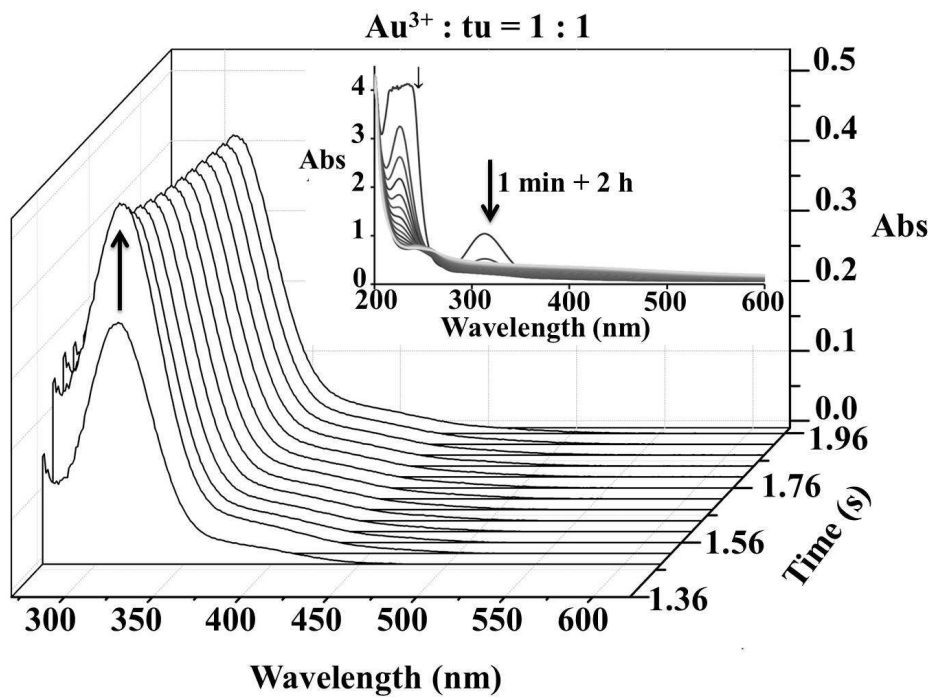
Figure 1. Rapid-scan spectral changes observed during the first 2 s of the reaction between [\text{AuCl}_4]^- and thiourea in 1:1 molar ratio; inset – the same reaction progress followed on a longer time scale.
