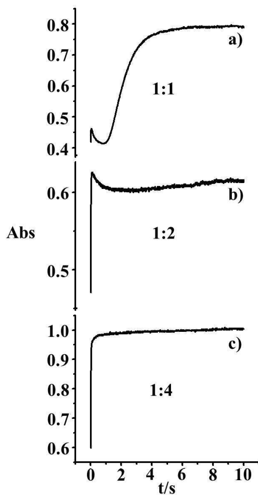
Figure 13. Kinetic traces recorded for the reaction of 1 \times 10^{-4} M [\text{AuCl}_4]^- with different concentrations of \text{I}^- : a) 1 \times 10^{-4} , b) 2 \times 10^{-4} , c) 4 \times 10^{-4} M at 298 K.
