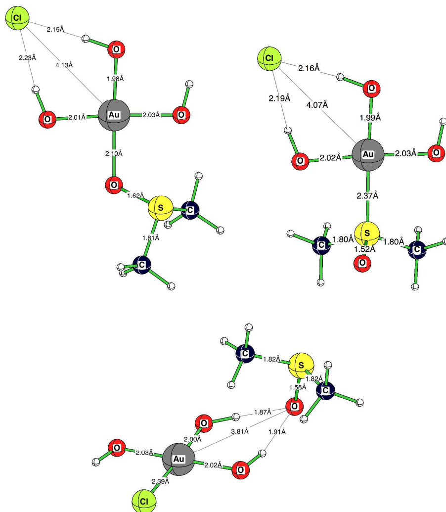
Figure 10. Ab-initio calculated (RMP2(full)(CPCM)/LANL2DZp) structures of the three possible aggregates formed between DMSO and [AuCl(OH) 3 ] - .
