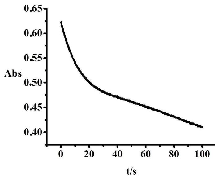
Figure 14. Typical reaction trace obtained for the reaction of 1 \times 10^{-4} M [\text{AuCl}_4]^- with the forty-fold excess of \text{NO}_2^- , T = 298.6 K; \lambda = 310 nm.
