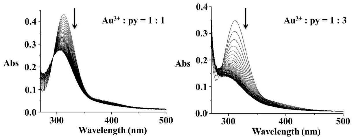
Figure 7. Rapid-scan spectral changes recorded for the reaction between [\text{AuCl}_4]^- and pyridine in different molar ratios over 50 s; left - observed substitution reaction, right - substitution followed by redox reaction.
