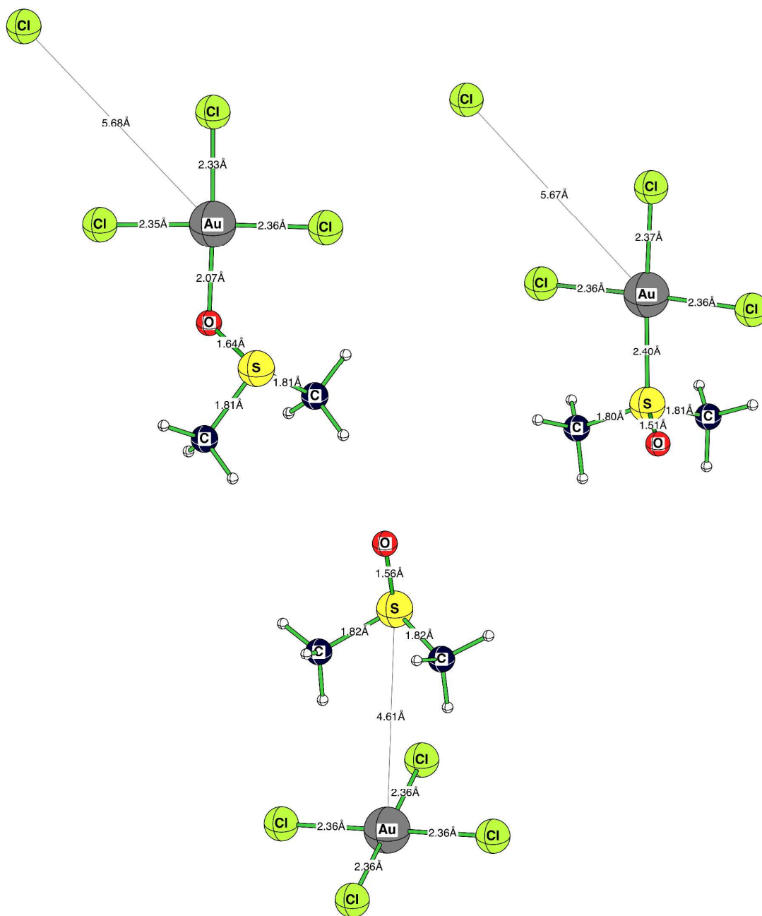
Figure 9. Ab-initio calculated (RMP2(full)(CPCM)/LANL2DZp) structures of the three possible aggregates formed between DMSO and [\text{AuCl}_4]^- .
