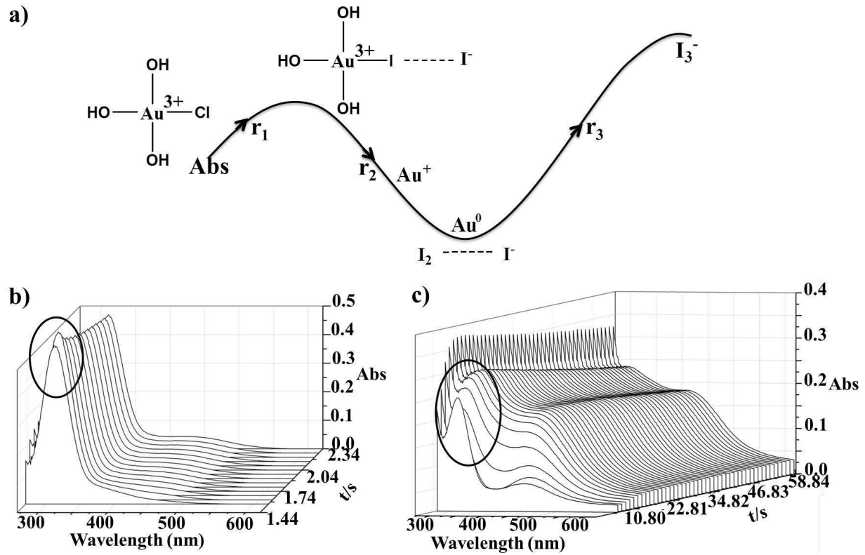
Figure 4. Spectral changes recorded after rapid mixing of 1 \times 10^{-4} M [\text{AuCl}_4]^- and an equimolar concentration of iodide; a) trend in the absorbance changes upon formation of different reaction products, \lambda = 285 nm, b) during the first 3 s of the reaction, and c) the next 60 s.
