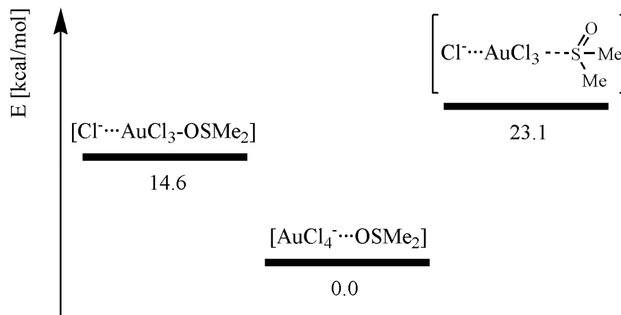
Scheme 3. Energetic differences (RMP2(full)(CPCM)/LANL2DZp) of the three possible aggregates formed between DMSO and [\text{AuCl}_4]^- .
