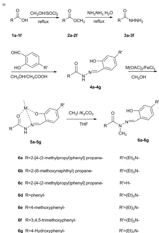
Scheme 2 The synthesis of the N-Methyl-N'-2-hydroxybenzaldehyde acylhydrazones (6a–6g)
