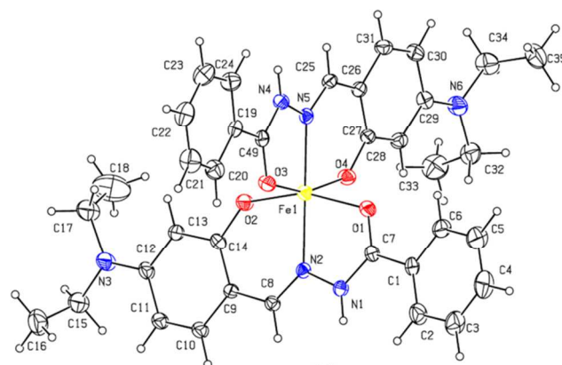
Fig. 1 ORTEP diagram of the Fe(III) complex of N-(4-diethylamino-2-hydroxybenzylidene)-benzohydrazide (5d)
