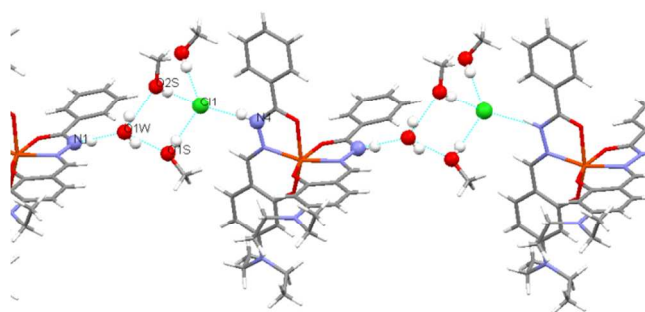
Fig. 3 The H-bond network of the complex 5d .
