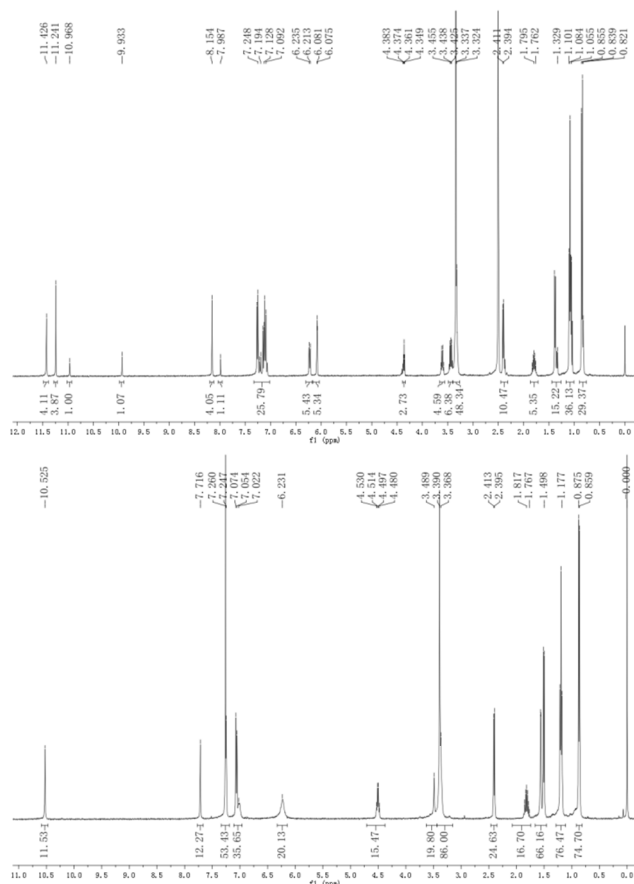
Fig. 2 ^1\text{H} NMR spectra of N-(4-diethylamino-2-hydroxybenzylidene)-2-[4-(2-methylpropyl)phenyl]propane hydrazide ( 4a ) (top) and N-methyl-N'-(4-diethylamino-2-hydroxybenzylidene)-2-[4-(2-methylpropyl)phenyl]propane hydrazide ( 6a ) (bottom).
