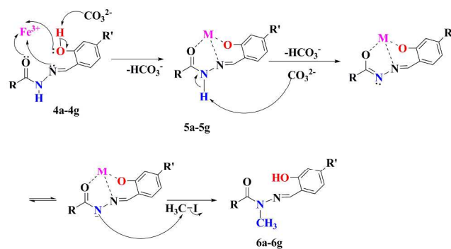
65 Scheme 1 Proposed selective N-methylation of amide bond of N-acylhydrazone by an iron complex.
