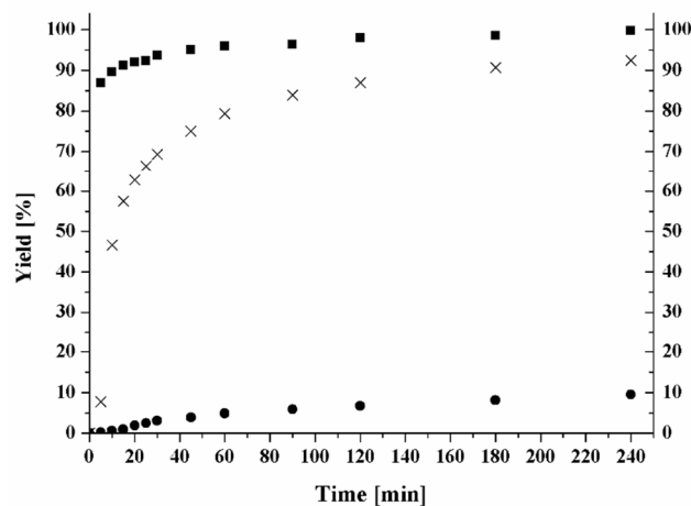
Figure 3 Kinetics of the tricarbonyl complexes 1 [\text{CpMo}(\text{CO})_3\text{Cl}] ( \blacksquare ), 2 [\text{CpMo}(\text{CO})_3\text{CH}_3] ( \times ) and 3 [\text{CpMo}(\text{CO})_3\text{CF}_3] ( \bullet ). Catalyst:cyclooctene:tert-butylhydroperoxide (TBHP); ratio: (0.0025:1:1.2); T = 25 °C.
