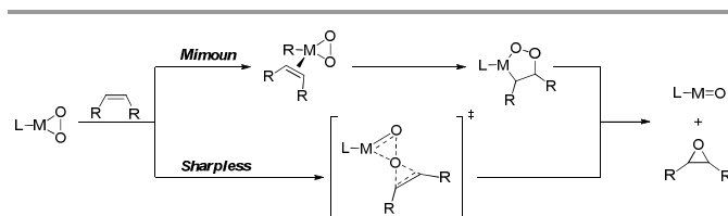
Scheme 1 Two major mechanistic proposals of olefin epoxidation: Mimoun-type and Sharpless-type mechanisms.
