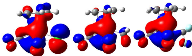
Fig. 4 Comparison of the HOMOs of the compounds [CpMo(CO) 3 R] with R = Cl ( 1 ), CH 3 ( 2 ) and CF 3 ( 3 ) (from left to right) in gas phase (B3LYP/6-31+G**(d,p) level of theory, for details see supp. info. ).
