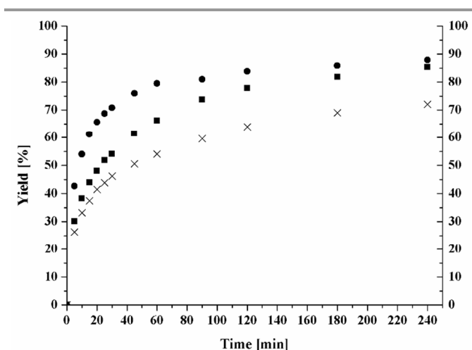
Fig. 6 Kinetics of the oxo-peroxy complexes 4 [CpMo(O 2 )(O)Cl] (■), 5 [CpMo(O 2 )(O)CH 3 ] (X) and 6 [CpMo(O 2 )(O)CF 3 ] (●). Catalyst:cyclooctene:TBHP; ratio: (0.0025:1:1.2); T = 25 °C.
