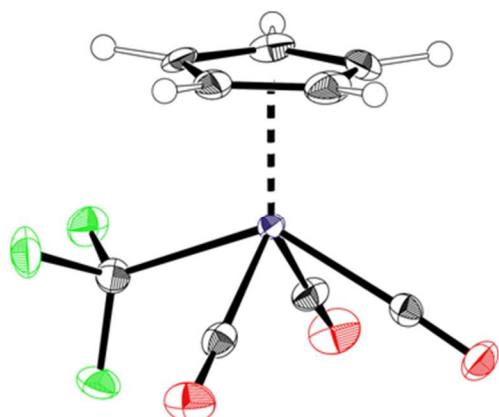
Fig. 1 ORTEP style drawing of the solid-state structure of 3 [\text{CpMo}(\text{CO})_3\text{CF}_3] . The thermal ellipsoids are shown at the 50% probability level.
